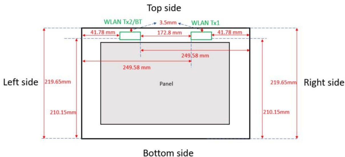
Fig.9 Antenna location of EUT (Tablet mode)
