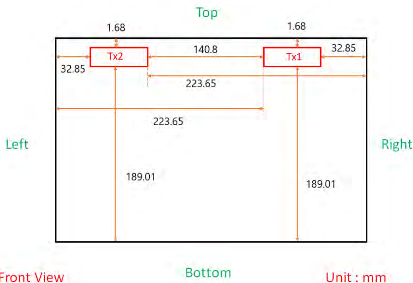
Fig.10 Antenna position of EUT (Tablet mode)
