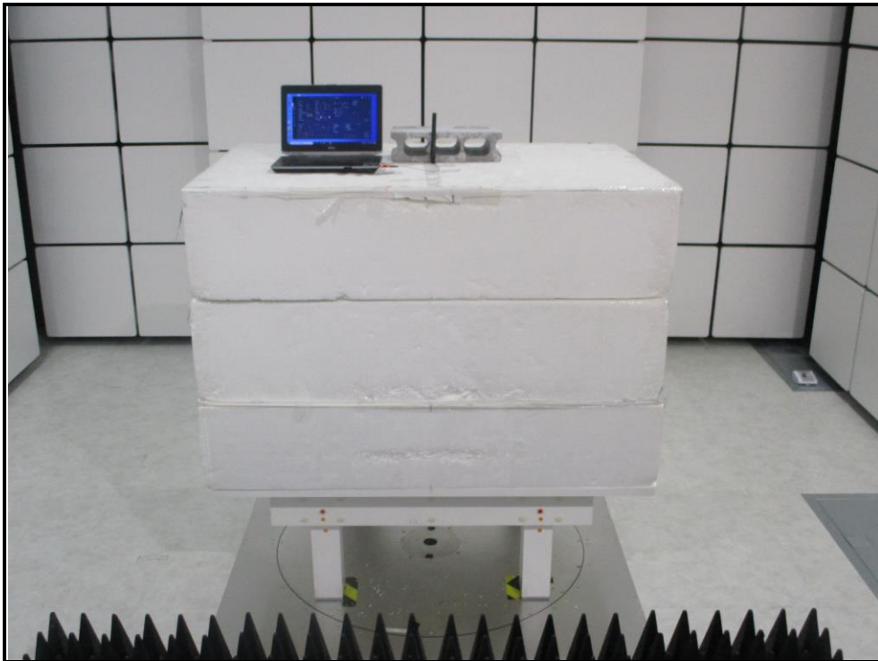
Dipole Antenna 1TX
