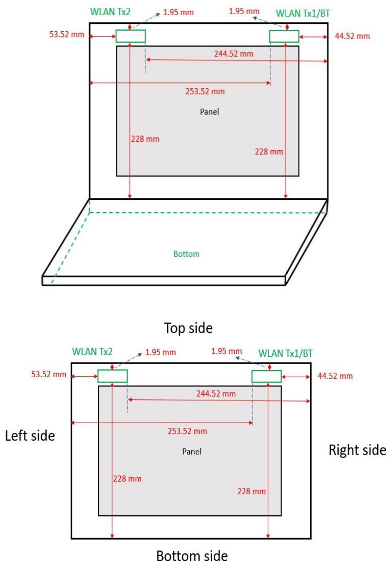
Photograph 17. Antenna position of EUT
