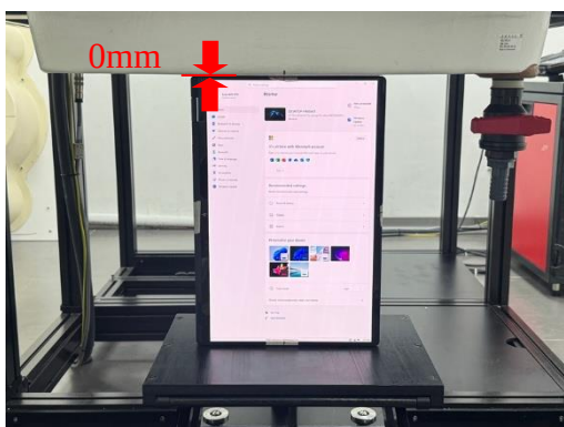
Photograph 5. Body, Left Edge, 0mm
