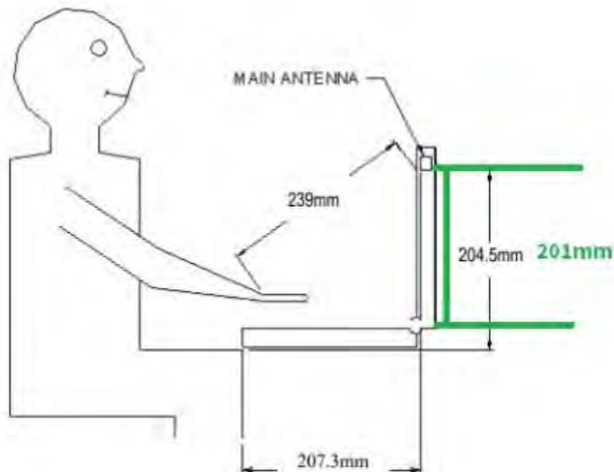
Antenna location (laptop mode)
