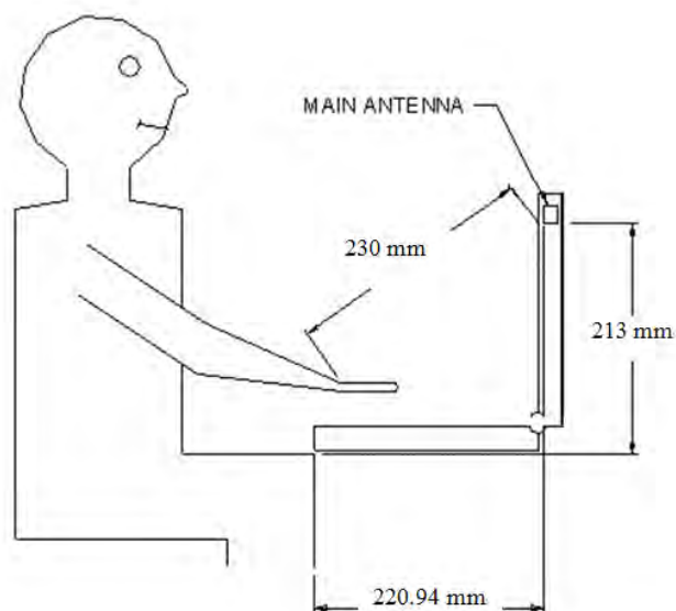
Fig.10 Antenna location of EUT (laptop mode)
