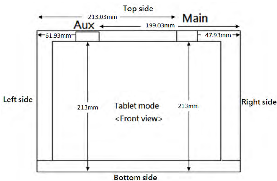
Fig.9 Antenna location of EUT (tablet mode)
