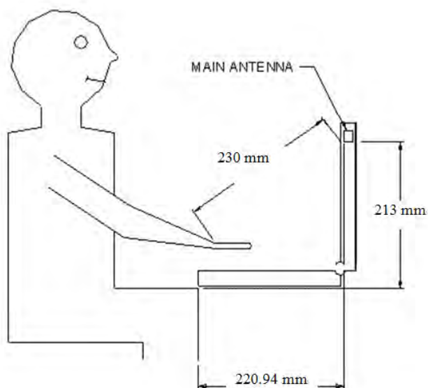
Fig.10 Antenna location of EUT (laptop mode)
