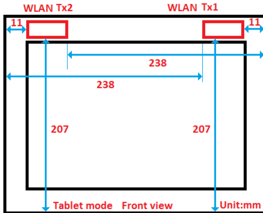
Fig.9 Antenna position of EUT (Tablet mode)
