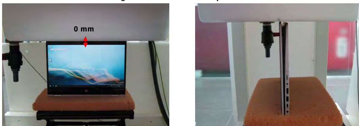
Fig.4 EUT Top side to flat phantom
