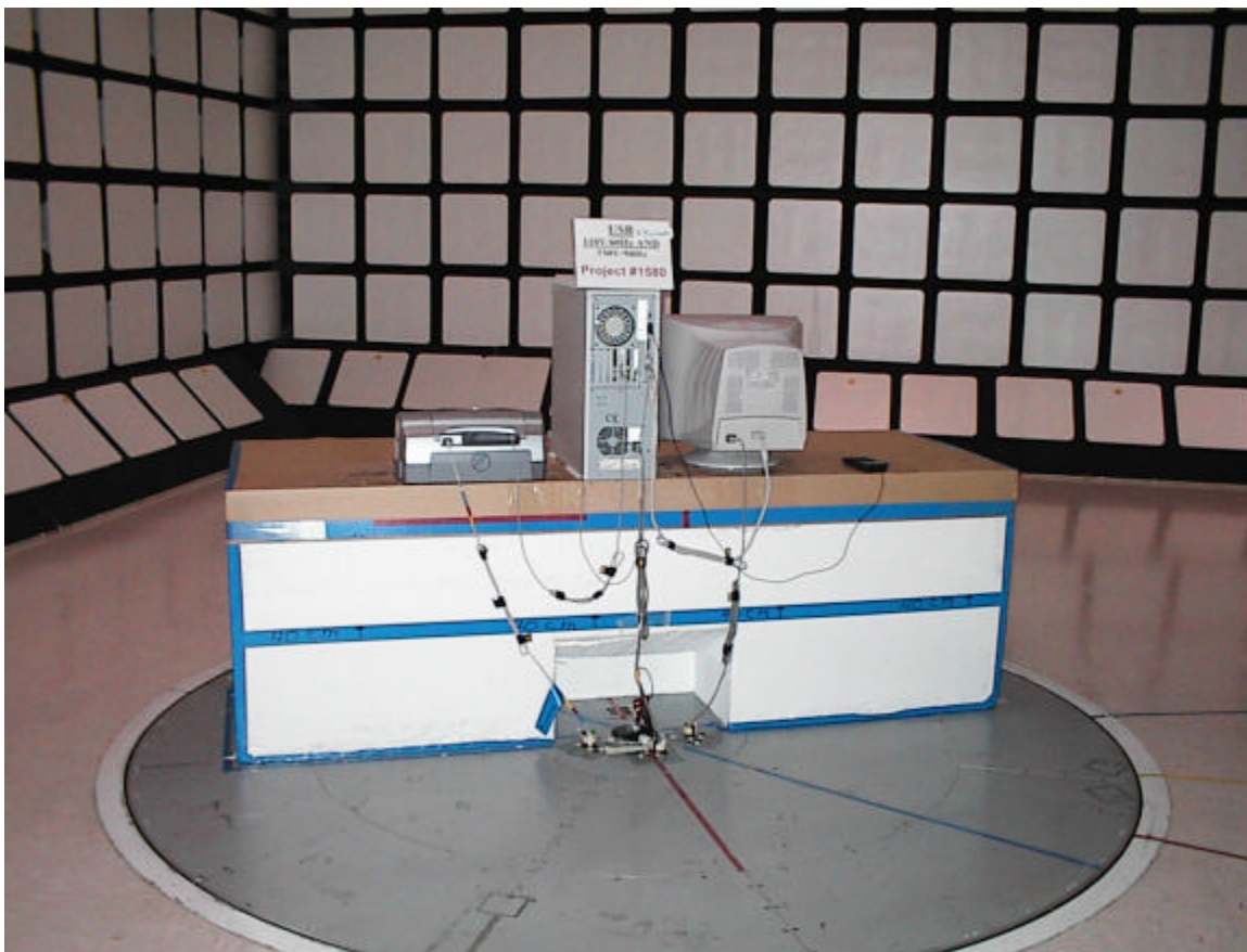
This test setup represents both 110V and 230V operation, with or without the RF link.
