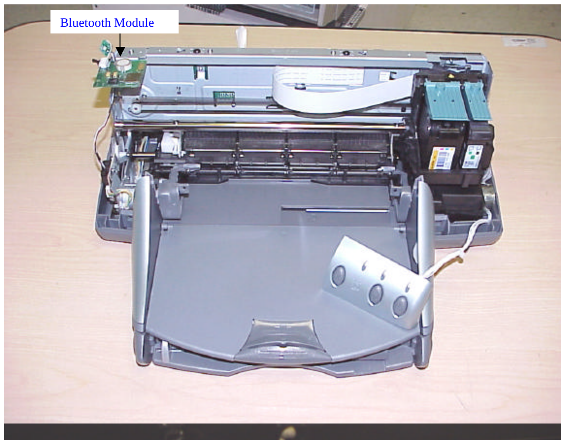
Printer open view with Bluetooth Module
