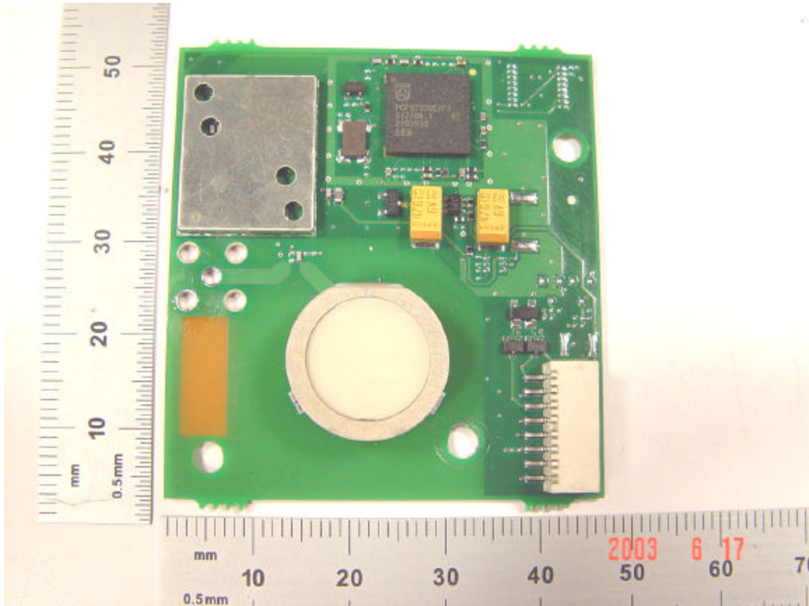
Bluetooth Module Top with shielding
