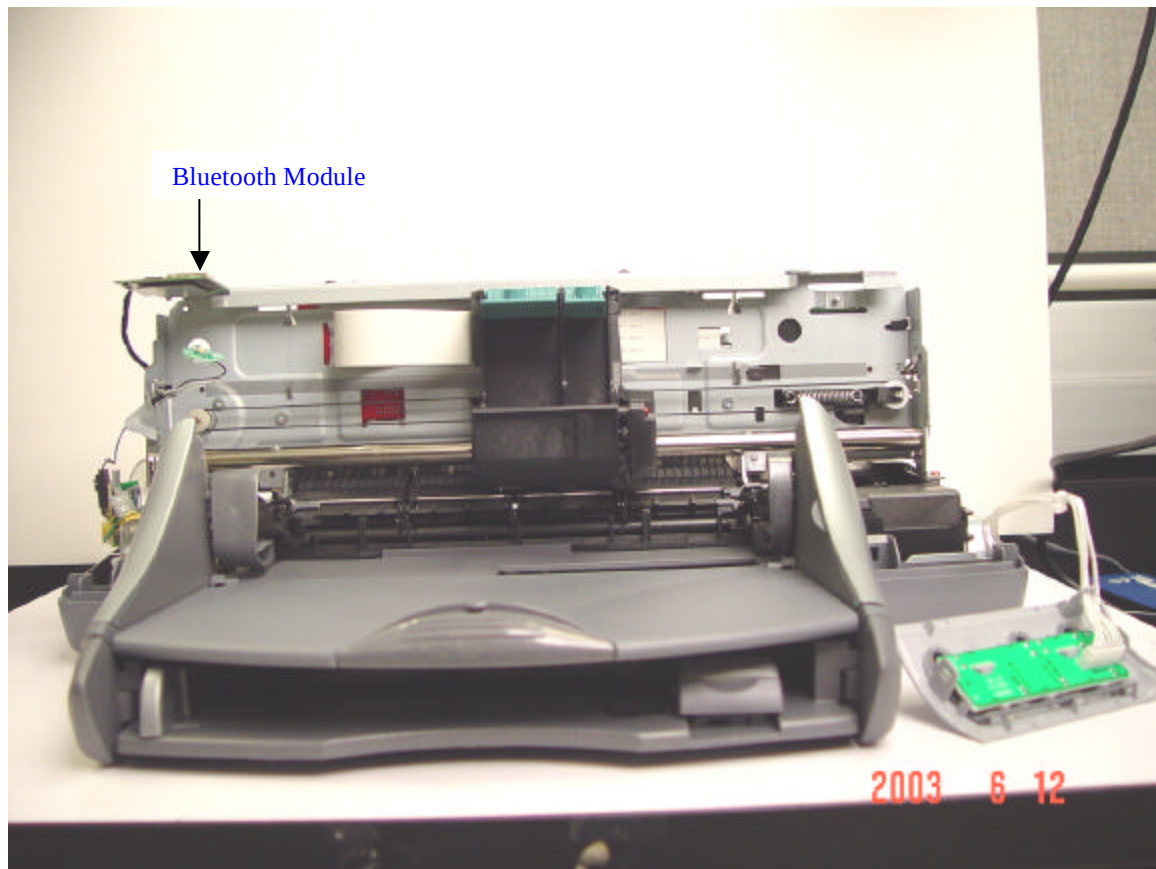
Printer open view with Bluetooth module
