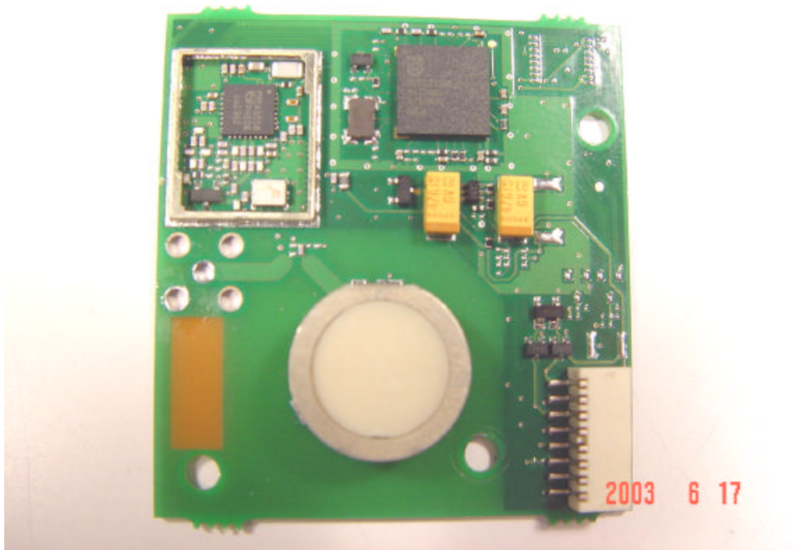
Bluetooth Module Top without shielding
