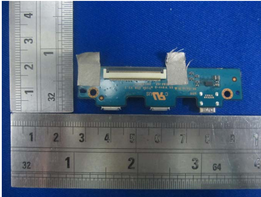
EUT- USB and HDMI Port Board Bottom View
