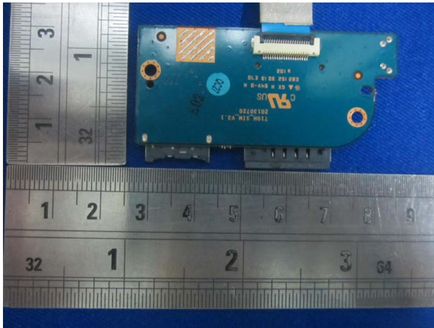
EUT- TF and SIM Card Board Bottom View
