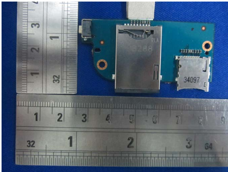
EUT- TF and SIM Card Board Top View
