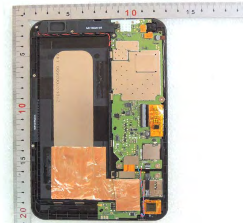
Open View of EUT – 6
