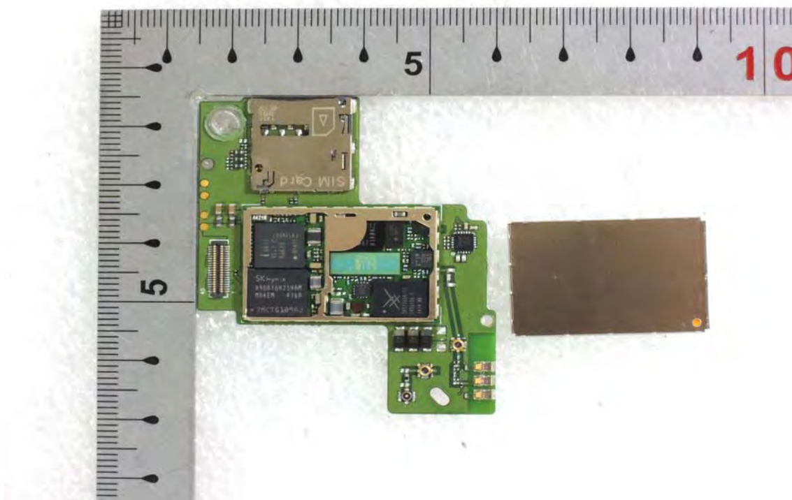
Internal View of EUT – 8
