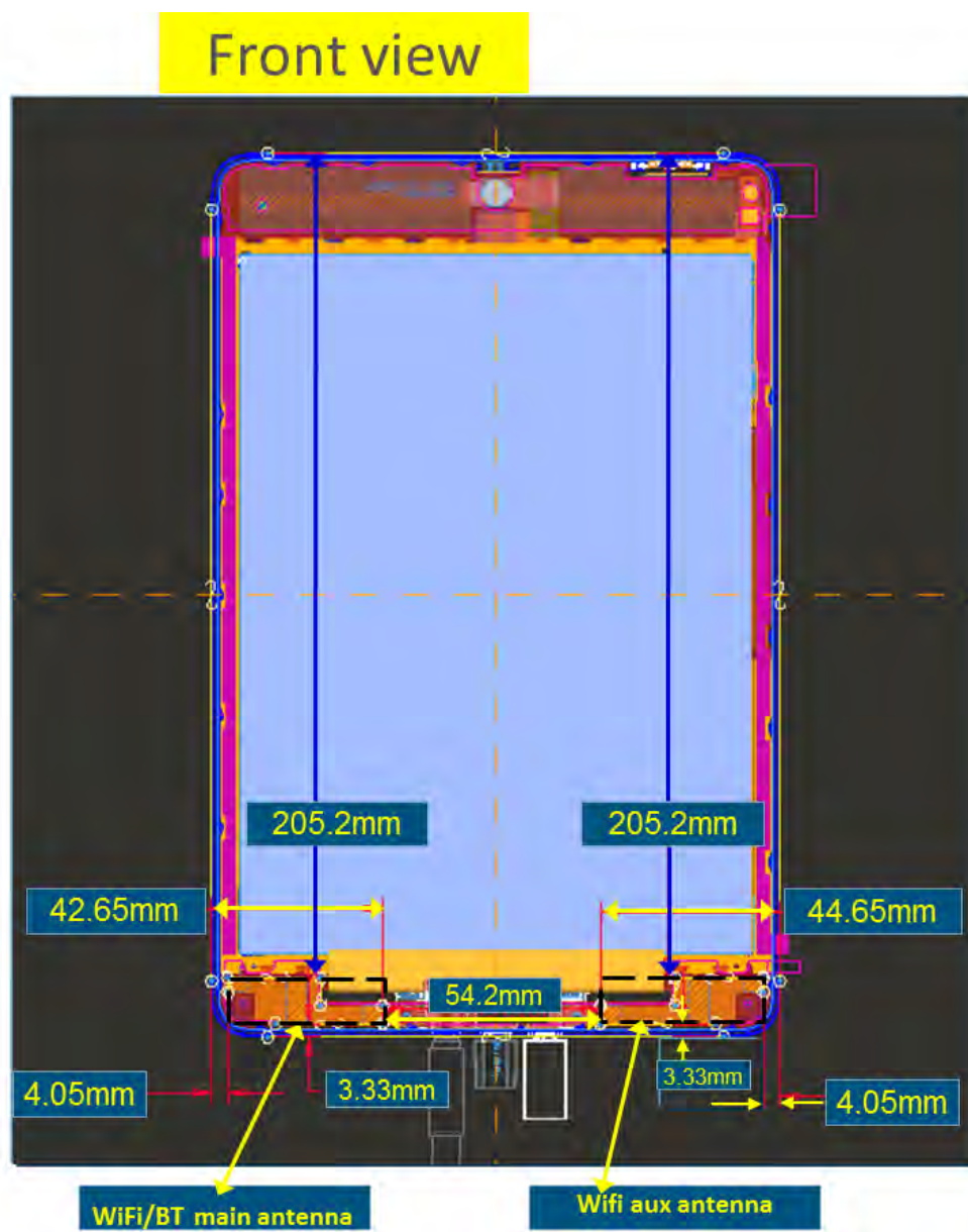
Fig.8 Antenna position of EUT
