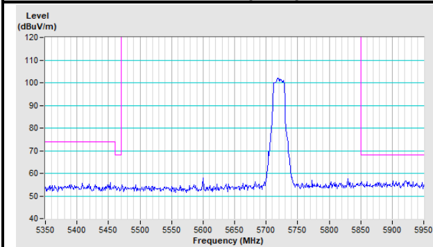
Horizontal (Peak)
