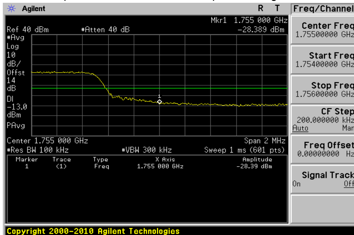
Figure 9-88: Band edge emission at antenna terminals –10MHz BW LTE-Band 4 (QPSK RB Number: 50 Offset: 0) Channel Highest
