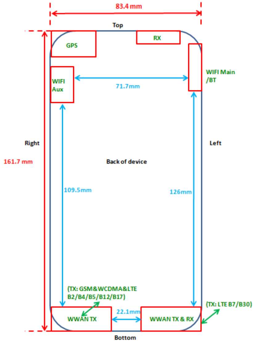
Fig.21 Antenna position of EUT
