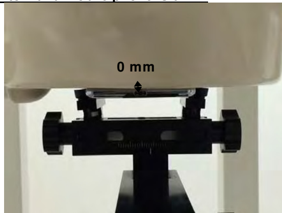
Fig.14 EUT front to flat phantom
