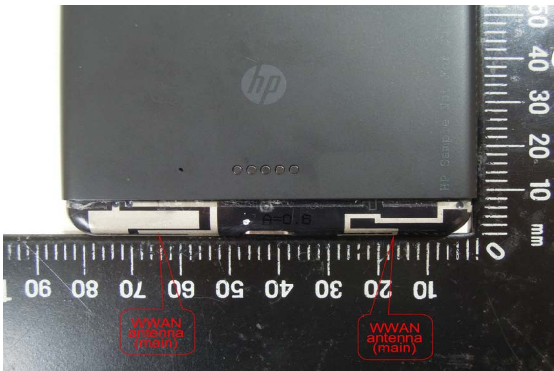
WWAN Antenna (Main)
