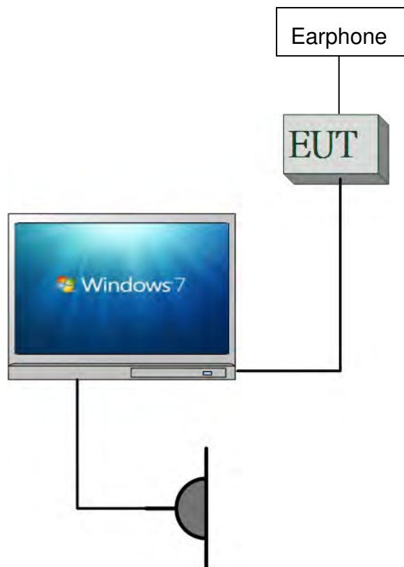
Fig. 2-1 Radiated Emission & Conducted (Antenna Port) Configuration
