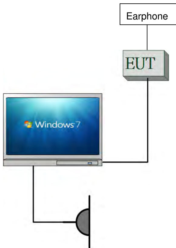
Fig. 2-2 Conducted (Antenna Port) Configuration Emission
