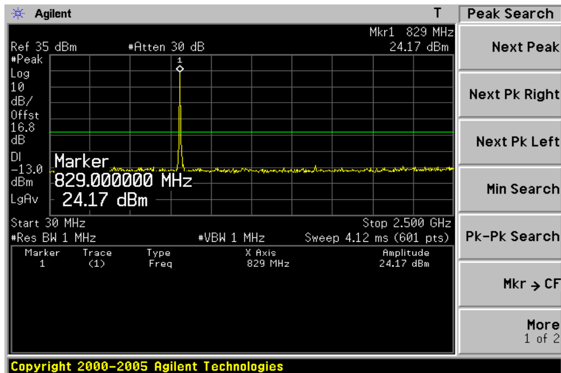
Figure 8-46: Out of Band emission at antenna terminals – HSUPA V Channel Lowest
