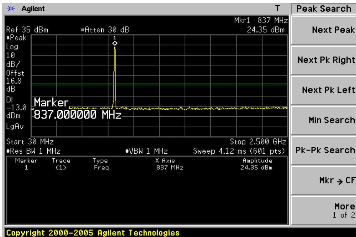
Figure 8-47: Out of Band emission at antenna terminals – HSUPA V Channel Mid
