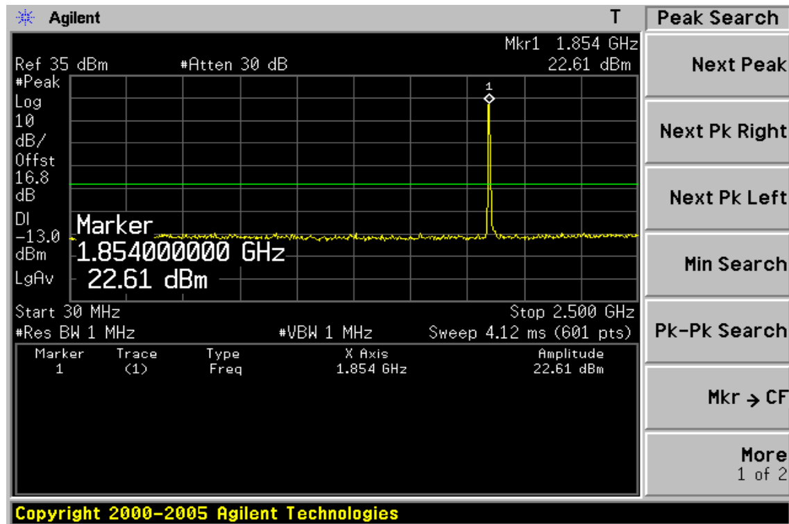
Figure 8-41: Out of Band emission at antenna terminals – HSUPA II Channel Lowest
