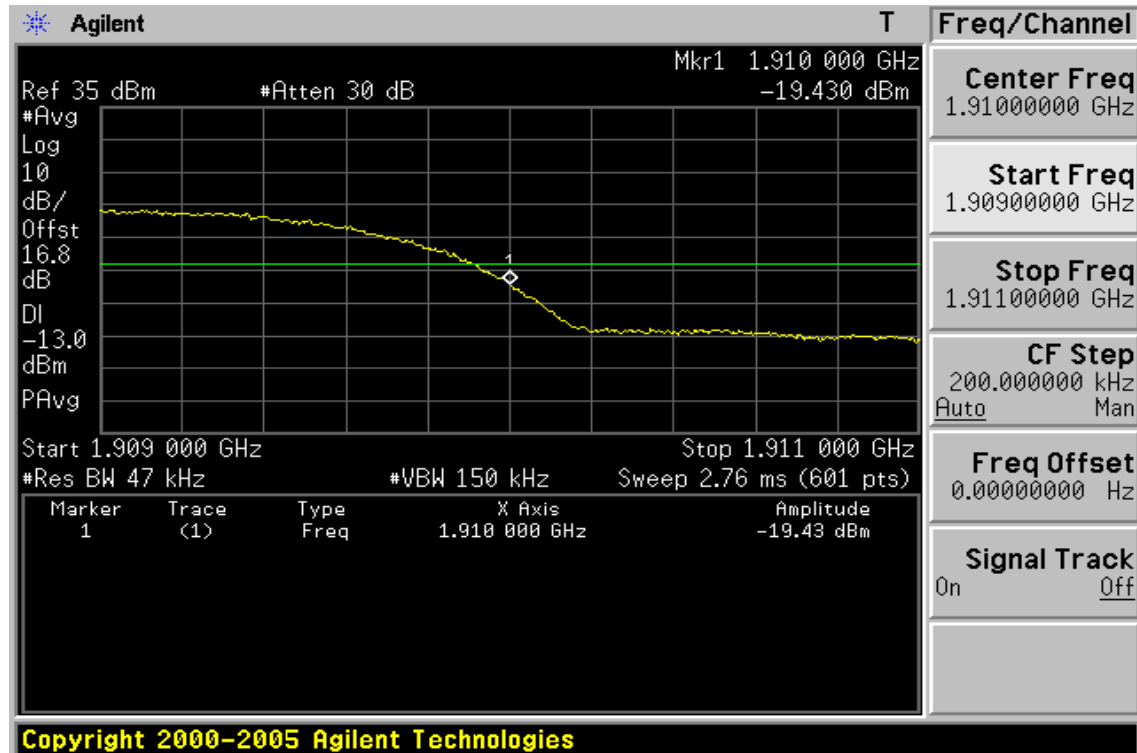
Figure 8-45: Band edge emission at antenna terminals – HSUPA II Channel Highest
