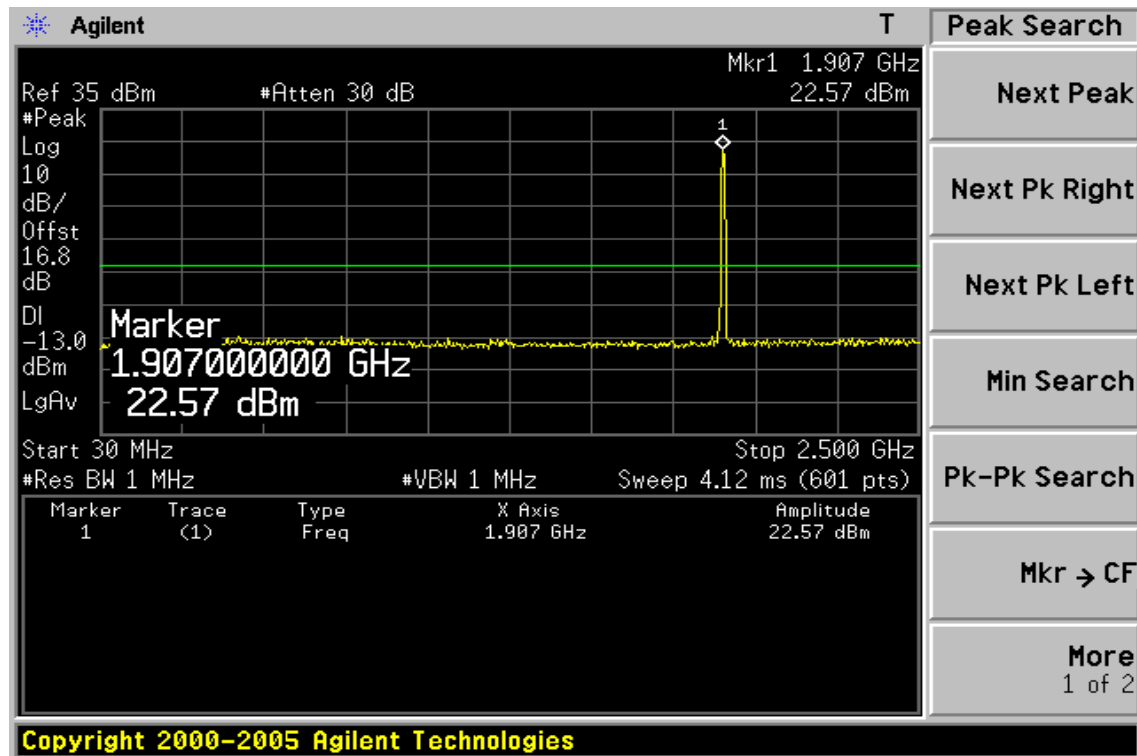
Figure 8-43: Out of Band emission at antenna terminals – HSUPA II Channel Highest
