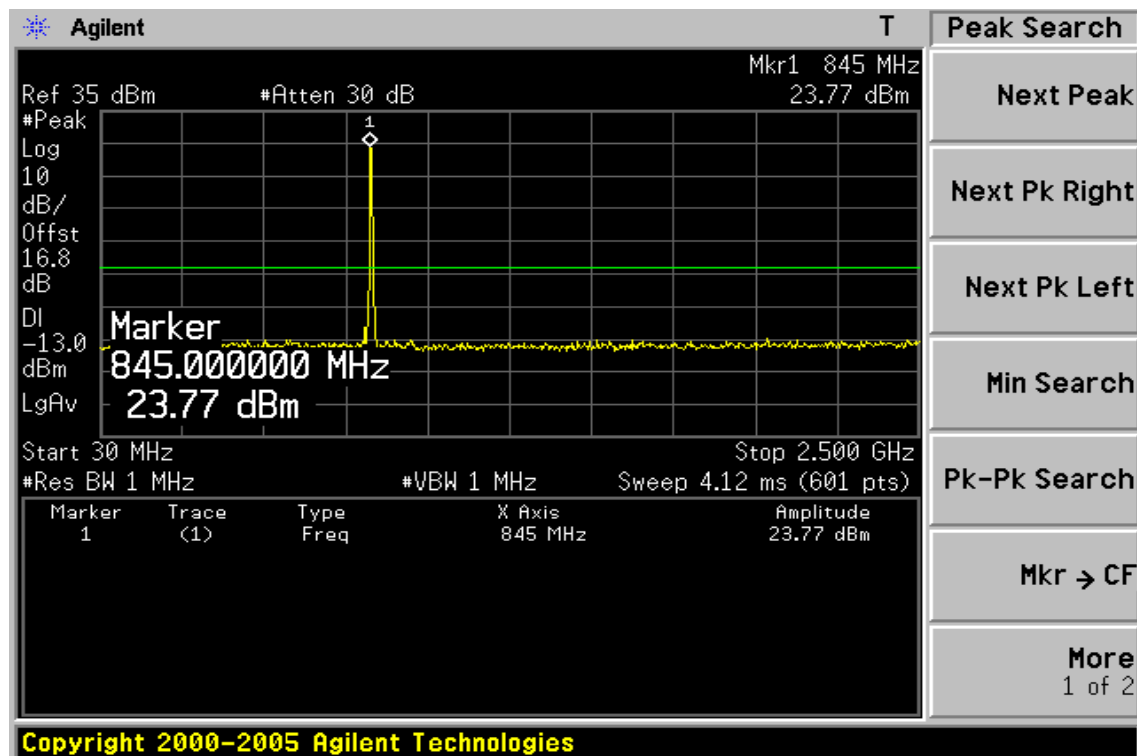
Figure 8-48: Out of Band emission at antenna terminals – HSUPA V Channel Highest
