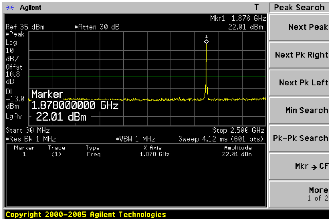
Figure 8-42: Out of Band emission at antenna terminals – HSUPA II Channel Mid
