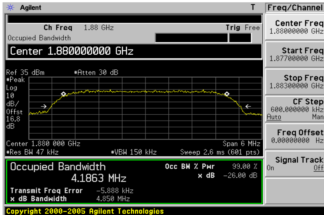
Figure 7-26 HSUPA II Channel Mid
