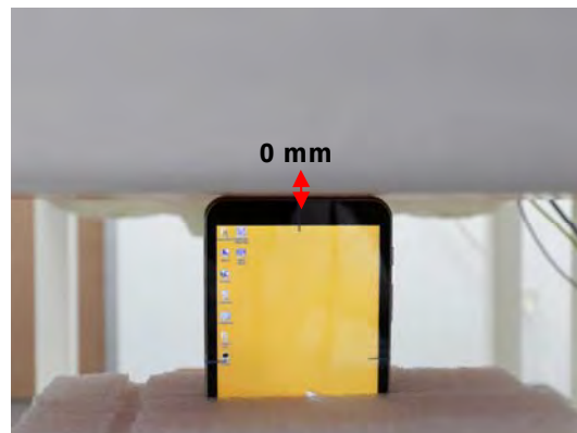
Fig.4 Top side to flat phantom
