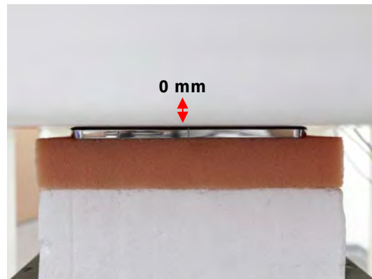
Fig.3 Back side to flat phantom
