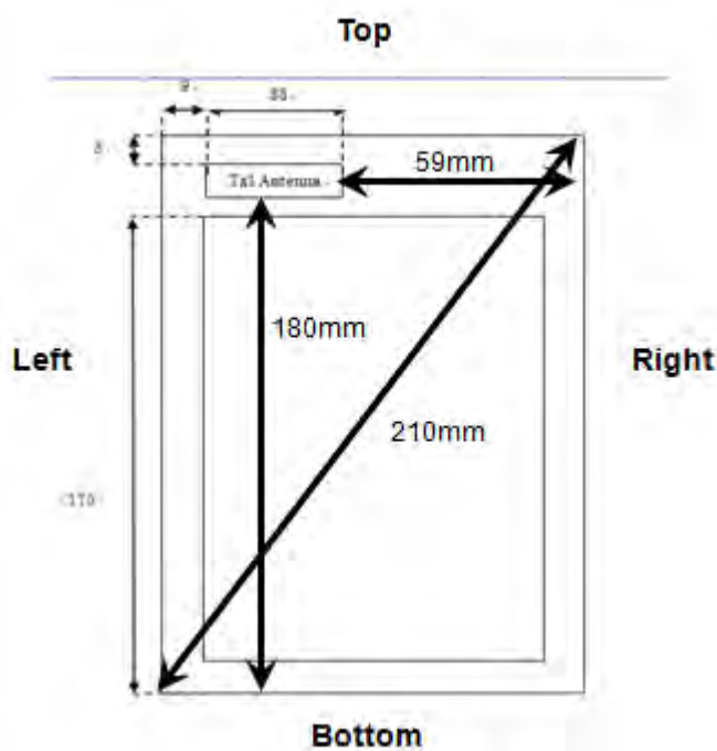
Fig.8 Antenna position (Front view)
