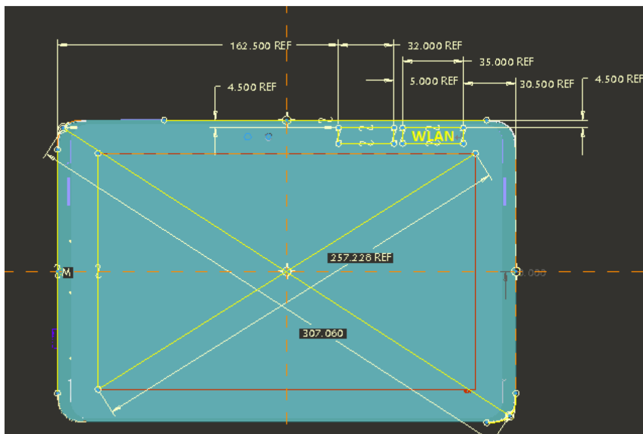
Fig.7 Antenna position of EUT (Front view)
