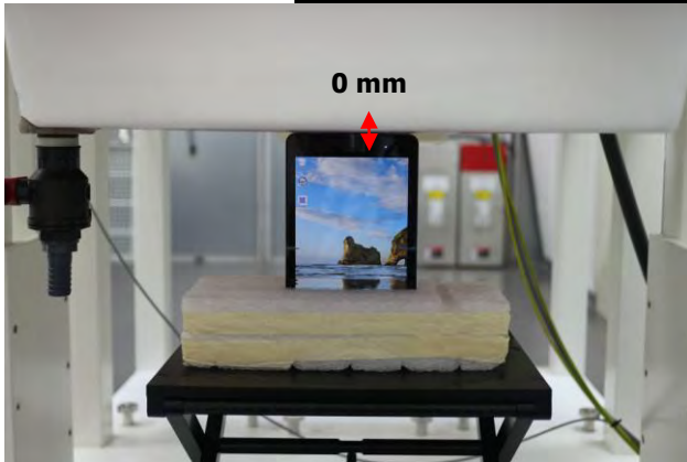
Fig.3 EUT Top side to flat phantom
