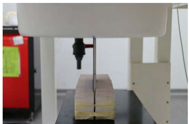
Fig.5 EUT Bottom side to flat phantom
