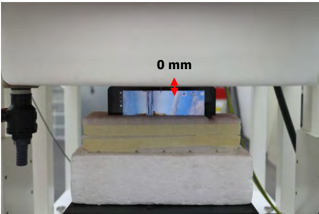
Fig.7 EUT Left side to flat phantom
