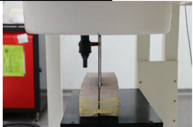
Fig.3 EUT Top side to flat phantom
