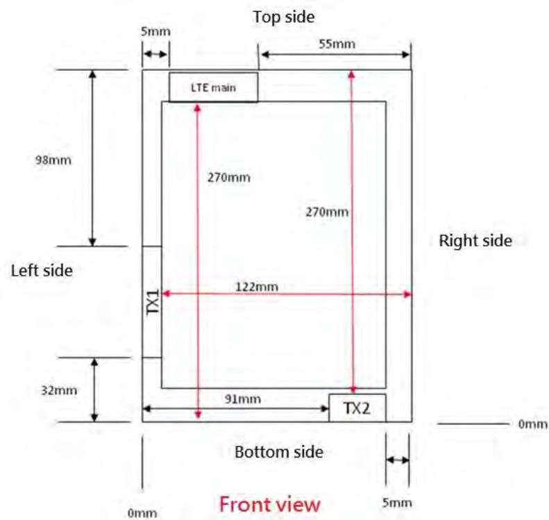
Fig.12 Antenna position of EUT (Front view)
