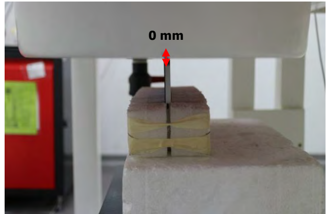
Fig.6 EUT Right side to flat phantom
