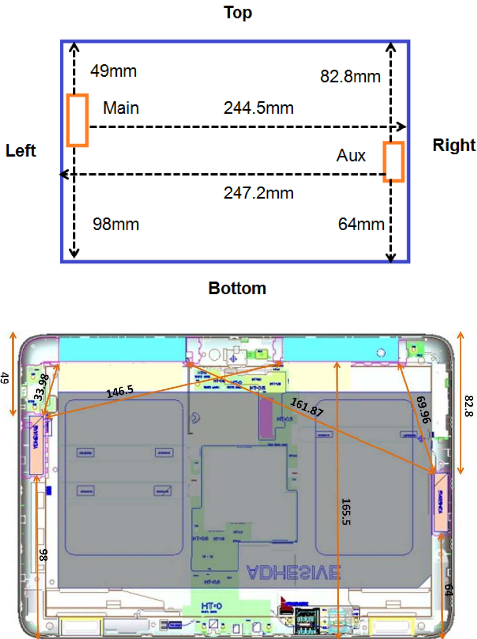
Fig.8 Antenna position of EUT
