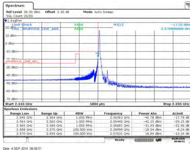
BAND38_5MHz_QPSK_37775_25RB#0
