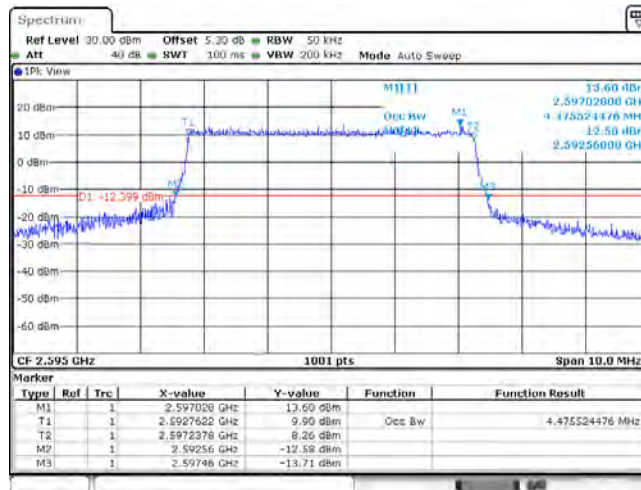
BAND38_5MHz_QPSK_38000_25RB#0
