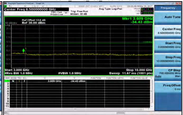
3GHz~10GHz EVDO BC0 MidCH384-836.52
