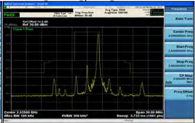
Mask Band7 5MHz QPSK 1 24 MidCH21100-2535
