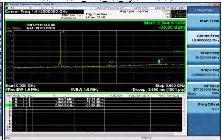
30MHz~3GHz EVDO BC0 HighCH777-848.31
