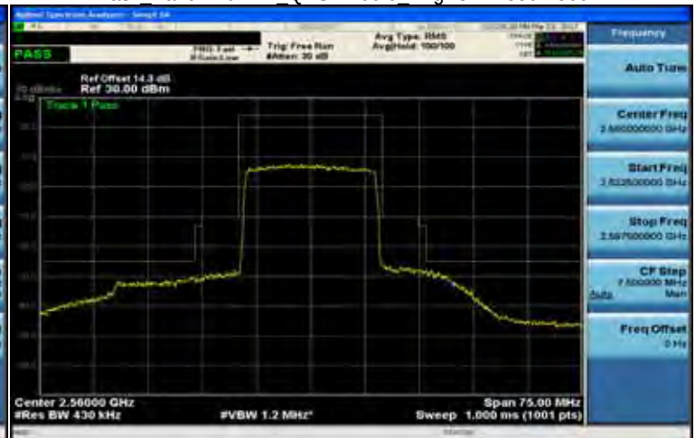
Mask Band7 20MHz_QPSK 100 0 HighCH21350-2560
