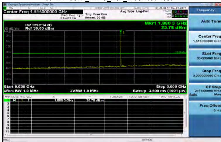
30MHz~3GHz EVDO BC1 MidCH600-1880
