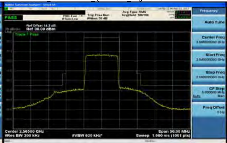
Mask Band7 10MHz_QPSK 50 0_High CH21400-2565
