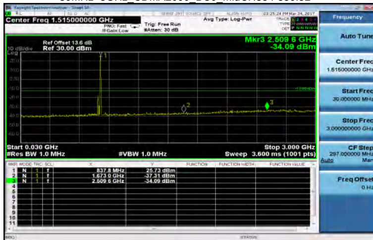
30MHz~3GHz CDMA2000 BC0 MidCH384-836.52
