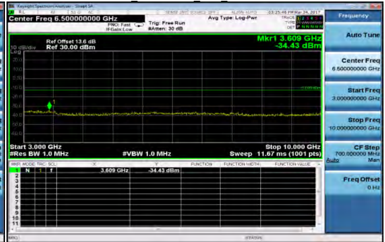
3GHz~10GHz CDMA2000 BC0 MidCH384-836.52
