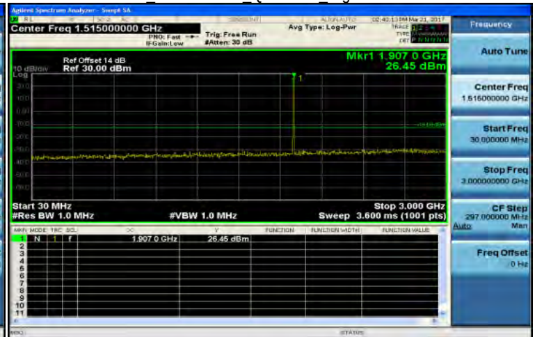
30MHz~3GHz Band2 5MHz QPSK 1 0 HighCH19175-1907.5
