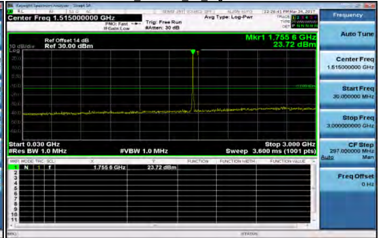
30MHz~3GHz WCDMA B4 HighCH1513-1752.6
