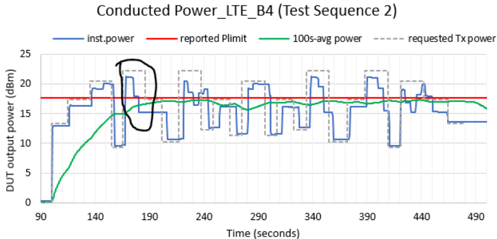
Figure 6-2 Sample plot of time-varying conducted power for LTE Band 4
