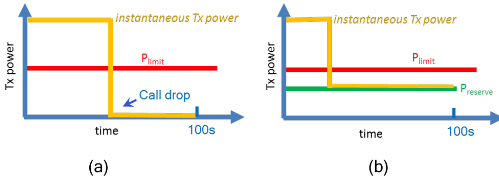
Figure 2-1 Smart Transmit Operation: (a) Transmit at high power when needed and permitted; (b) Transmit with reserve power to support continuous transmission at a minimum power level ( P_{reserve} ).
