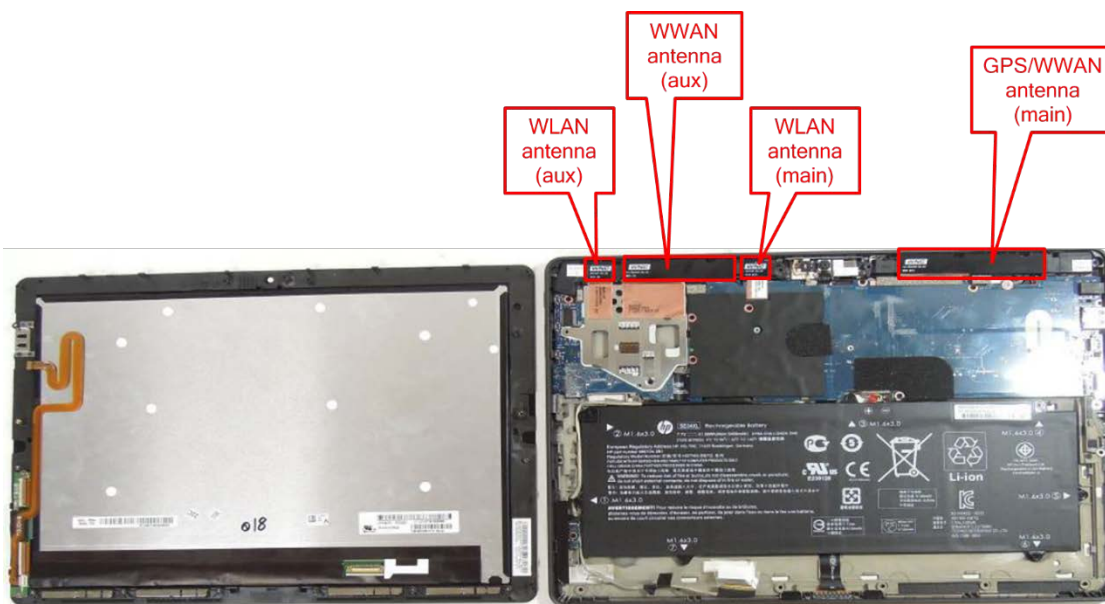
Figure 3-2 WWAN and WLAN antenna locations
