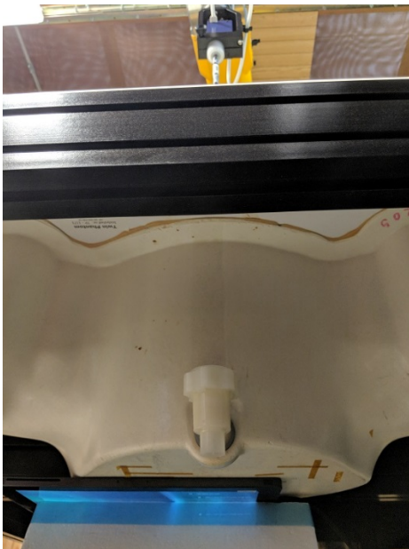
Figure 7-1 SAR measurement setup
