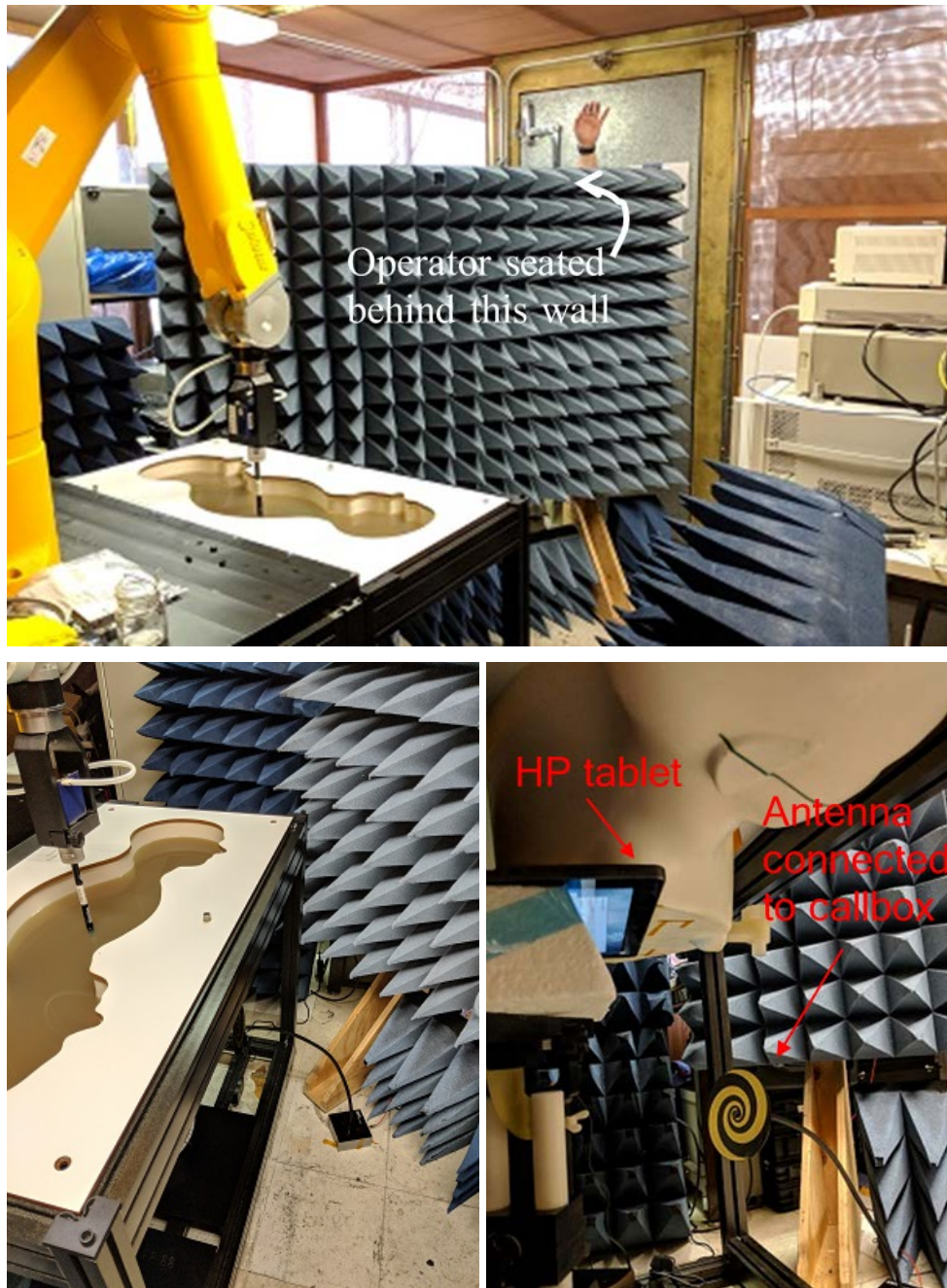
Figure 7-2 Path loss calibration setup
