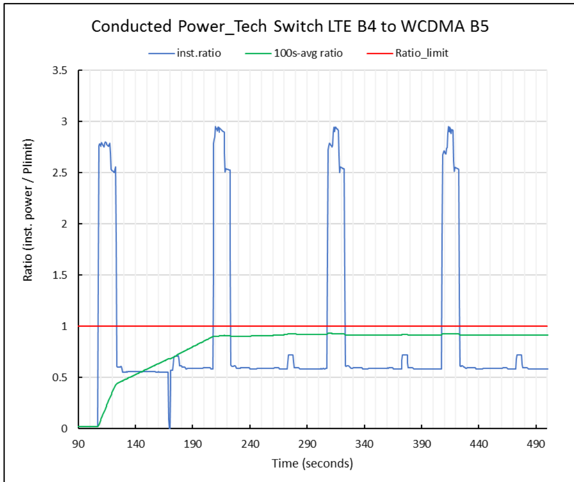
Plot 2: Ratio of instantaneous Tx power (mW) to its corresponding reported P_{limit} versus time and the time averaged ratio does not exceed “1” in any 100s-time window (Eq. (4) in Section 5.3.3).
