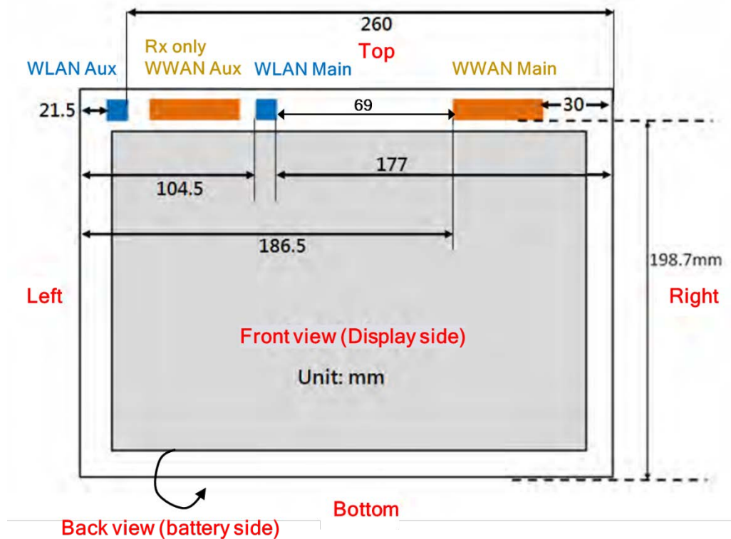
Figure 5-2 Test positions of EUT for SAR assessment
