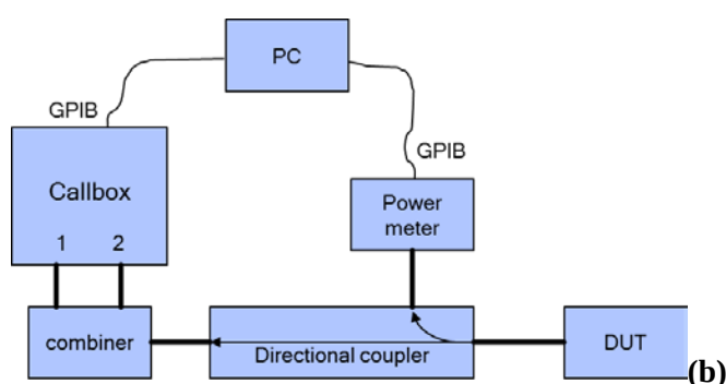
Figure 6-1 Conducted power measurement setup
