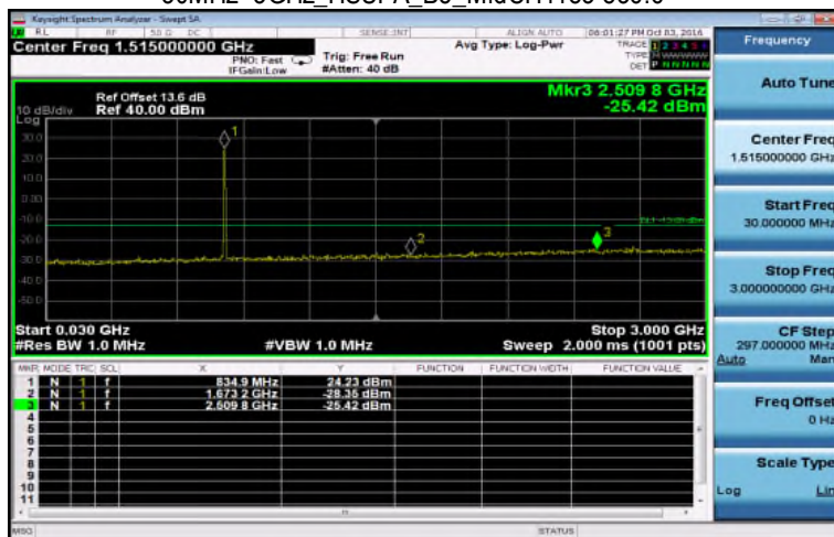
30MHz~3GHz_HSUPA_B5_MidCH4183-836.6
