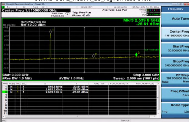
30MHz~3GHz_HSDPA_B5_HighCH4233-846.6
