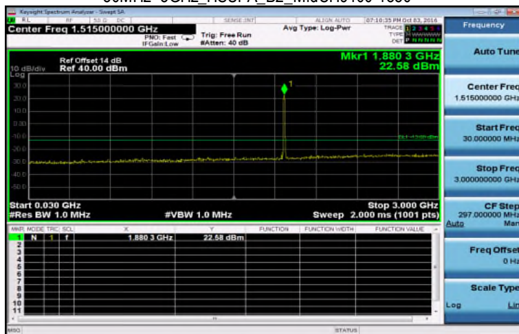
30MHz~3GHz_HSUPA_B2_MidCH9400-1880
