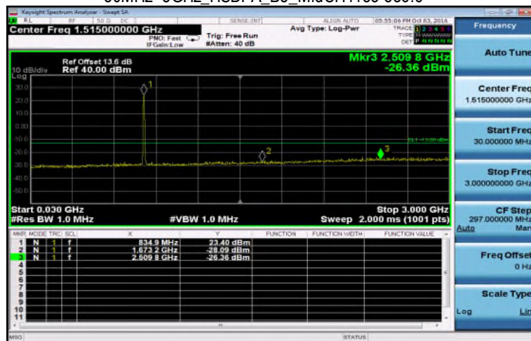
30MHz~3GHz_HSDPA_B5_MidCH4183-836.6
