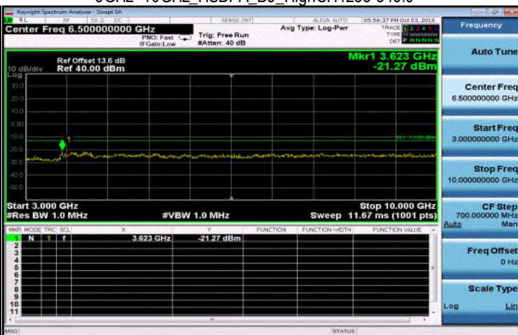
3GHz~10GHz_HSDPA_B5_HighCH4233-846.6
