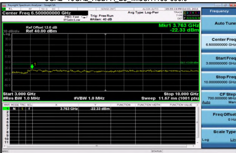
3GHz~10GHz_HSDPA_B5_MidCH4183-836.6
