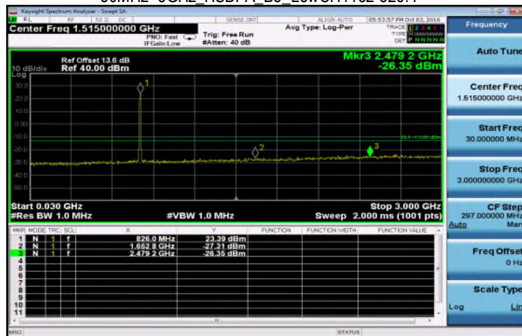
30MHz~3GHz_HSDPA_B5_LowCH4132-826.4
