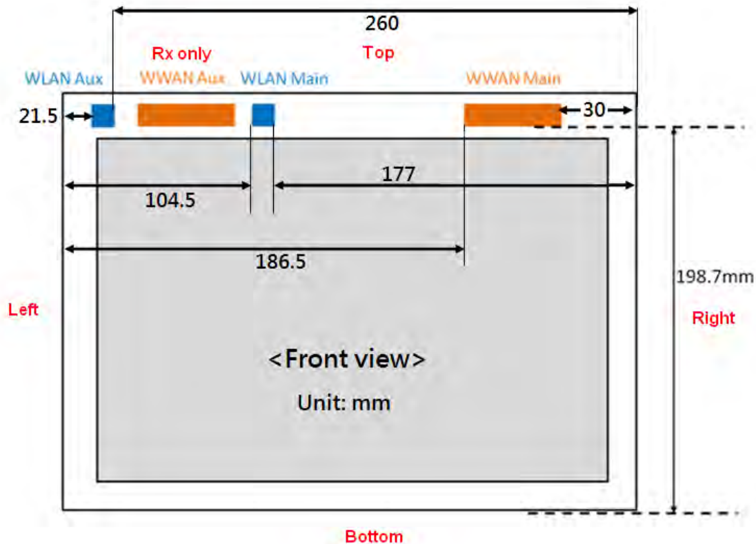
Fig.8 Antenna position of EUT (Front view)
