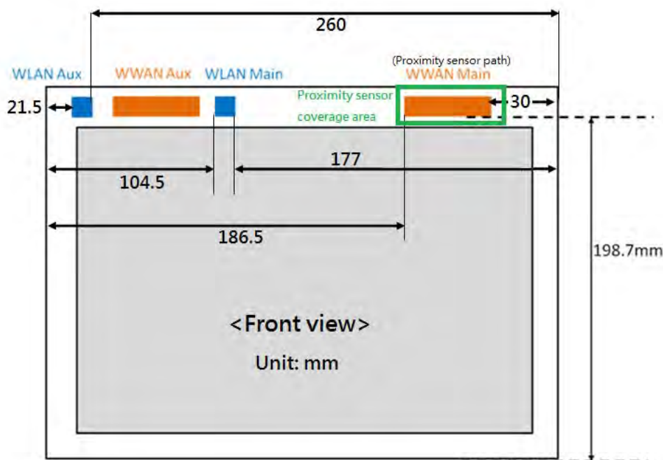
Fig.11 Antenna position of EUT (Front view)
