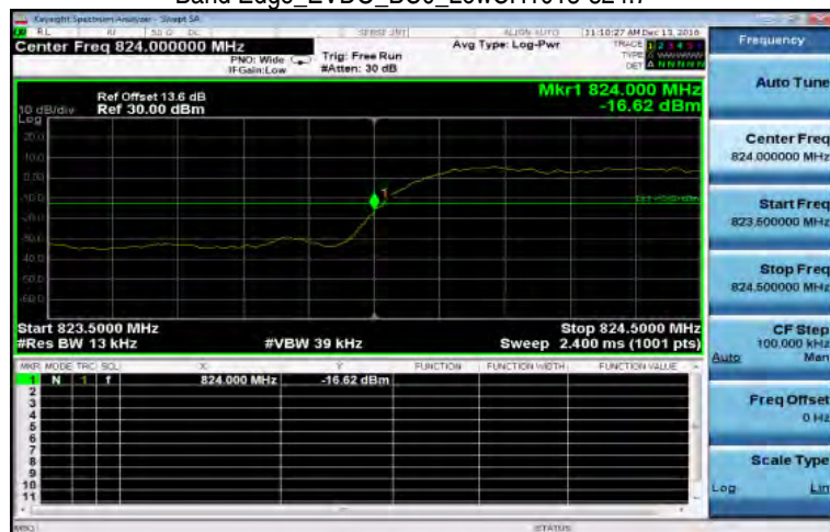
Band Edge_EVDO_BC0_LowCH1013-824.7
