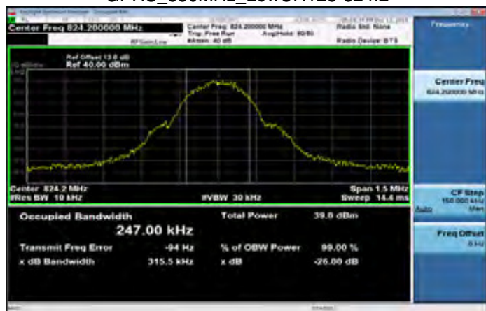
GPRS_850MHz_LowCH128-824.2
