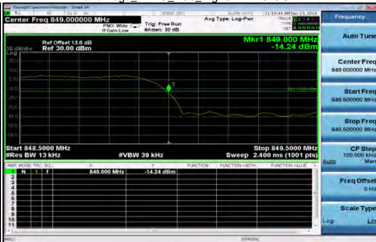
Band Edge_EVDO_BC0_HighCH777-848.31
