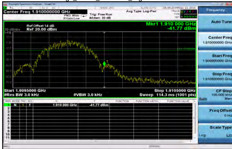
Band Edge_EDGE_1900MHz_HighCH810-1909.8
