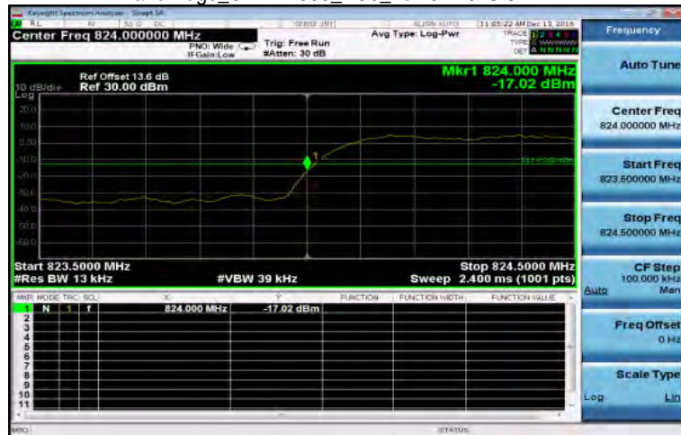
Band Edge_CDMA2000_BC0_LowCH1013-824.7
