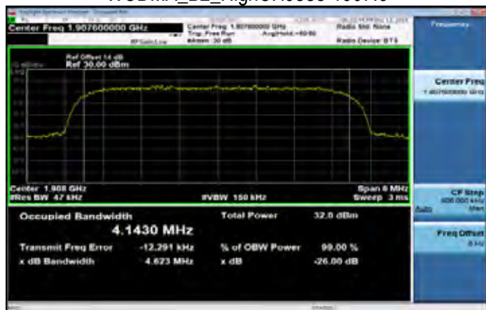
WCDMA_B2_HighCH9538-1907.6
