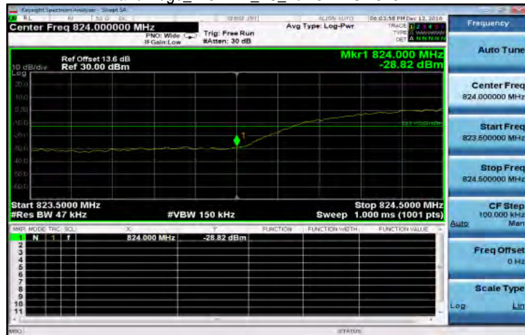
Band Edge_WCDMA_B5_LowCH4132-826.4
