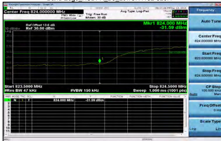
Band Edge_HSDPA_B5_LowCH4132-826.4
