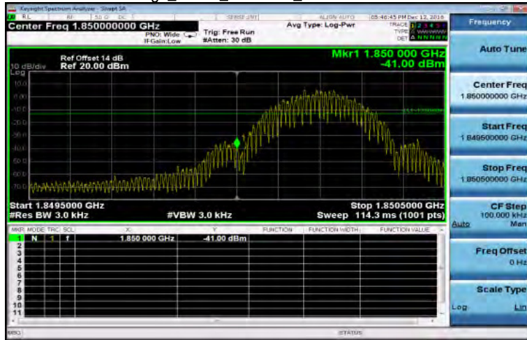
Band Edge_EDGE_1900MHz_LowCH512-1850.2
