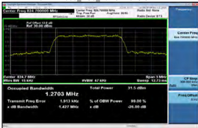
CDMA2000_BC0_LowCH1013-824.7
