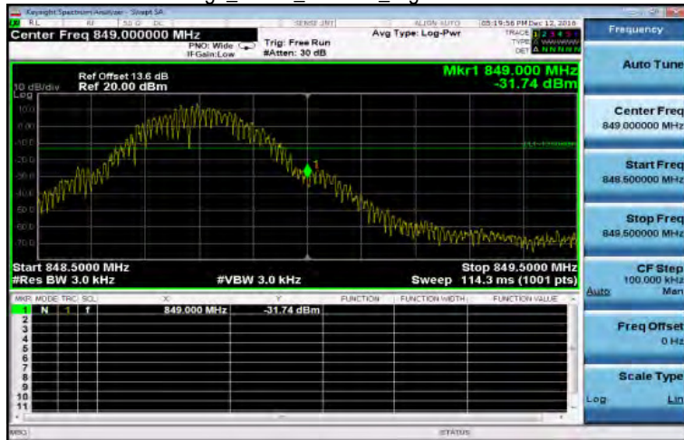
Band Edge_GPRS_850MHz_HighCH251-848.8
