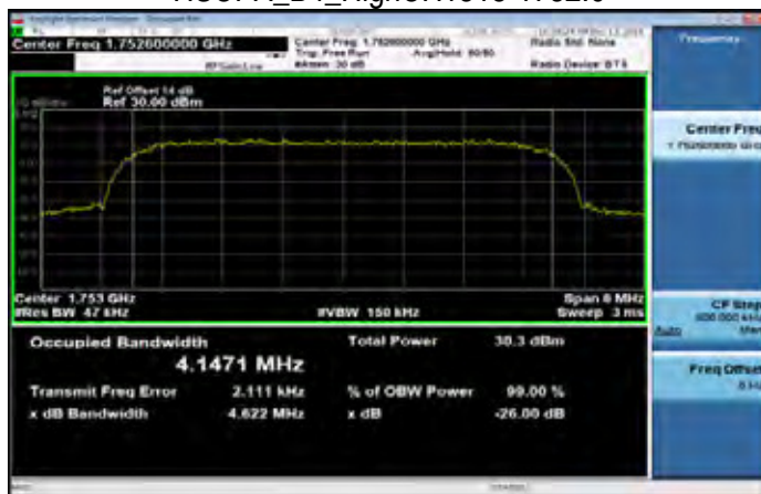
HSUPA_B4_HighCH1513-1752.6
