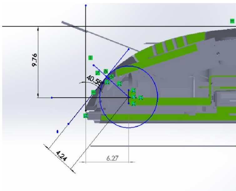
The surface edge along the curved
