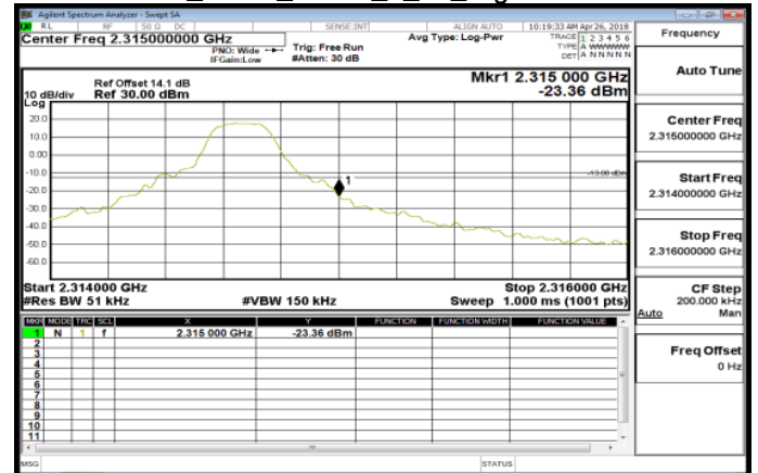
Band30_5MHz_QPSK_1_24_HighCH27735
