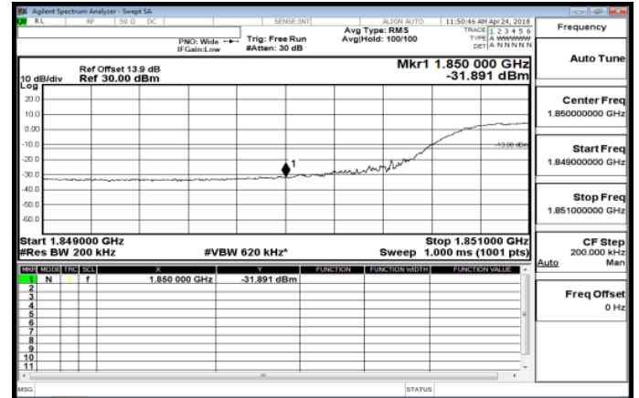
Band25_15MHz_QPSK_75_0_LowCH26115
