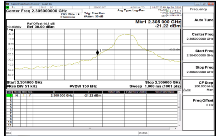
Band30_5MHz_QPSK_1_0_LowCH27685
