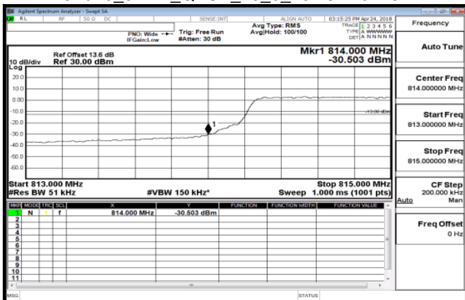
Band26_5MHz_QPSK_25_0_LowCH26715
