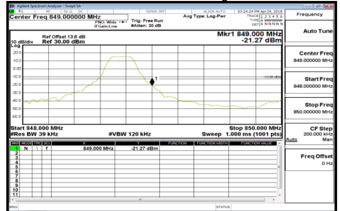
Band26_3MHz_QPSK_1_14_HighCH27025
