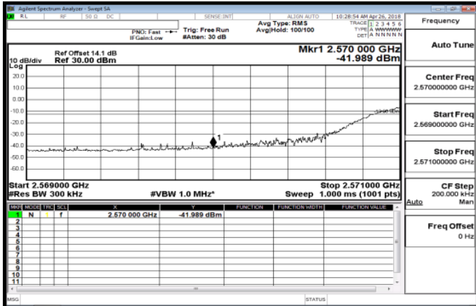
Band38_20MHz_QPSK_100_0_LowCH37850
