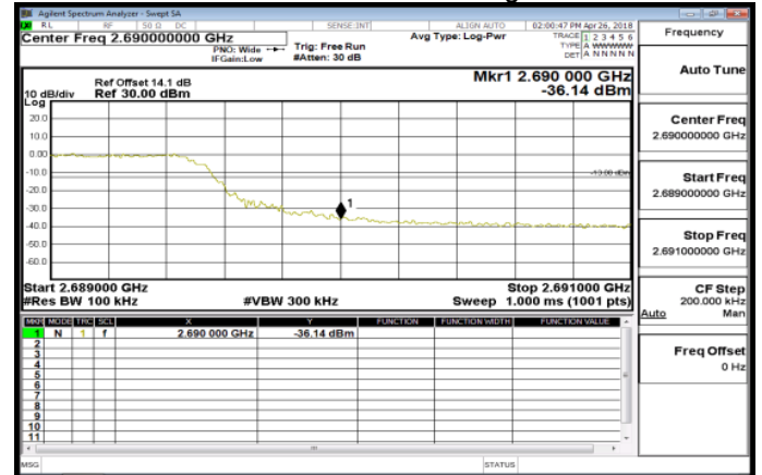
Band41_10MHz_QPSK_50_0_HighCH41540
