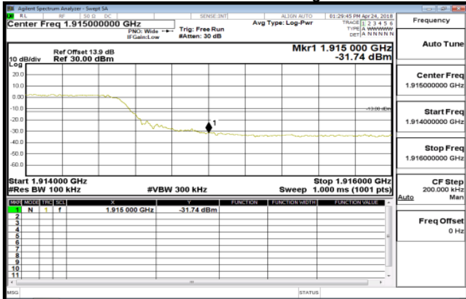
Band25_10MHz_QPSK_50_0_HighCH26640
