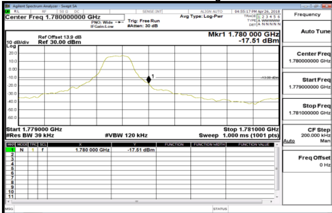
Band66_3MHz_QPSK_1_14_HighCH132657
