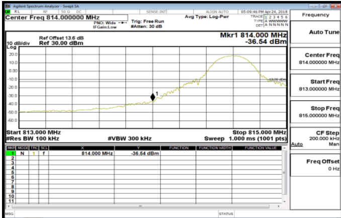
Band26_10MHz_QPSK_1_0_LowCH26740
