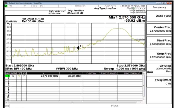
Band38_10MHz_QPSK_1_0_LowCH37800
