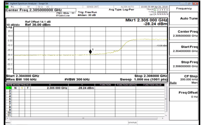
Band30_10MHz_QPSK_50_0_HighCH27710
