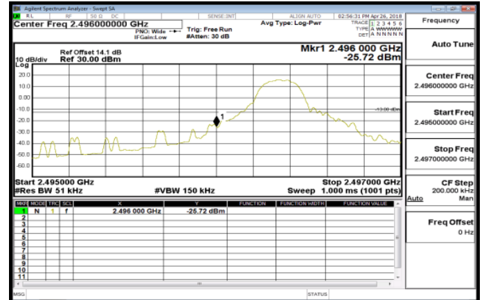
Band41_5MHz_QPSK_1_0_LowCH39675
