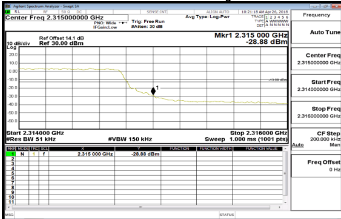
Band30_10MHz_QPSK_1_0_LowCH27710
