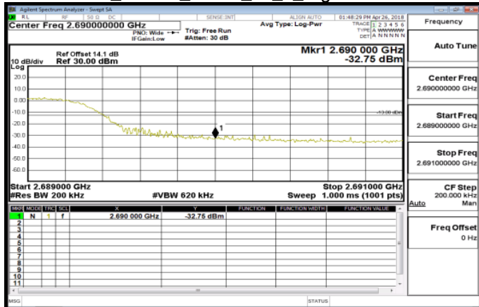
Band41_15MHz_QPSK_75_0_HighCH41515
