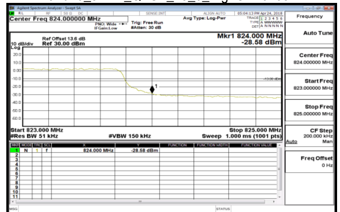
Band26_5MHz_QPSK_25_0_HighCH26765
