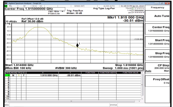
Band25_10MHz_QPSK_1_49_HighCH26640
