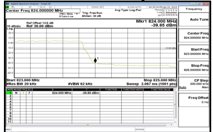
Band26_1_4MHz_QPSK_6_0_HighCH26783
