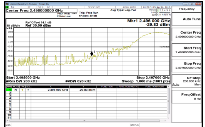
Band41_15MHz_QPSK_1_0_LowCH39725
