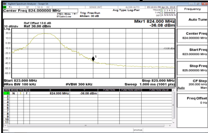
Band26_10MHz_QPSK_1_49_HighCH26740
