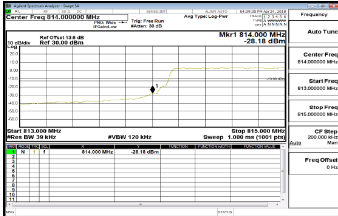
Band26_3MHz_QPSK_15_0_LowCH26705
