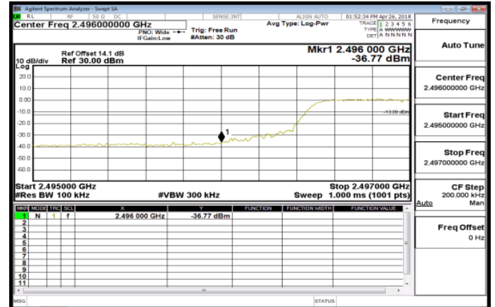
Band41_10MHz_QPSK_50_0_LowCH39700
