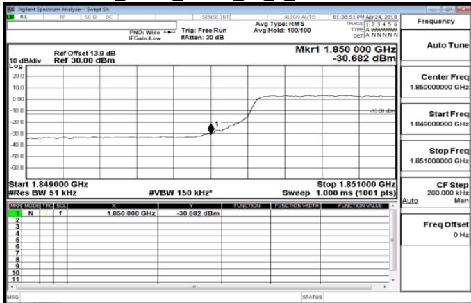
Band25_5MHz_QPSK_25_0_LowCH26065
