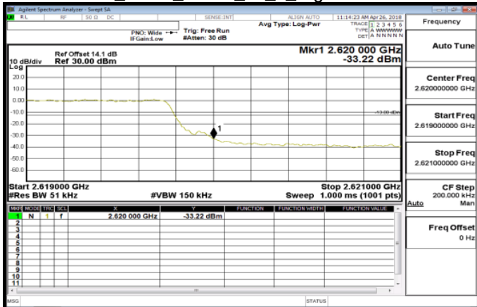
Band38_5MHz_QPSK_25_0_HighCH38225
