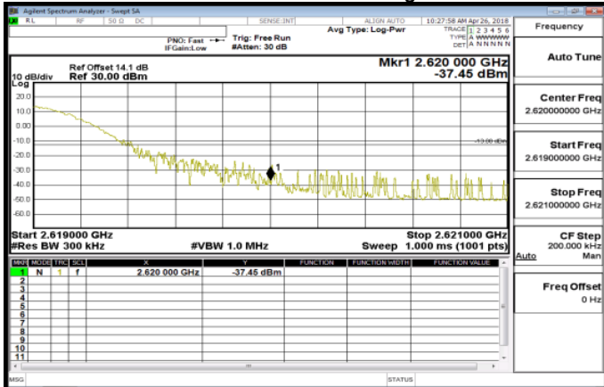
Band38_20MHz_QPSK_1_99_HighCH38150
