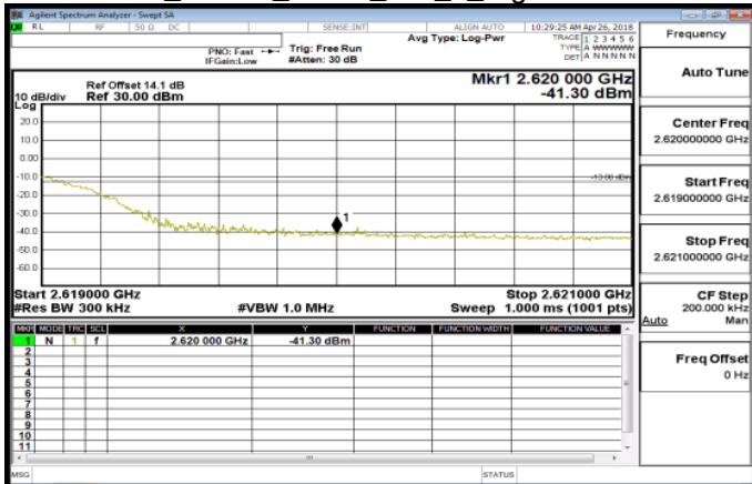
Band38_20MHz_QPSK_100_0_HighCH38150
