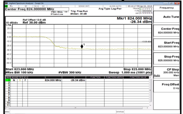
Band26_10MHz_QPSK_50_0_HighCH26740
