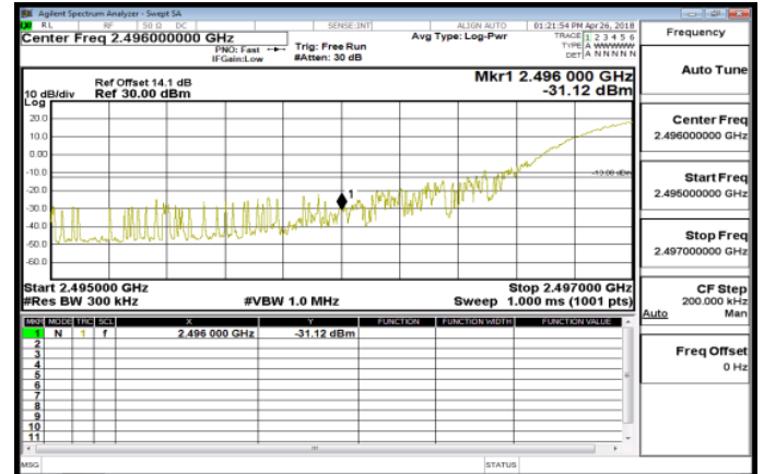
Band41_20MHz_QPSK_1_0_LowCH39750
