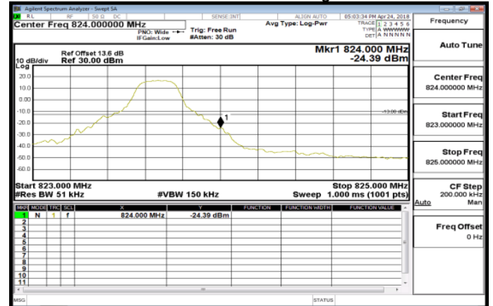
Band26_5MHz_QPSK_1_24_HighCH26765
