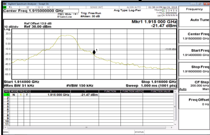
Band25_5MHz_QPSK_1_24_HighCH26665
