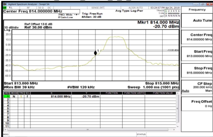
Band26_3MHz_QPSK_1_0_LowCH26705
