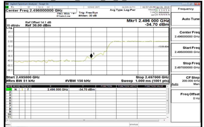
Band41_5MHz_QPSK_25_0_LowCH39675
