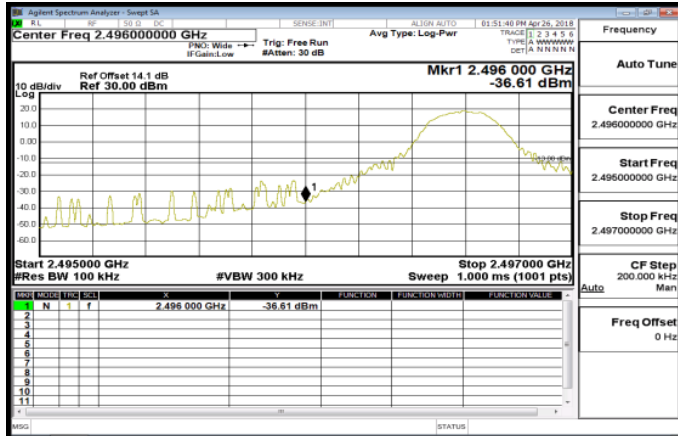
Band41_10MHz_QPSK_1_0_LowCH39700
