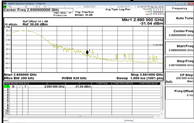
Band41_15MHz_QPSK_1_74_HighCH41515
