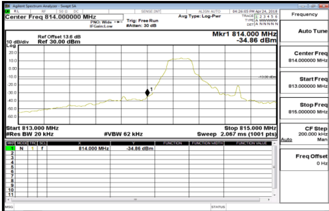
Band26_1_4MHz_QPSK_1_0_LowCH26697-814.7
