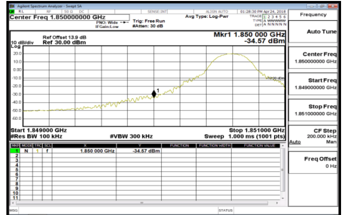
Band25_10MHz_QPSK_1_0_LowCH26090
