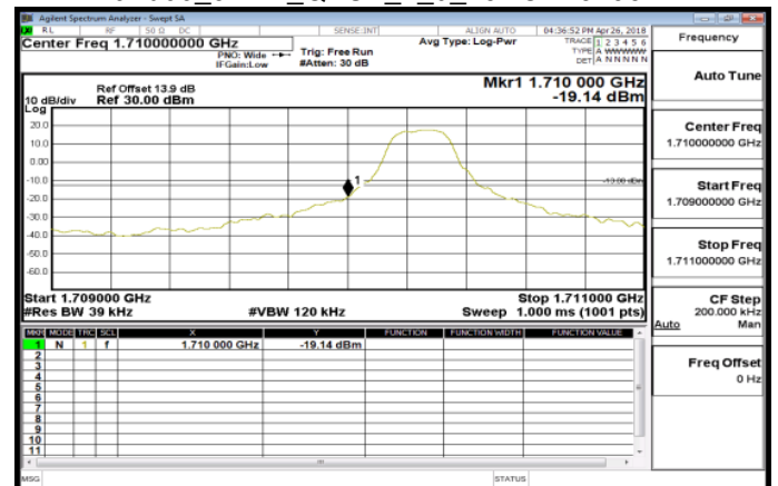
Band66_3MHz_QPSK_1_0_LowCH131987
