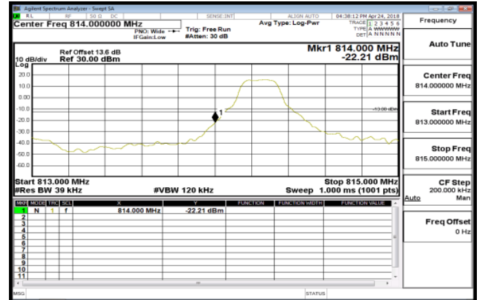
Band26_3MHz_QPSK_1_0_LowCH26705
