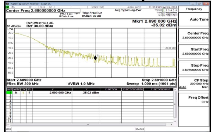
Band41_20MHz_QPSK_1_99_HighCH41490
