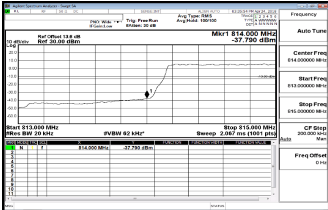
Band26_1_4MHz_QPSK_6_0_LowCH26697
