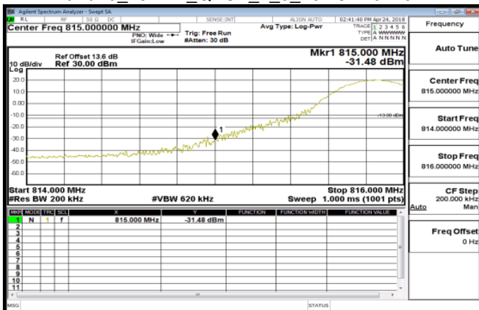
Band26_15MHz_QPSK_1_0_LowCH26775
