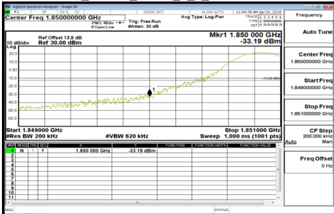
Band25_15MHz_QPSK_1_0_LowCH26115
