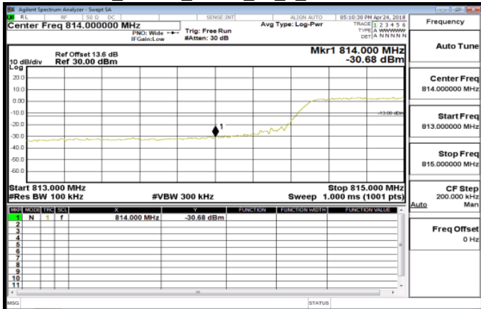
Band26_10MHz_QPSK_50_0_LowCH26740
