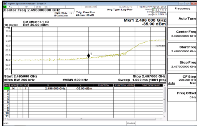
Band41_15MHz_QPSK_75_0_LowCH39725
