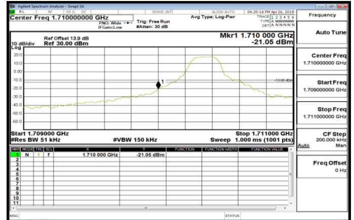
Band66_5MHz_QPSK_1_0_LowCH131997
