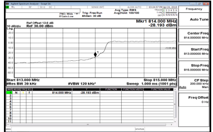
Band26_3MHz_QPSK_15_0_LowCH26705
