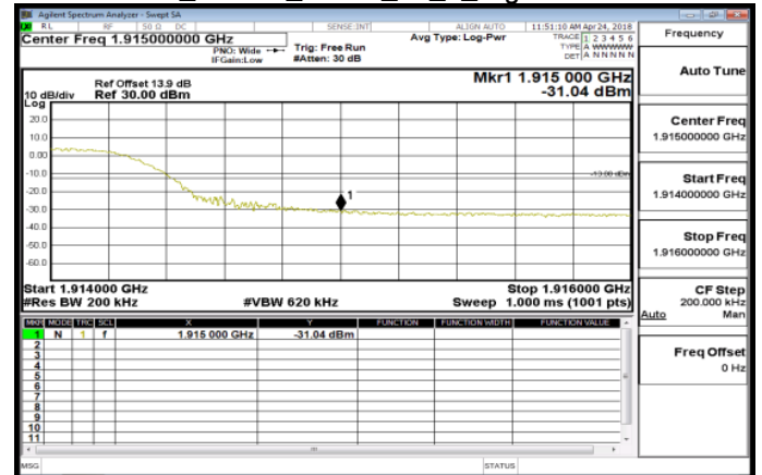
Band25_15MHz_QPSK_75_0_HighCH26615
