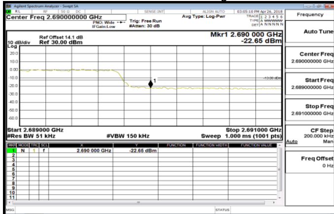
Band41_5MHz_QPSK_25_0_HighCH41565
