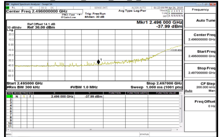
Band41_20MHz_QPSK_100_0_LowCH39750
