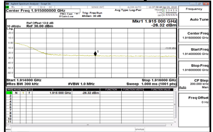
Band25_20MHz_QPSK_100_0_HighCH26590
