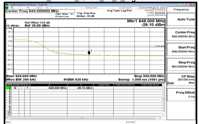
Band26_15MHz_QPSK_75_0_HighCH26965
