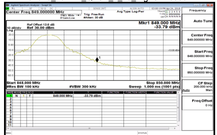
Band26_10MHz_QPSK_1_49_HighCH26990
