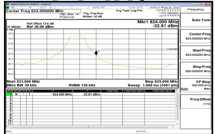
Band26_3MHz_QPSK_1_14_HighCH26775
