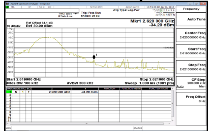
Band38_10MHz_QPSK_1_49_HighCH38200
