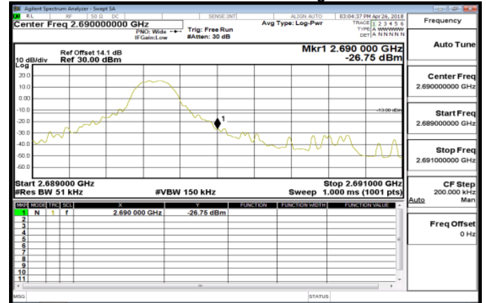
Band41_5MHz_QPSK_1_24_HighCH41565
