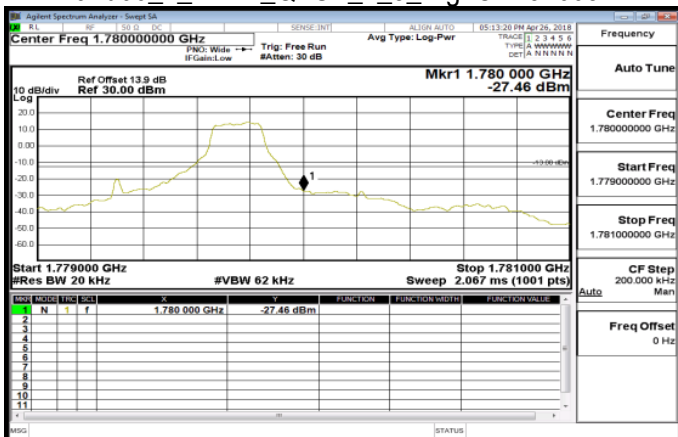
Band66_1_4MHz_QPSK_1_5_HighCH132665
