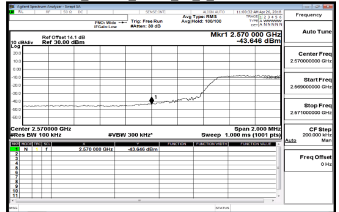
Band38_10MHz_QPSK_50_0_LowCH37800
