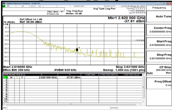
Band38_15MHz_QPSK_1_74_HighCH38175
