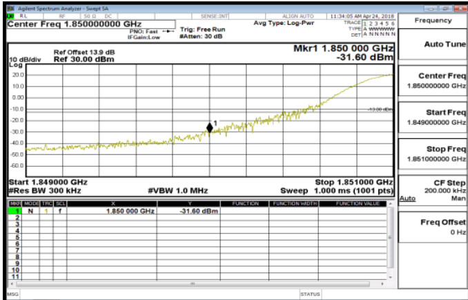
Band25_20MHz_QPSK_1_0_LowCH26140
