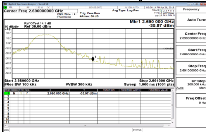
Band41_10MHz_QPSK_1_49_HighCH41540
