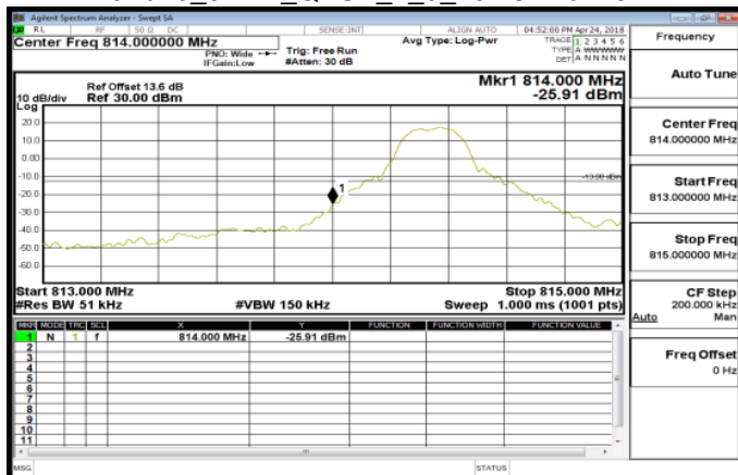
Band26_5MHz_QPSK_1_0_LowCH26715
