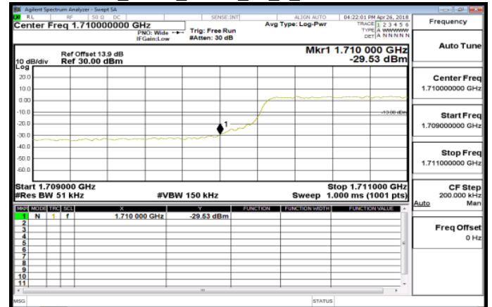
Band66_5MHz_QPSK_25_0_LowCH131997
