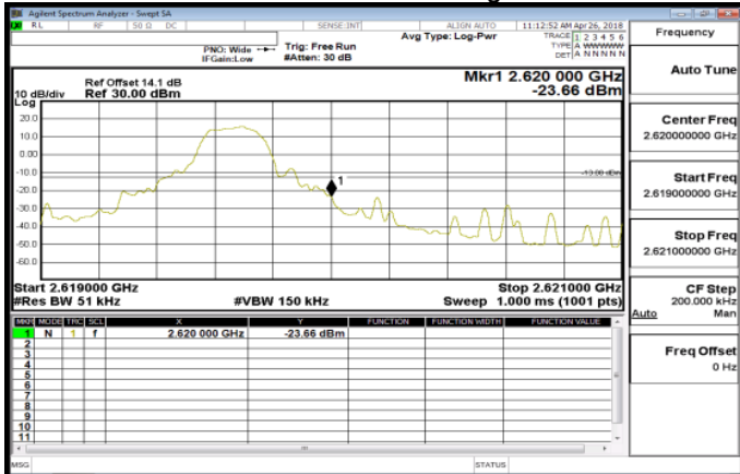
Band38_5MHz_QPSK_1_24_HighCH38225
