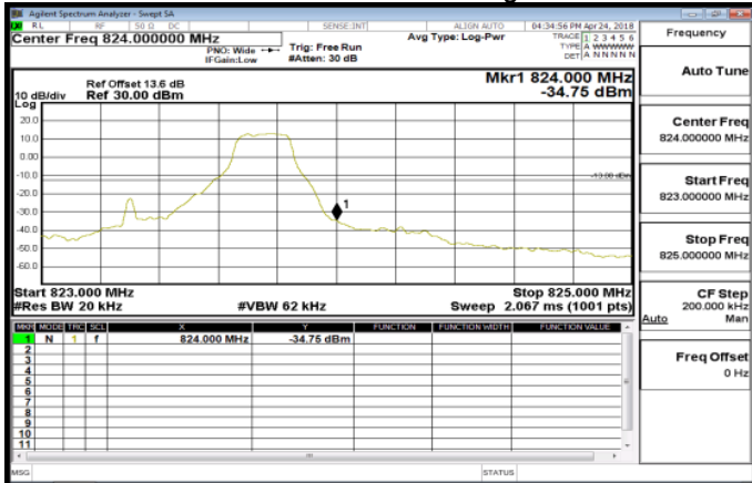
Band26_1_4MHz_QPSK_1_5_HighCH26783
