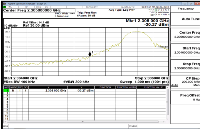
Band30_10MHz_QPSK_1_49_HighCH27710
