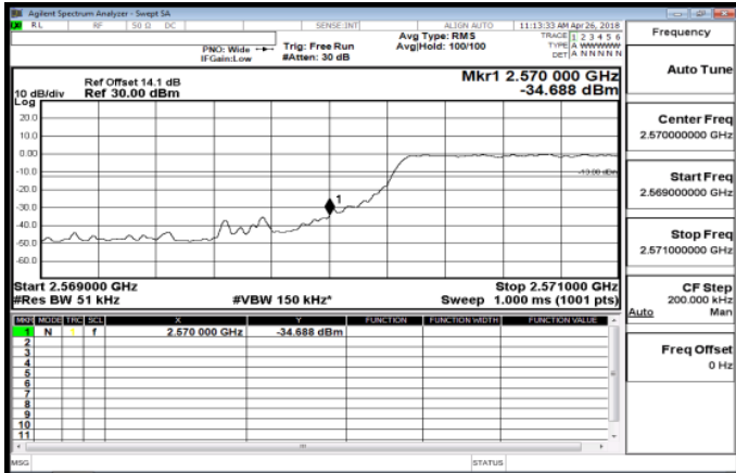
Band38_5MHz_QPSK_25_0_LowCH37775
