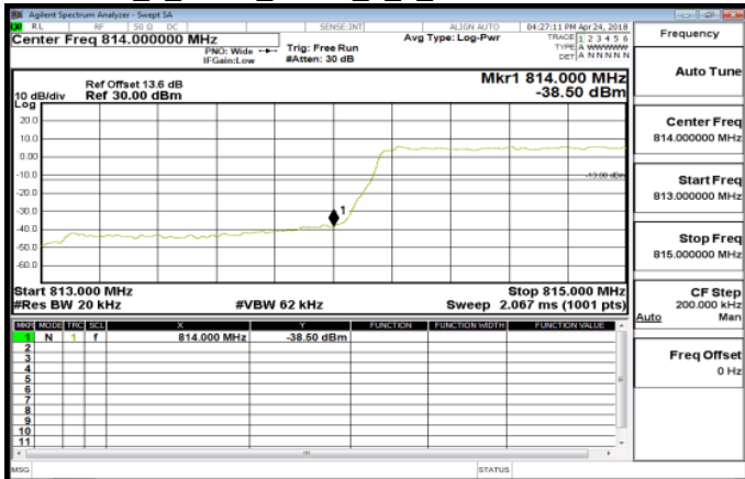
Band26_1_4MHz_QPSK_6_0_LowCH26697-814.7
