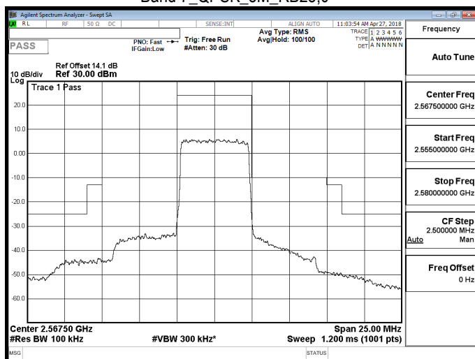
Band 7_QPSK_5M_RB25,0
