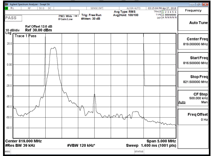
Part 90_Band 26_QPSK_3M_RB1,14
