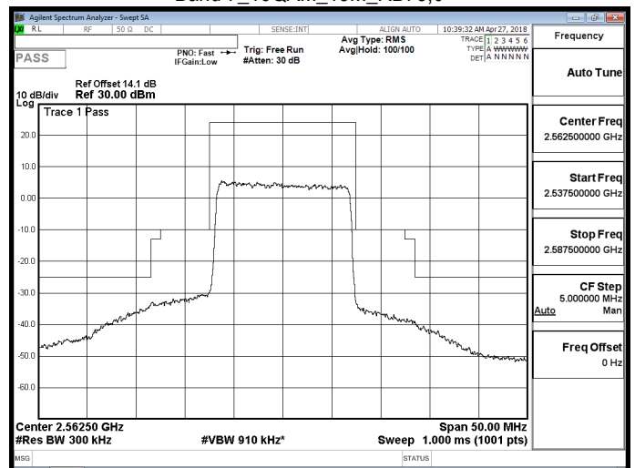
Band 7_16QAM_15M_RB75,0
