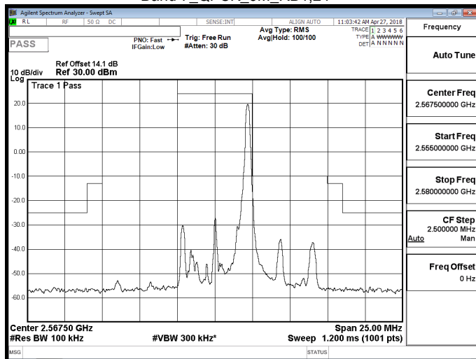
Band 7_QPSK_5M_RB25,0
