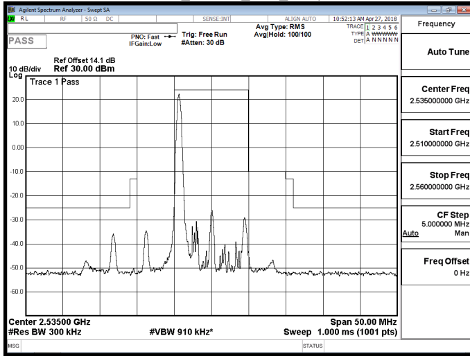
Band 7_16QAM_10M_RB1,49
