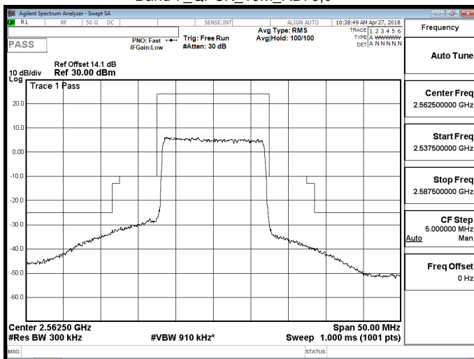
Band 7_QPSK_15M_RB75,0
