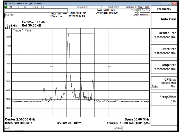
Band 7_16QAM_10M_RB1,49
