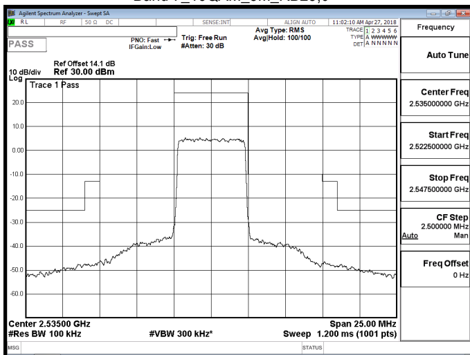
Band 7_16QAM_5M_RB25,0
