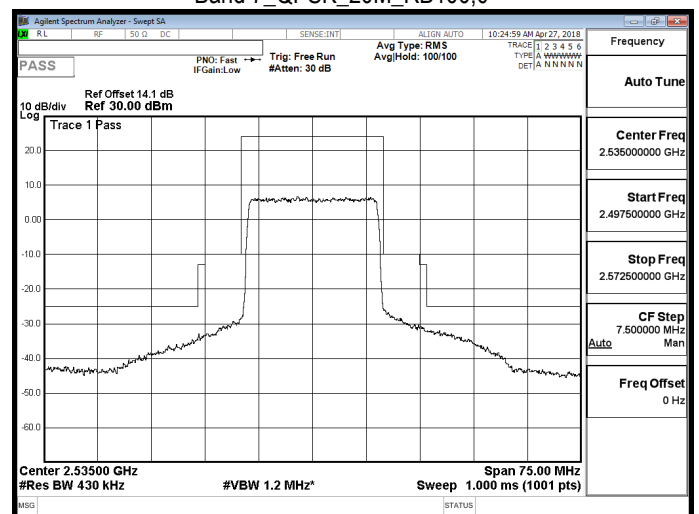
Band 7_QPSK_20M_RB100,0
