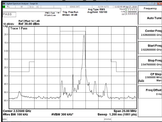
Band 7_16QAM_5M_RB25,0
