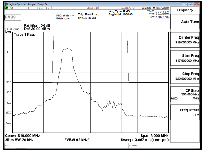
Part 90_Band 26_QPSK_1.4M_RB1,5
