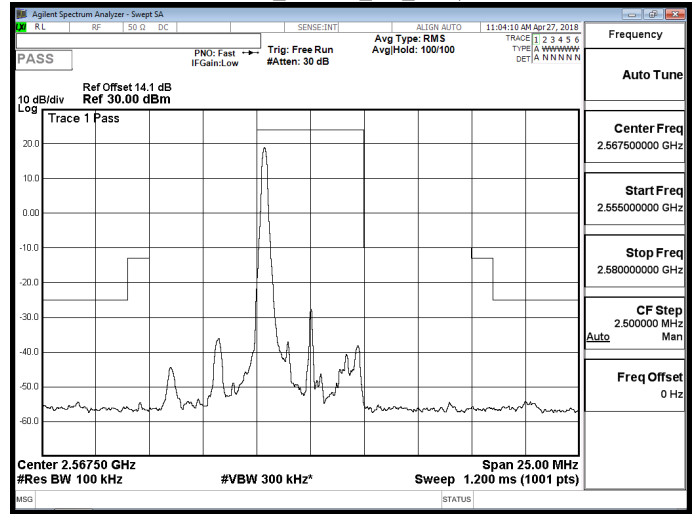
Band 7_16QAM_5M_RB1,24
