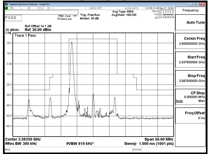
Band 7_16QAM_15M_RB1,74
