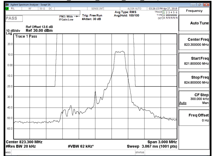
Part 90_Band 26_16QAM_1.4M_RB6,0
