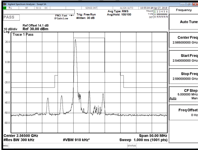
Band 7_QPSK_10M_RB1,49
