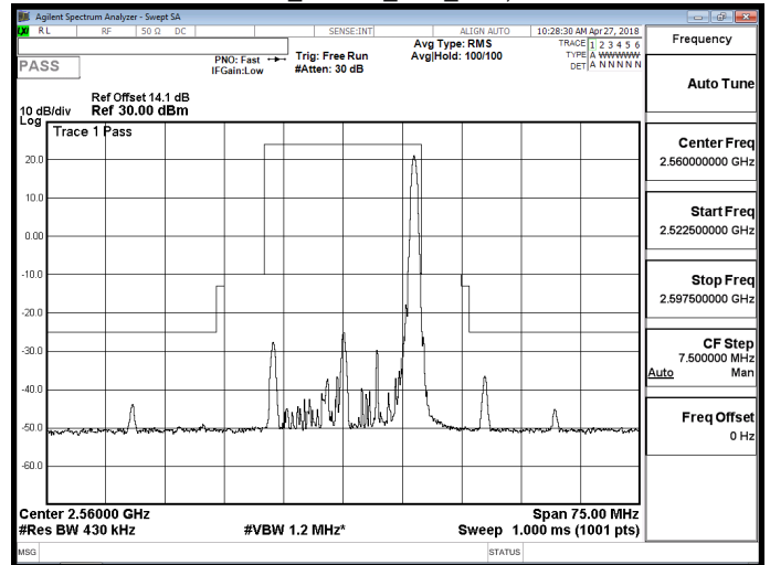
Band 7_16QAM_20M_RB100,0
