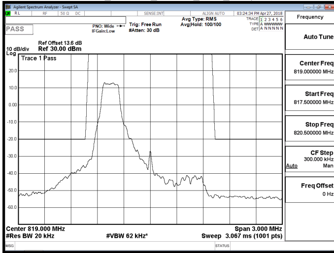
Part 90_Band 26_16QAM_1.4M_RB1,5
