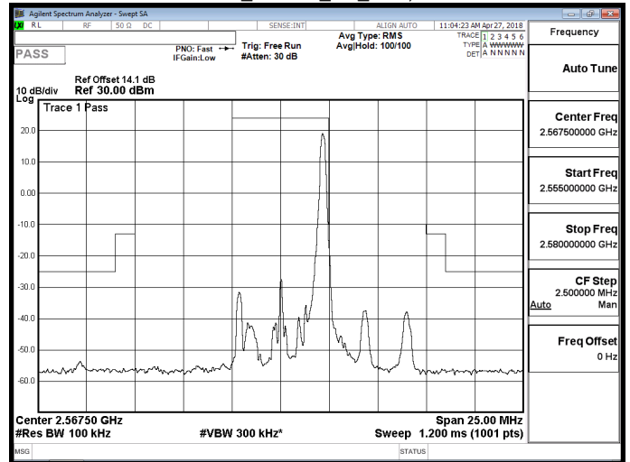
Band 7_16QAM_5M_RB25,0
