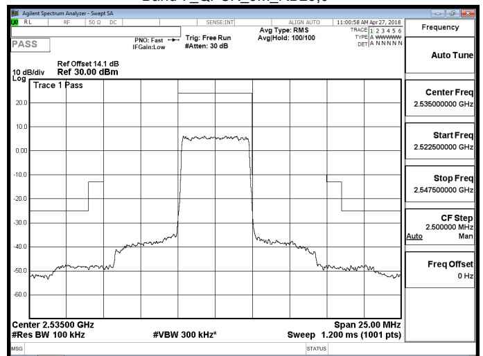
Band 7_QPSK_5M_RB25,0
