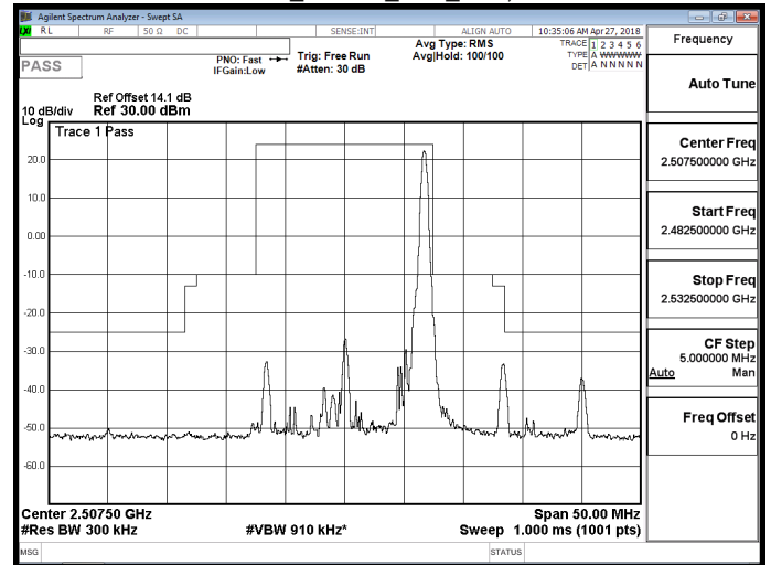
Band 7_16QAM_15M_RB75,0
