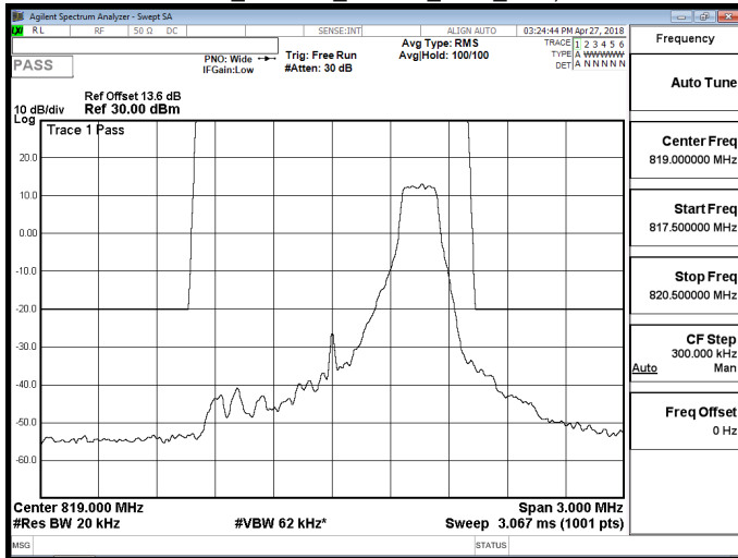
Part 90_Band 26_16QAM_1.4M_RB6,0
