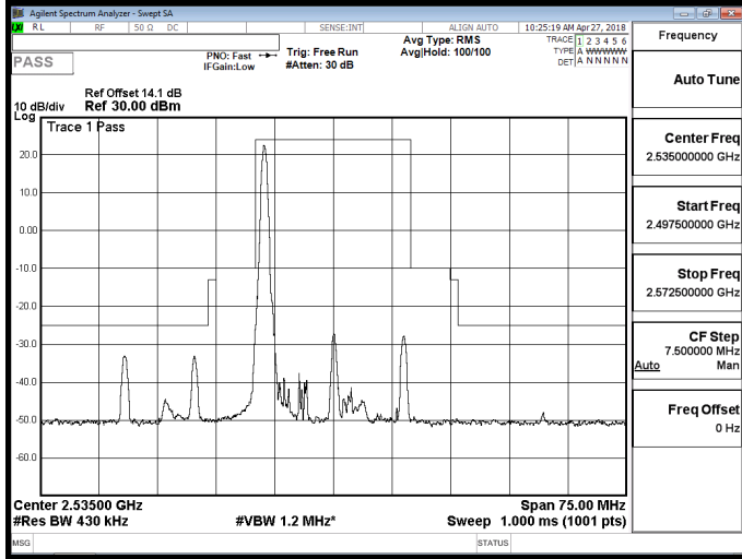
Band 7_16QAM_20M_RB1,99
