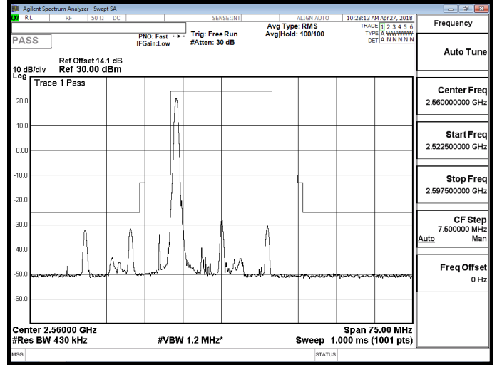
Band 7_16QAM_20M_RB1,99
