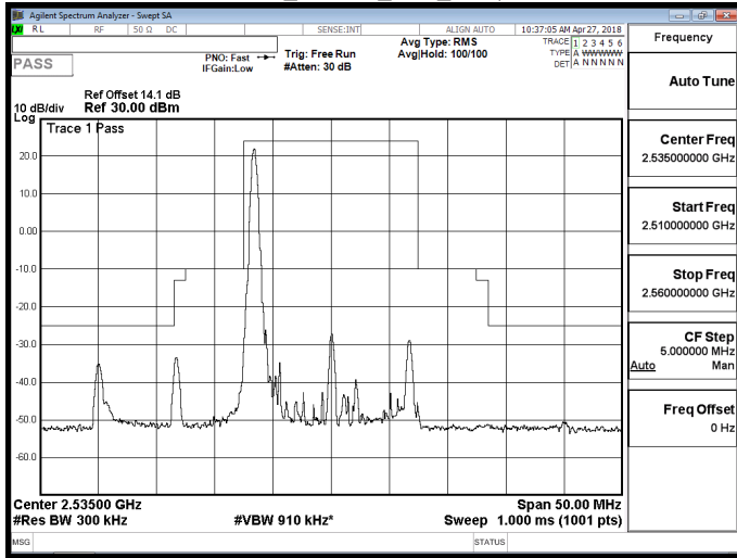
Band 7_16QAM_15M_RB1,74
