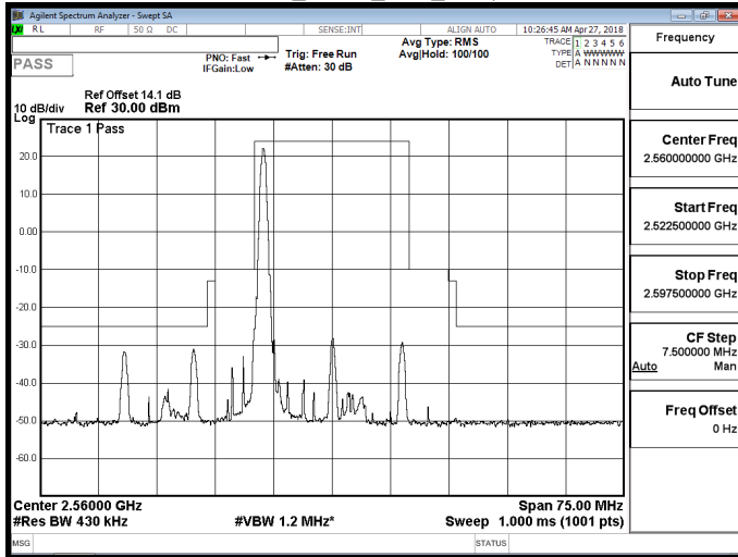
Band 7_QPSK_20M_RB1,99
