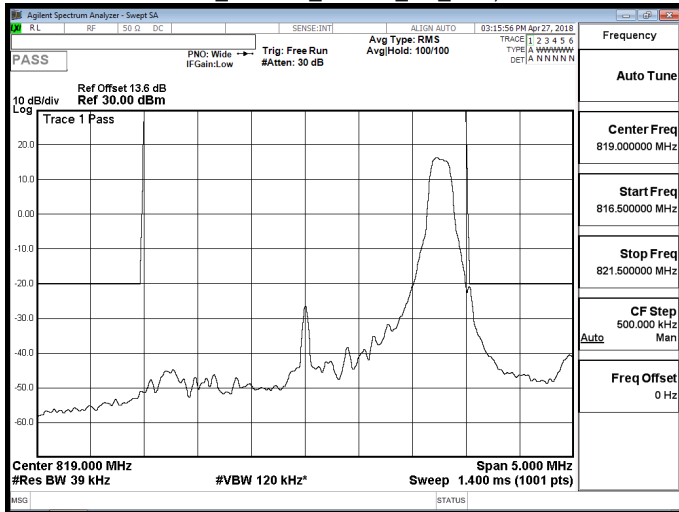
Part 90_Band 26_16QAM_3M_RB15,0
