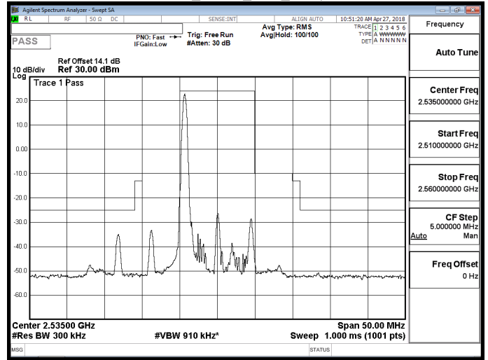
Band 7_QPSK_10M_RB1,49
