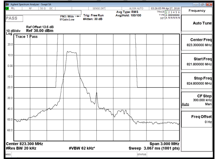
Part 90_Band 26_16QAM_1.4M_RB1,5
