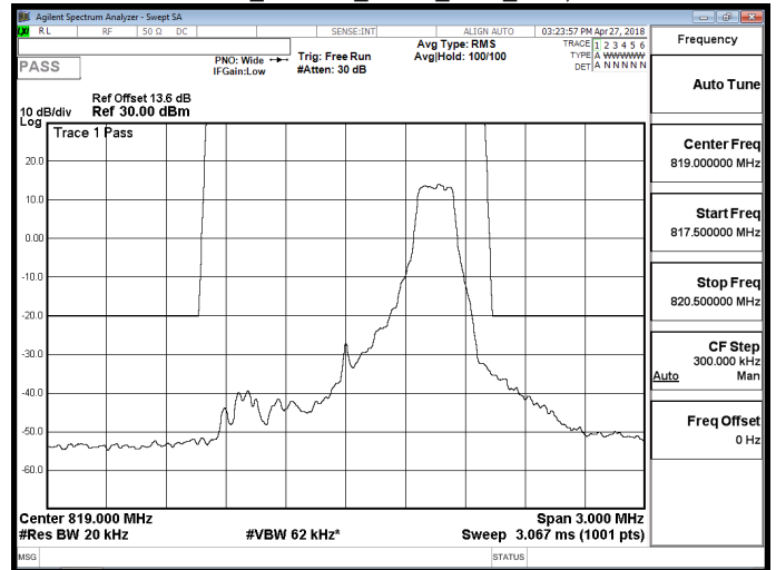
Part 90_Band 26_QPSK_1.4M_RB6,0
