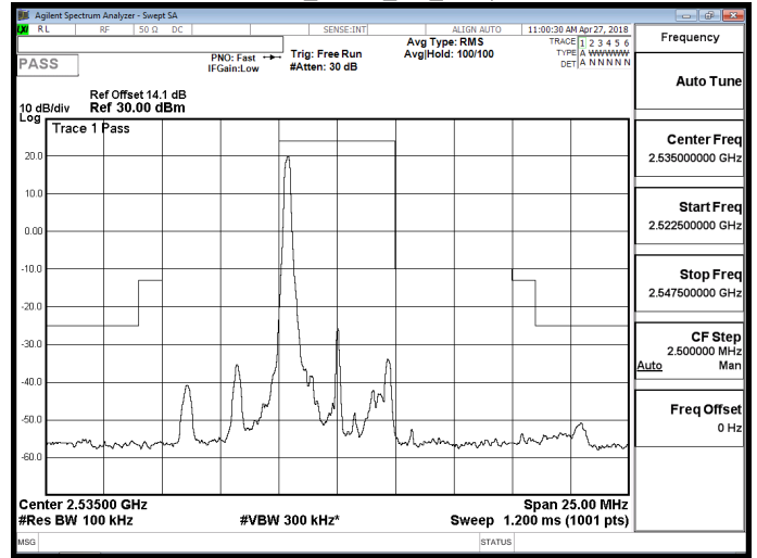
Band 7_QPSK_5M_RB1,24
