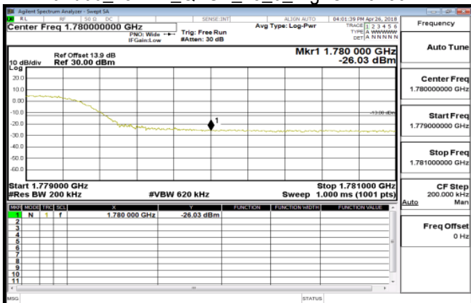
Band66_15MHz_QPSK_75_0_HighCH132597
