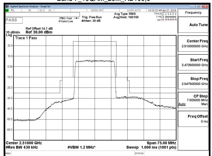
Band 7_16QAM_20M_RB100,0
