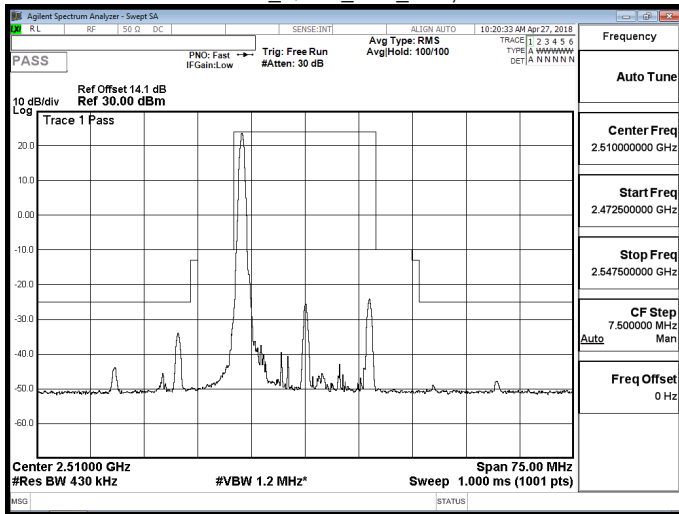
Band 7_QPSK_20M_RB1,99
