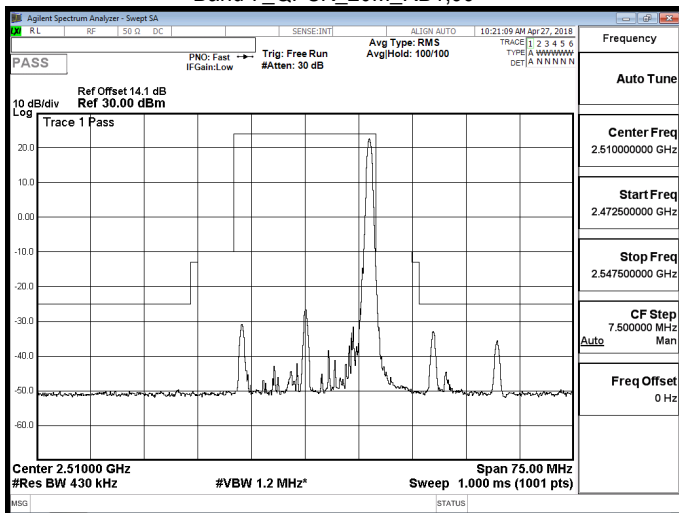
Band 7_QPSK_20M_RB100,0
