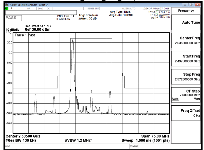
Band 7_QPSK_20M_RB1,99
