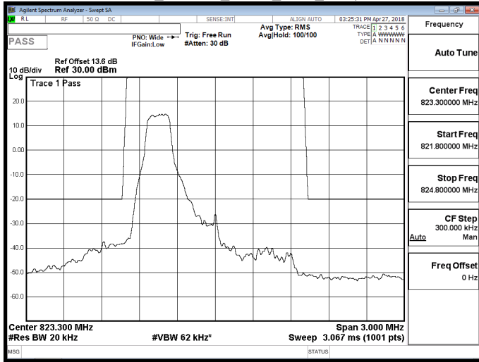
Part 90_Band 26_QPSK_1.4M_RB1,5
