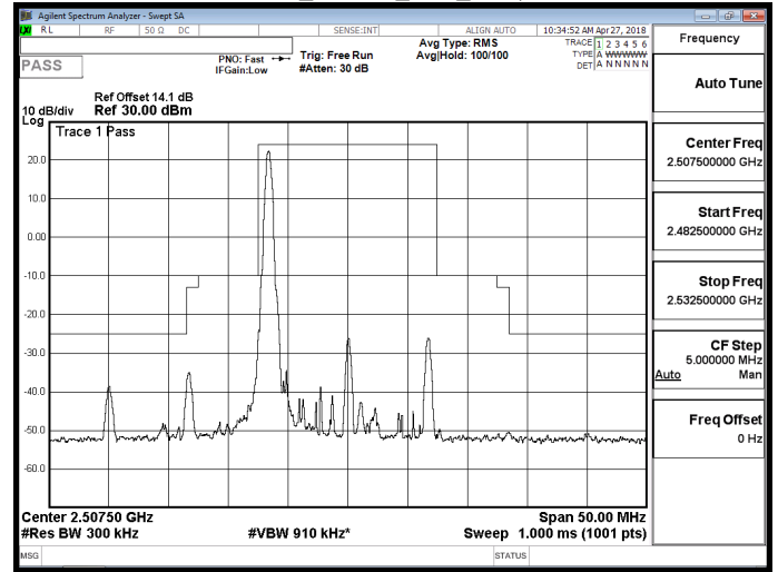
Band 7_16QAM_15M_RB1,74
