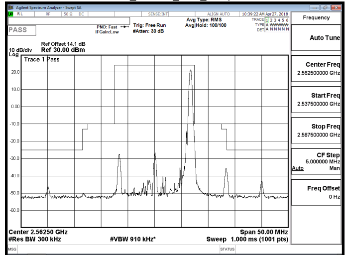
Band 7_16QAM_15M_RB75,0
