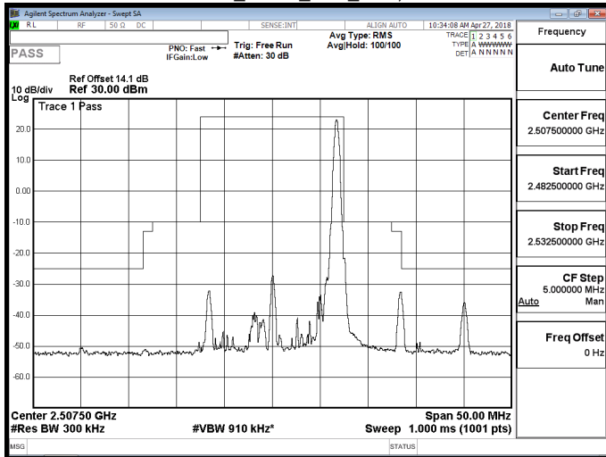
Band 7_QPSK_15M_RB75,0
