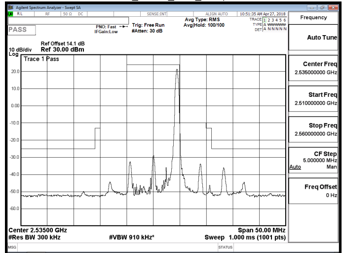
Band 7_QPSK_10M_RB50,0
