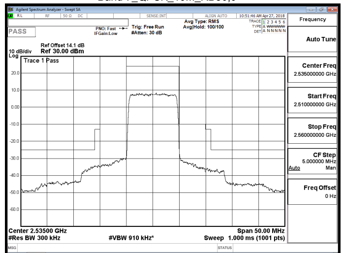
Band 7_QPSK_10M_RB50,0
