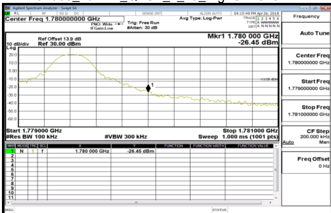
Band66_10MHz_QPSK_1_49_HighCH132622
