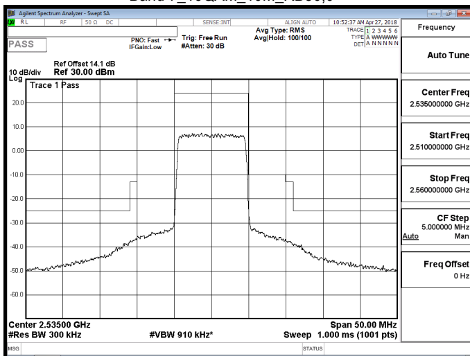
Band 7_16QAM_10M_RB50,0
