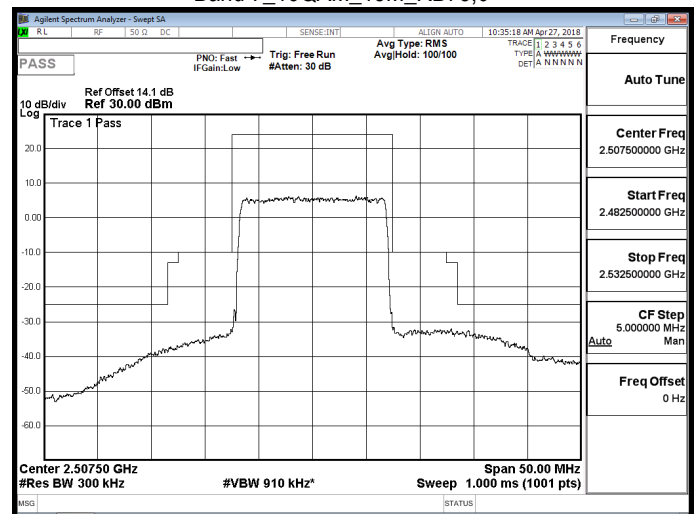
Band 7_16QAM_15M_RB75,0
