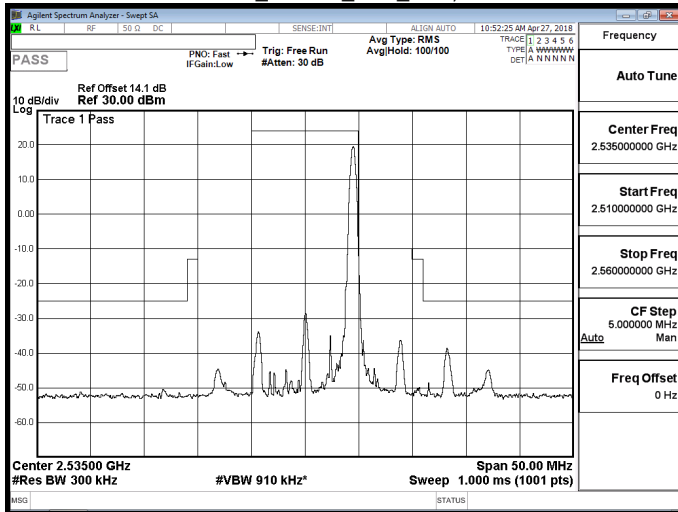
Band 7_16QAM_10M_RB50,0
