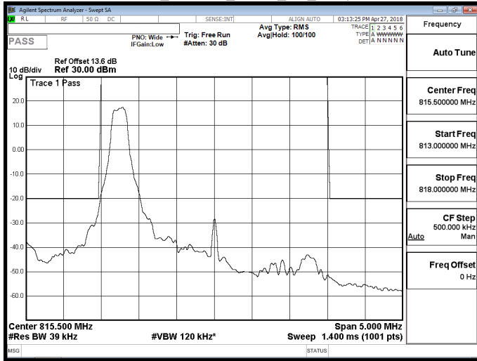
Part 90_Band 26_QPSK_3M_RB1,14
