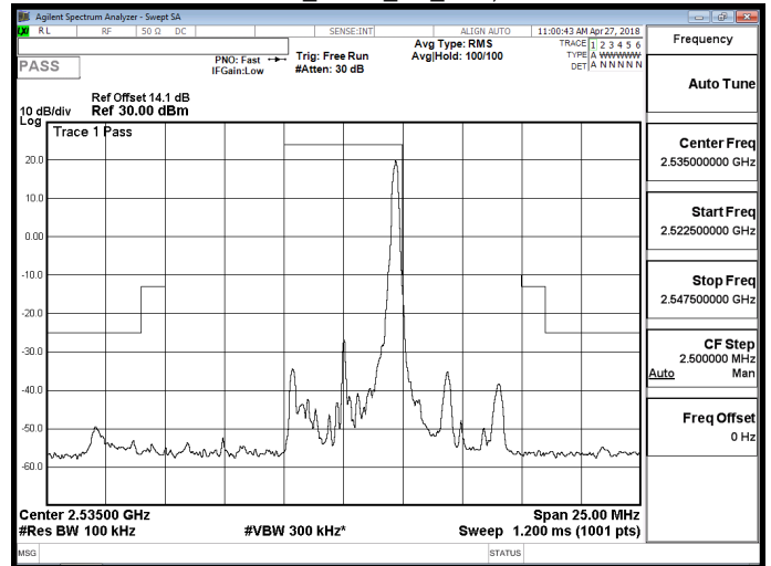
Band 7_QPSK_5M_RB25,0
