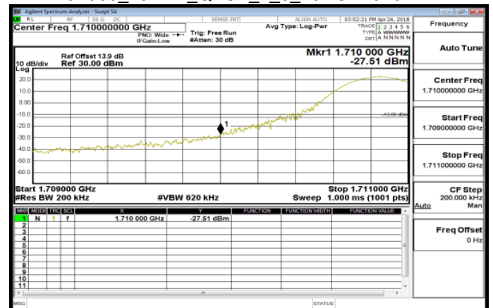
Band66_15MHz_QPSK_1_0_LowCH132047
