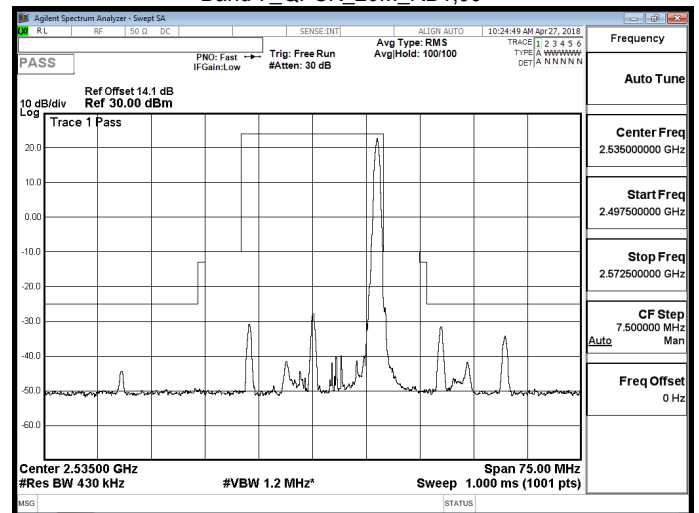
Band 7_QPSK_20M_RB100,0
