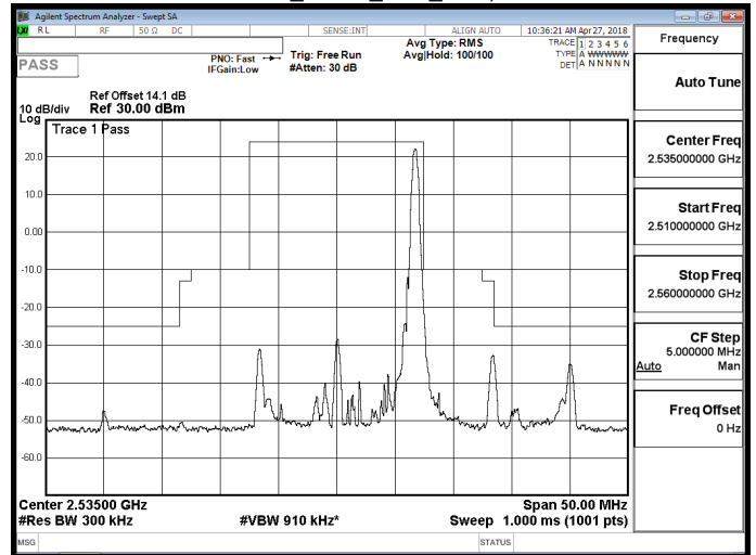
Band 7_QPSK_15M_RB75,0
