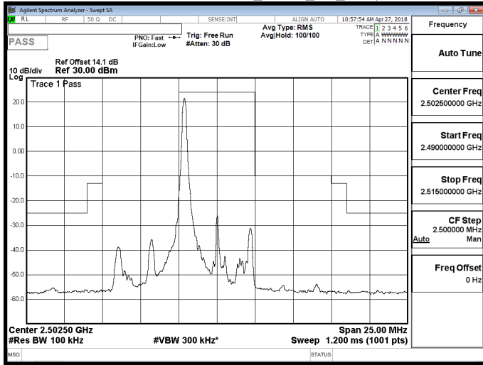
Band 7_QPSK_5M_RB1,24
