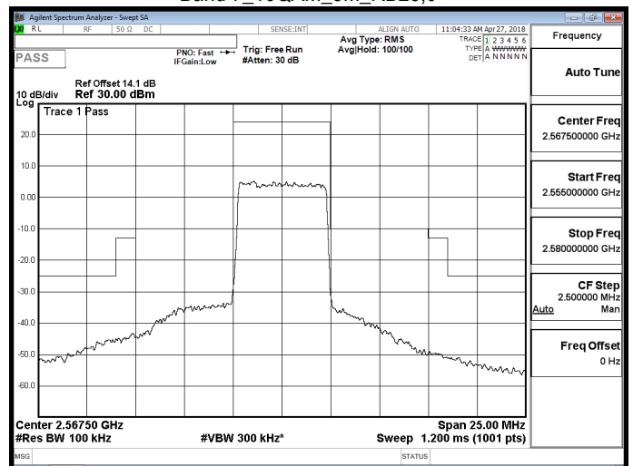
Band 7_16QAM_5M_RB25,0
