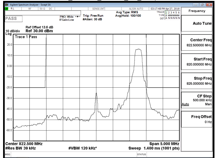
Part 90_Band 26_16QAM_3M_RB15,0
