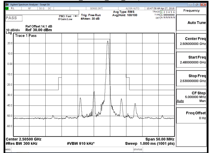
Band 7_16QAM_10M_RB50,0
