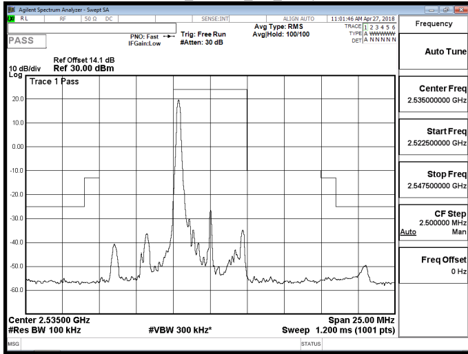
Band 7_16QAM_5M_RB1,24
