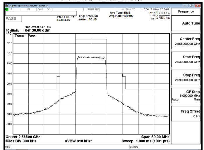
Band 7_16QAM_10M_RB50,0
