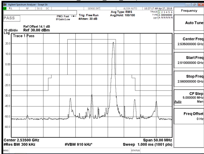
Band 7_16QAM_15M_RB75,0
