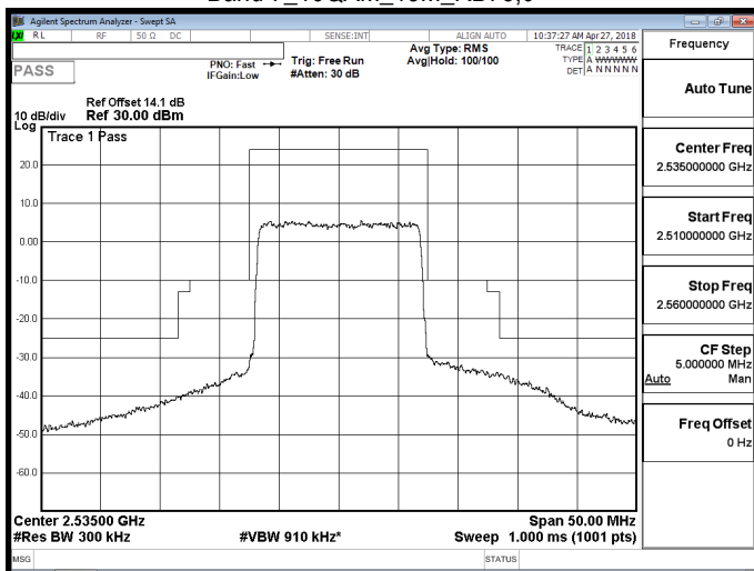
Band 7_16QAM_15M_RB75,0
