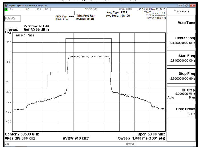
Band 7_QPSK_15M_RB75,0
