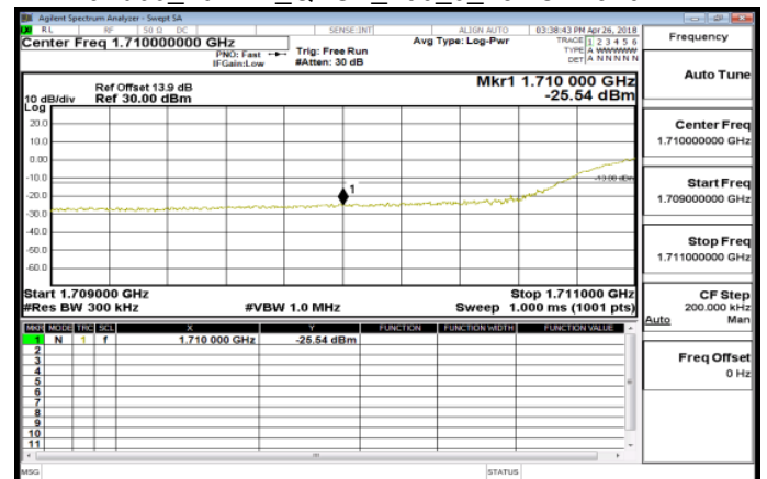
Band66_20MHz_QPSK_100_0_LowCH132072
