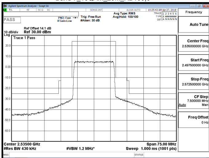
Band 7_16QAM_20M_RB100,0
