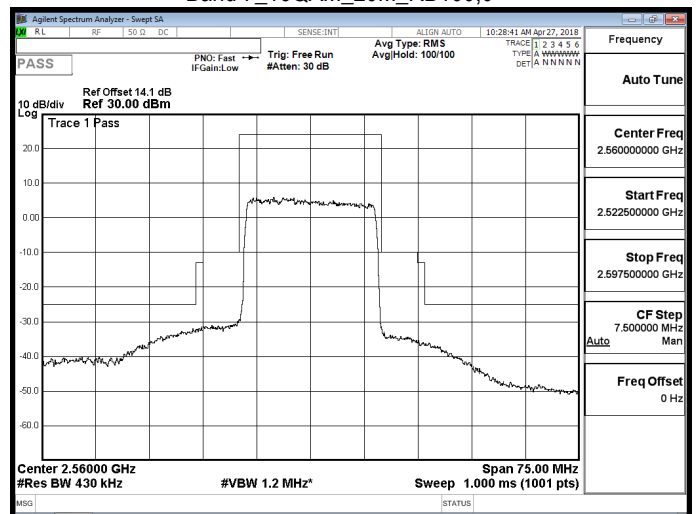
Band 7_16QAM_20M_RB100,0
