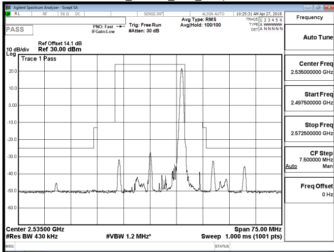
Band 7_16QAM_20M_RB100,0
