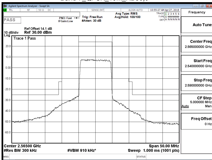
Band 7_QPSK_10M_RB50,0
