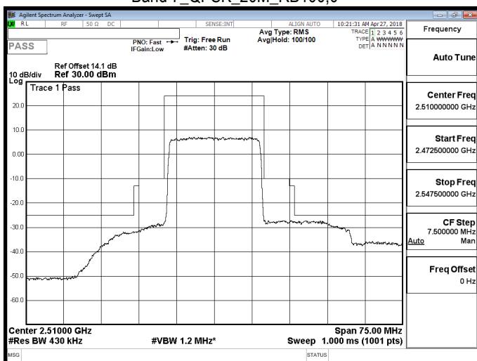
Band 7_QPSK_20M_RB100,0
