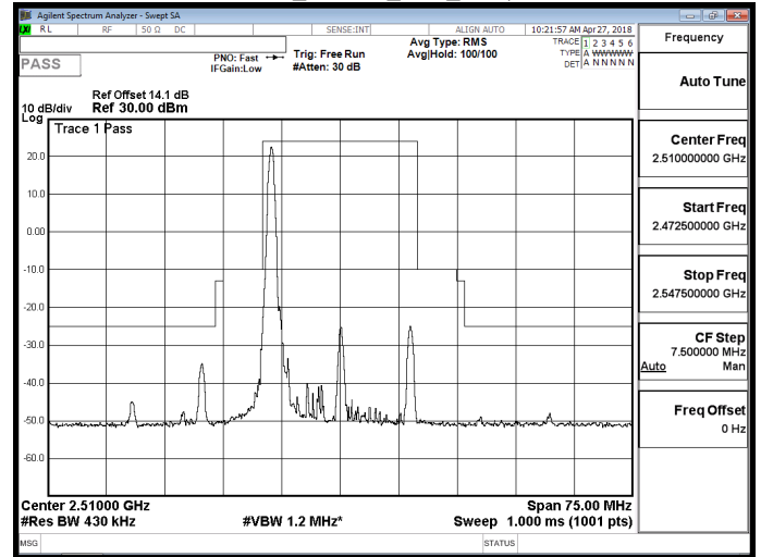
Band 7_16QAM_20M_RB1,99
