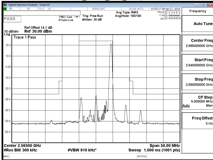
Band 7_QPSK_10M_RB50,0
