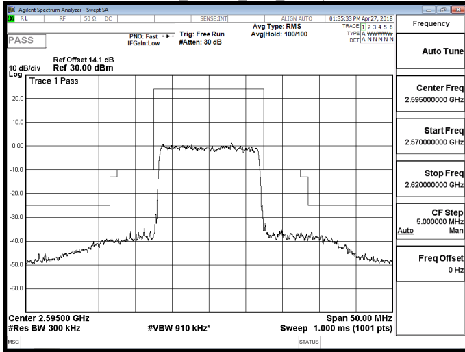
Band 38_16QAM_15M_RB1,0
