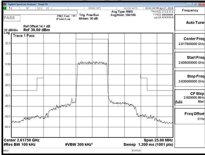
Band 38_16QAM_5M_RB1,0
