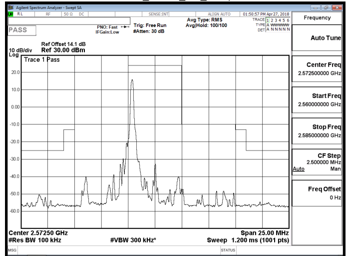
Band 38_QPSK_5M_RB1,24
