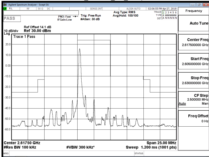
Band 38_16QAM_5M_RB1,24
