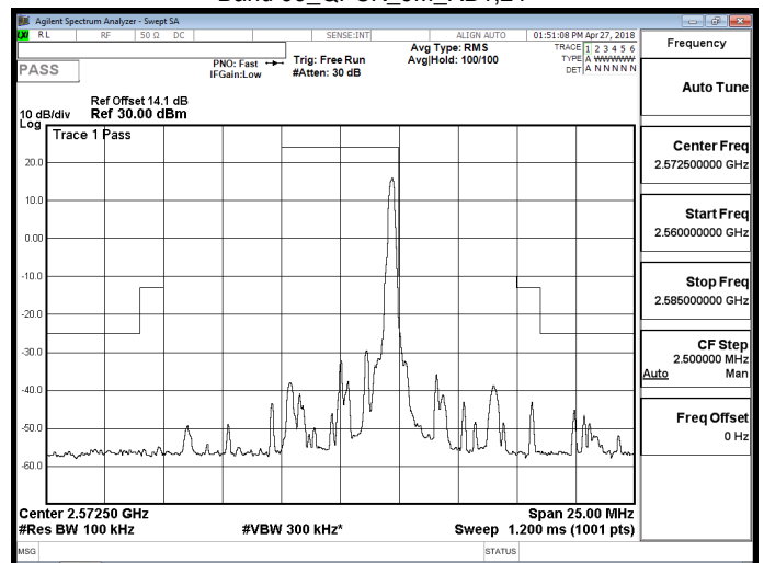
Band 38_QPSK_5M_RB1,24
