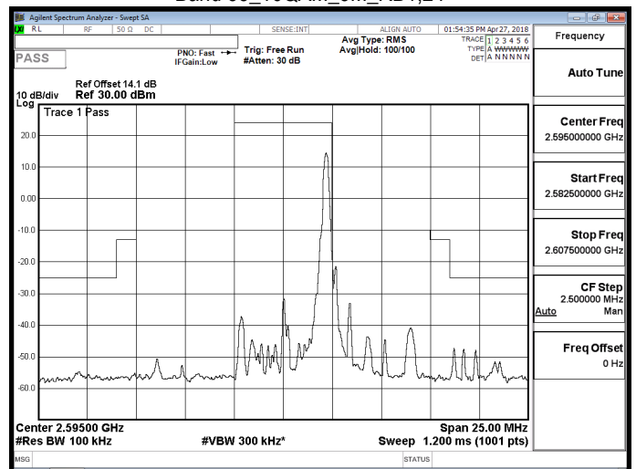
Band 38_16QAM_5M_RB1,24
