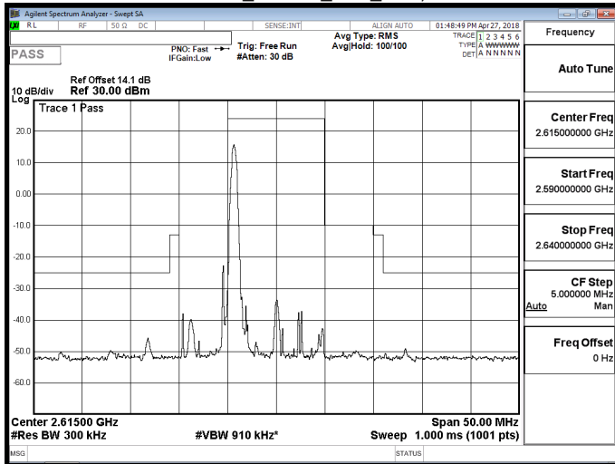
Band 38_16QAM_10M_RB1,49
