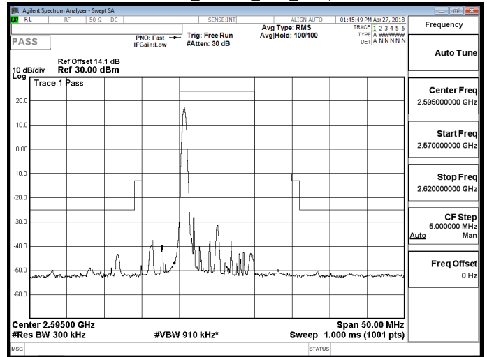
Band 38_16QAM_10M_RB1,49
