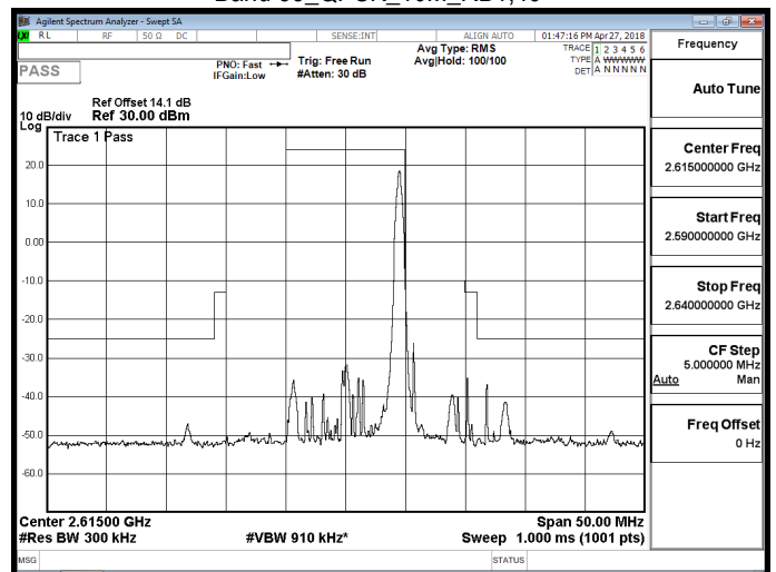
Band 38_QPSK_10M_RB1,49
