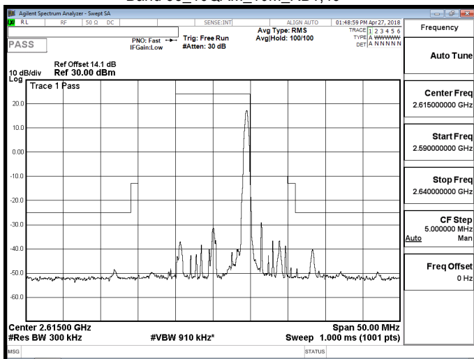
Band 38_16QAM_10M_RB1,49
