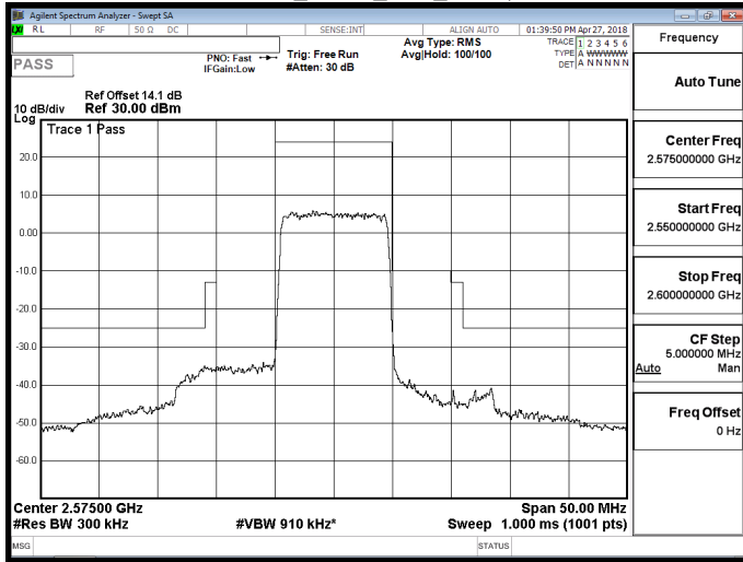
Band 38_QPSK_10M_RB1,0
