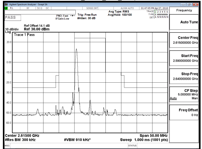
Band 38_QPSK_10M_RB1,49
