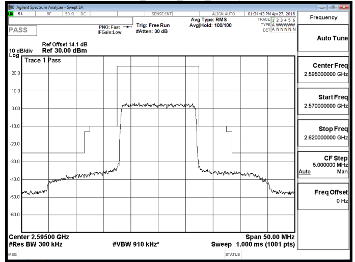
Band 38_QPSK_15M_RB1,0
