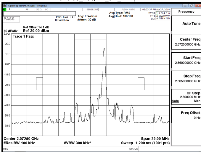
Band 38_16QAM_5M_RB1,24
