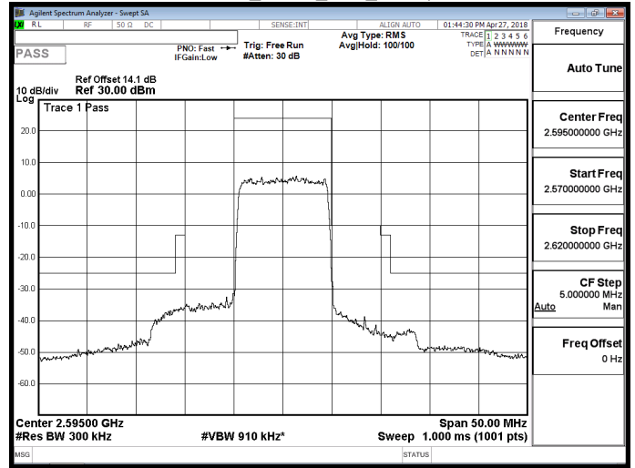
Band 38_QPSK_10M_RB1,0
