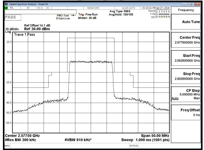
Band 38_16QAM_15M_RB1,0
