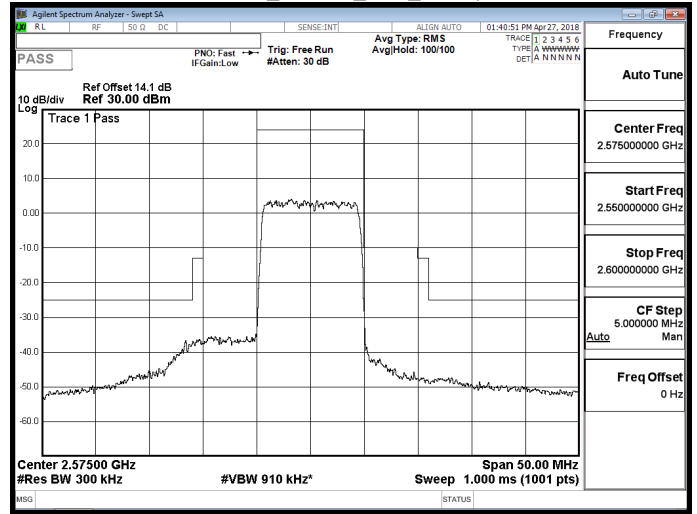
Band 38_16QAM_10M_RB1,0
