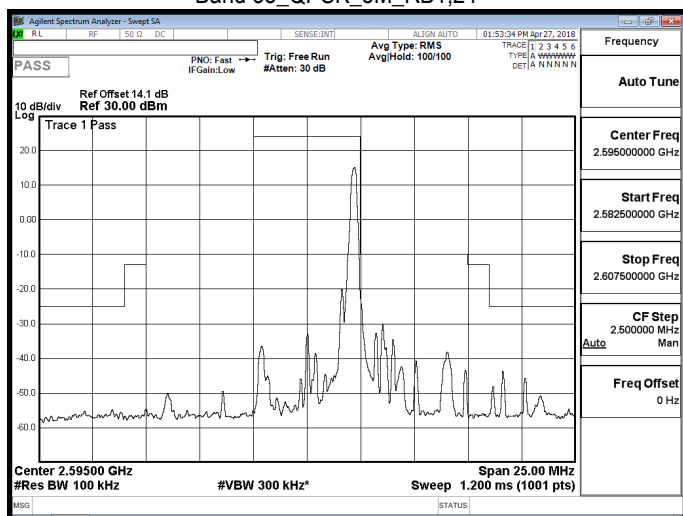
Band 38_QPSK_5M_RB1,24
