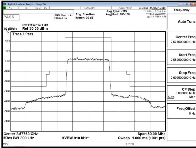
Band 38_QPSK_15M_RB1,0
