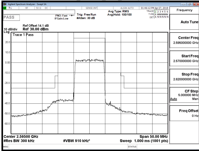
Band 38_16QAM_10M_RB1,0
