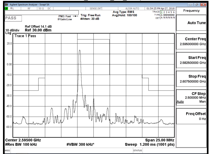
Band 38_16QAM_5M_RB1,24
