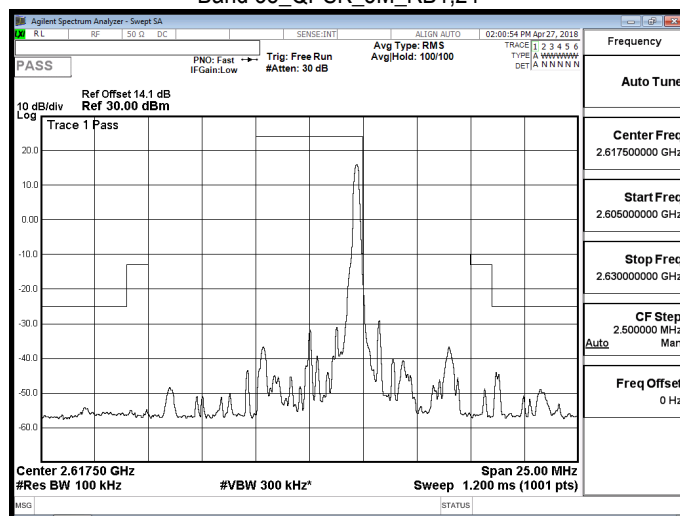
Band 38_QPSK_5M_RB1,24
