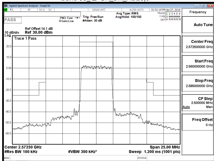
Band 38_QPSK_5M_RB1,0
