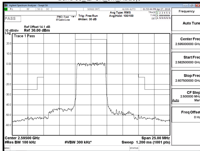
Band 38_QPSK_5M_RB1,0
