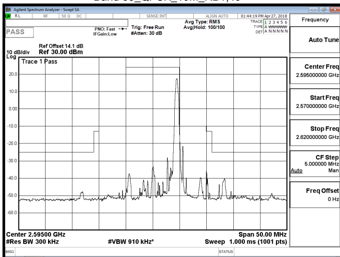
Band 38_QPSK_10M_RB1,49
