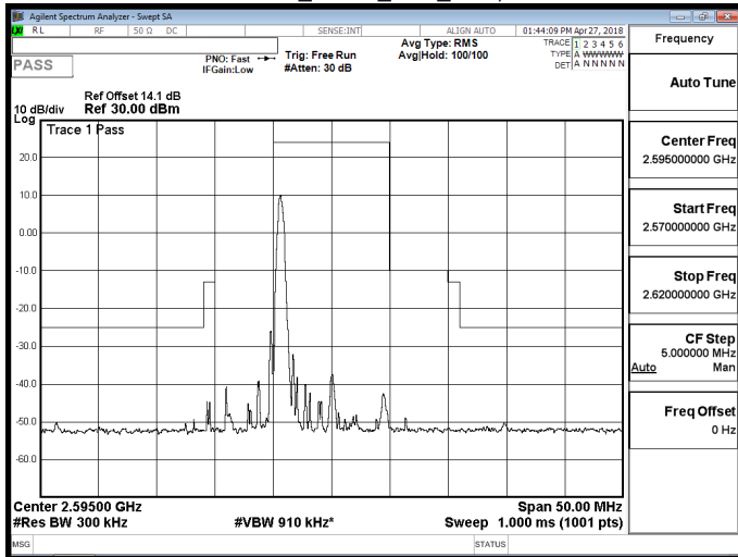
Band 38_QPSK_10M_RB1,49
