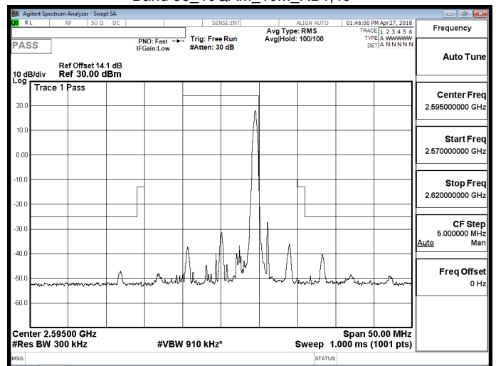
Band 38_16QAM_10M_RB1,49
