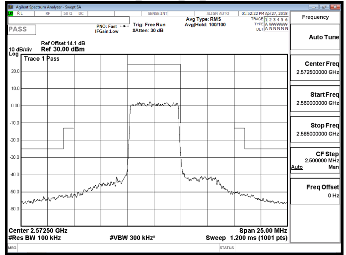
Band 38_16QAM_5M_RB1,0
