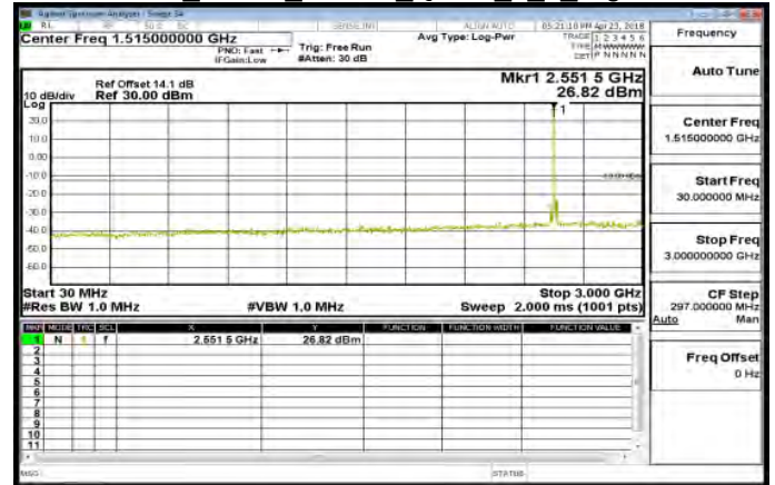
30MHz~3GHz Band7 20MHz QPSK 1 0 HighCH21350
