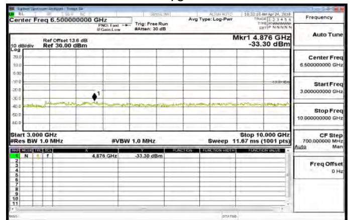
3GHz~10GHz_Band12_1_4MHz_QPSK_1_0_HighCH231 73
