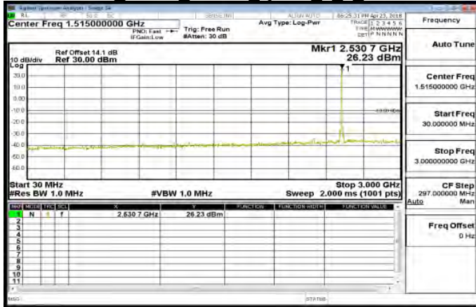
30MHz~3GHz Band7 15MHz QPSK 1 0 MidCH21100
