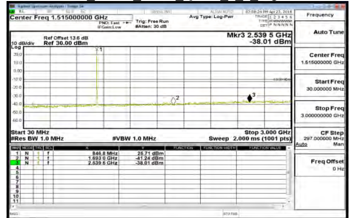
30MHz~3GHz Band5 5MHz QPSK 1 0 HighCH20625
