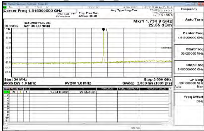
30MHz~3GHz WCDMA B4 MidCH1413-1732.6
