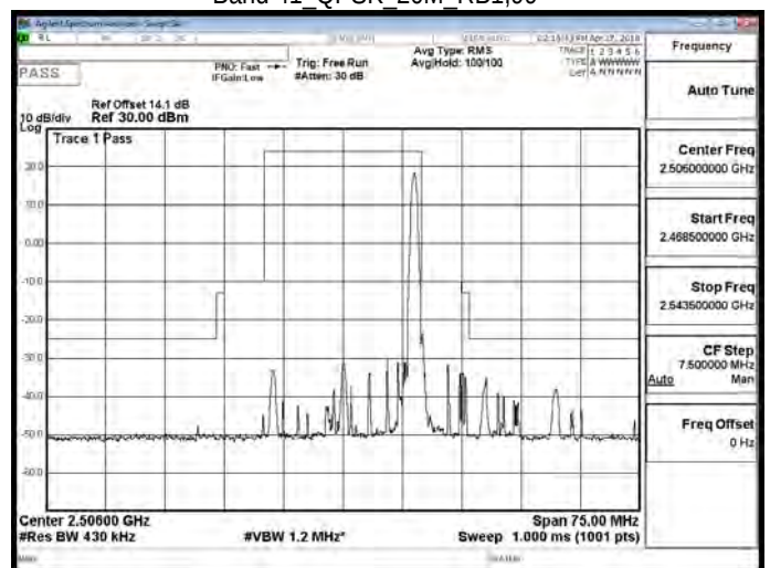
Band 41 QPSK 20M RB1,99
