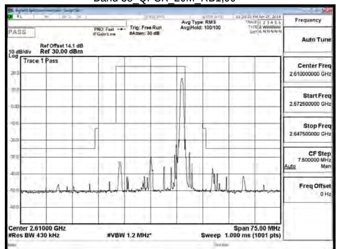
Band 38 QPSK 20M RB1,99
