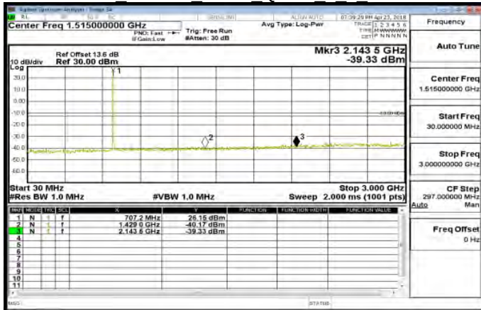
30MHz~3GHz Band12 3MHz QPSK 1 0 MidCH23095
