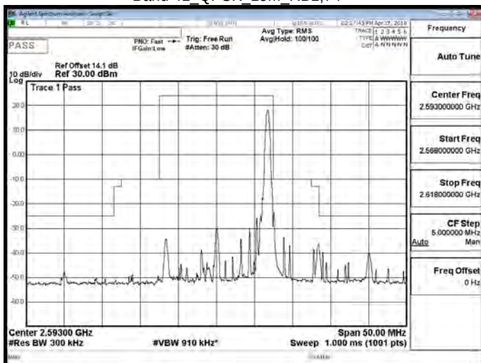
Band 41 QPSK 15M RB1,74
