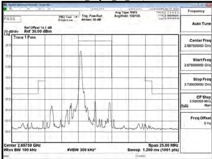
Band 41 16QAM 5M RB1,24
