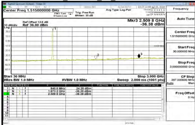
30MHz~3GHz WCDMA B5 MidCH4183-836.6
