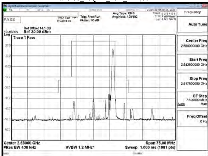
Band 38 16QAM 20M RB1,99
