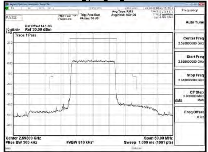
Band 41 QPSK 15M RB1,0
