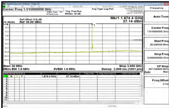
30MHz~3GHz_Band2_15MHz_QPSK_1_0_MidCH18900-1880
