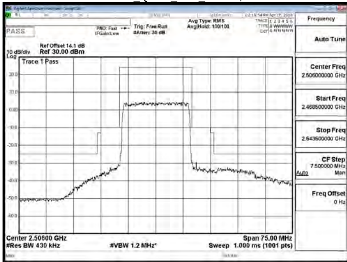
Band 41 QPSK 20M RB1,0
