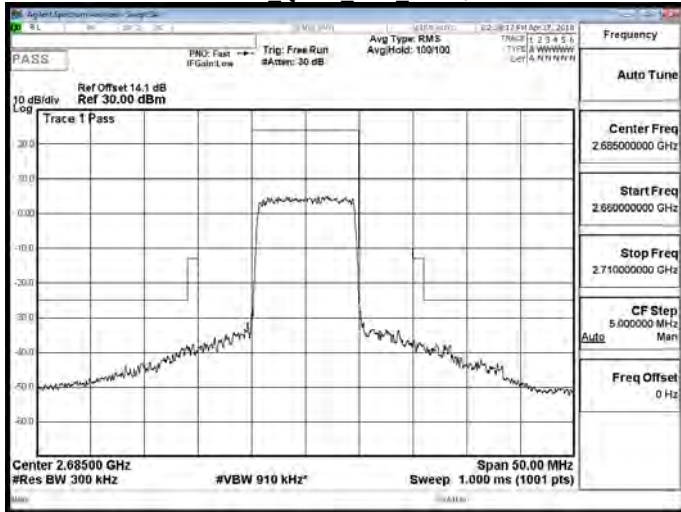
Band 41 16QAM 10M RB1,0
