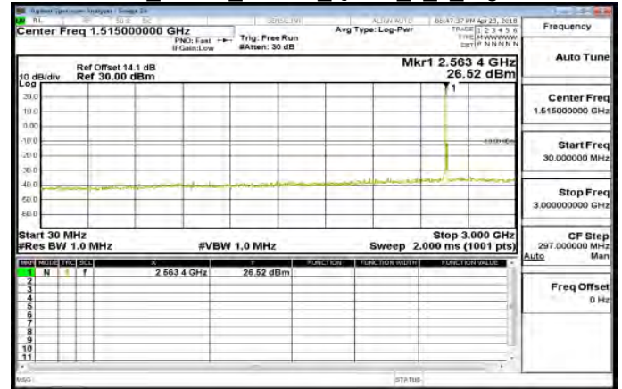
30MHz~3GHz Band7 10MHz QPSK 1 0 HighCH21400
