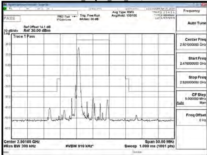
Band 41 16QAM 10M RB1,49
