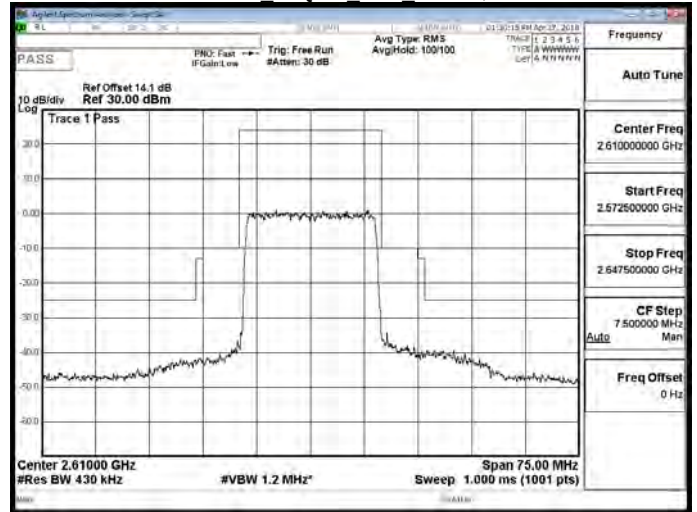
Band 41 QPSK 5M RB1,0
