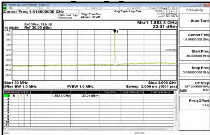
30MHz~3GHz HSDPA B2 MidCH9400-1880
