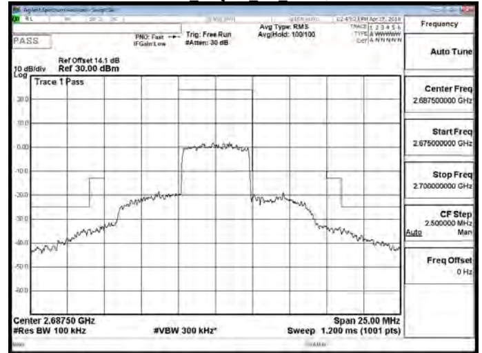
Band 41 QPSK 10M RB1,0
