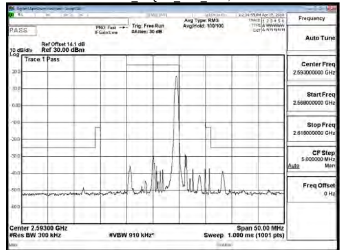
Band 41 16QAM 10M RB1,49
