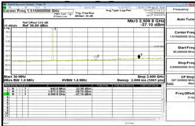
30MHz~3GHz HSDPA B5 MidCH4183-836.6
