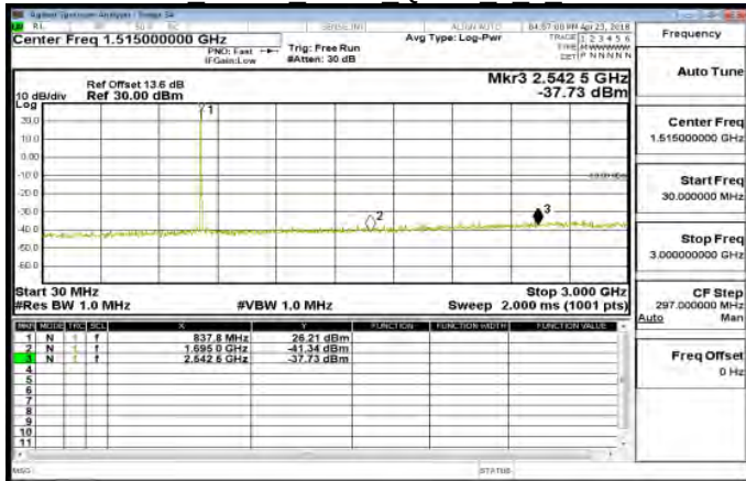
30MHz~3GHz Band5 3MHz QPSK 1 0 MidCH20525
