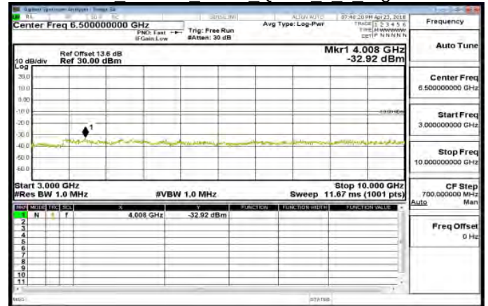
3GHz~10GHz Band12 3MHz QPSK 1 0 HighCH23165
