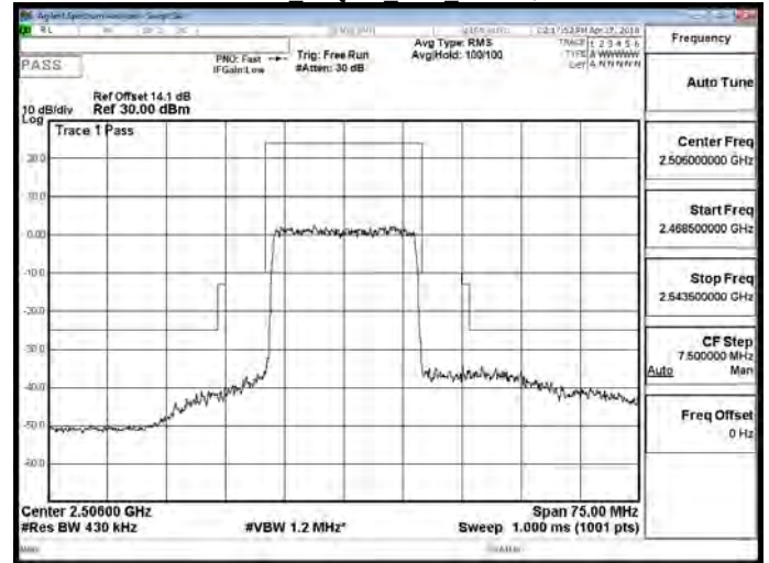
Band 41 16QAM 20M RB1,0
