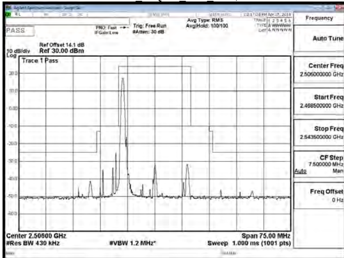
Band 41 16QAM 20M RB1,99
