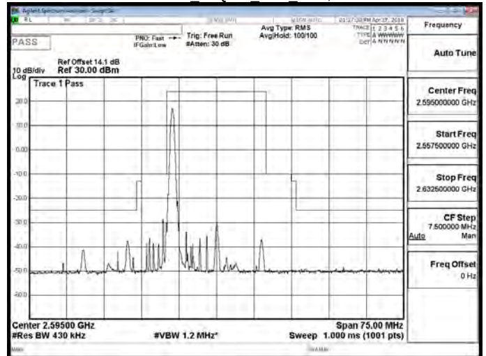
Band 38 16QAM 20M RB1,99
