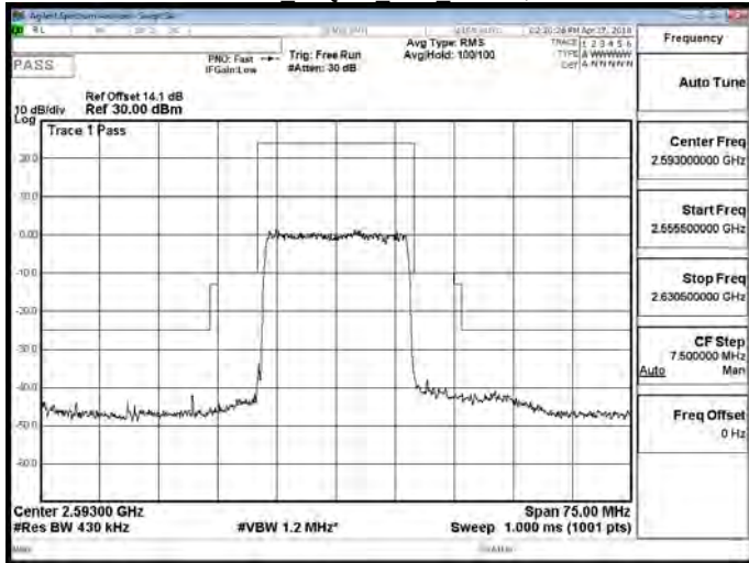
Band 41 16QAM 20M RB1,0
