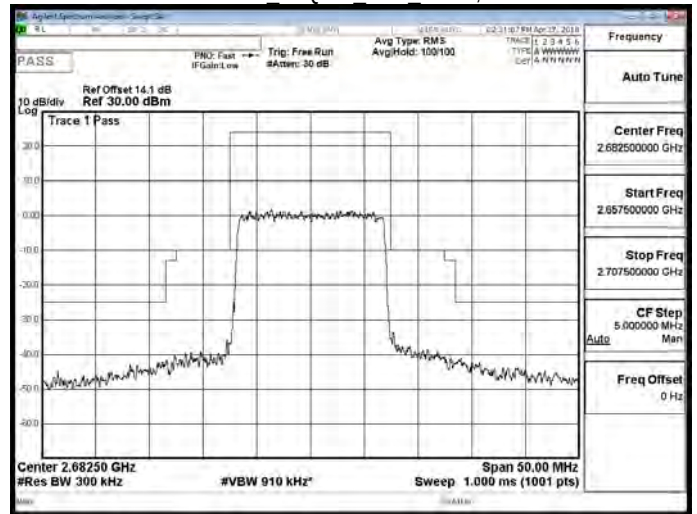
Band 41 QPSK 20M RB1,0
