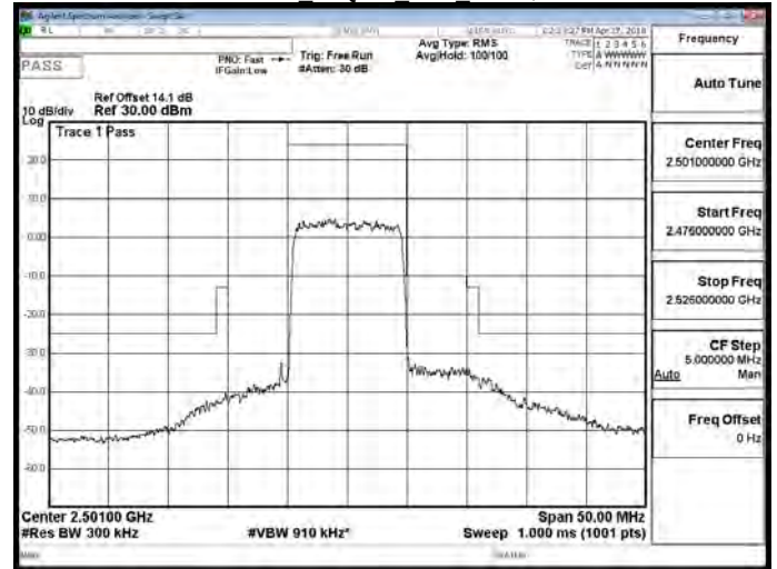
Band 41 16QAM 10M RB1,0
