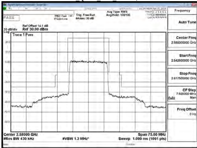
Band 38 QPSK 20M RB1,0
