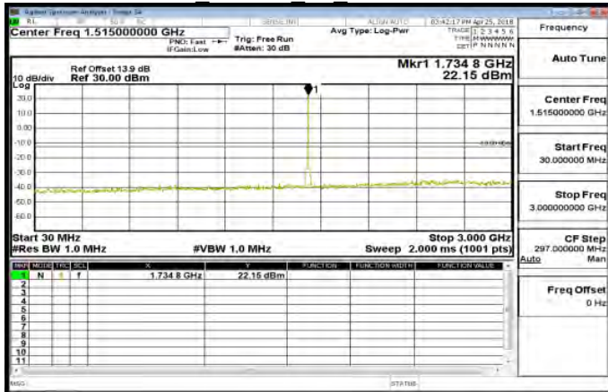
30MHz~3GHz HSDPA B4 MidCH1413-1732.6
