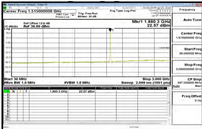
30MHz~3GHz HSUPA B2 MidCH9400-1880
