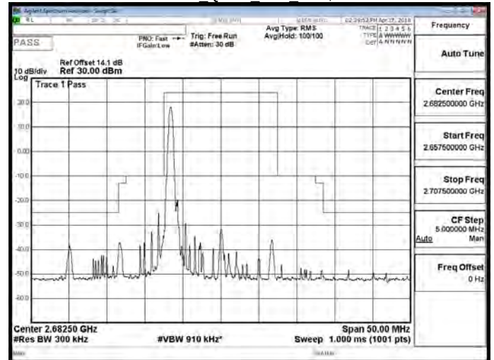
Band 41 QPSK 15M RB1,74
