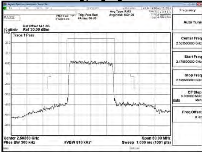
Band 41 QPSK 15M RB1,0
