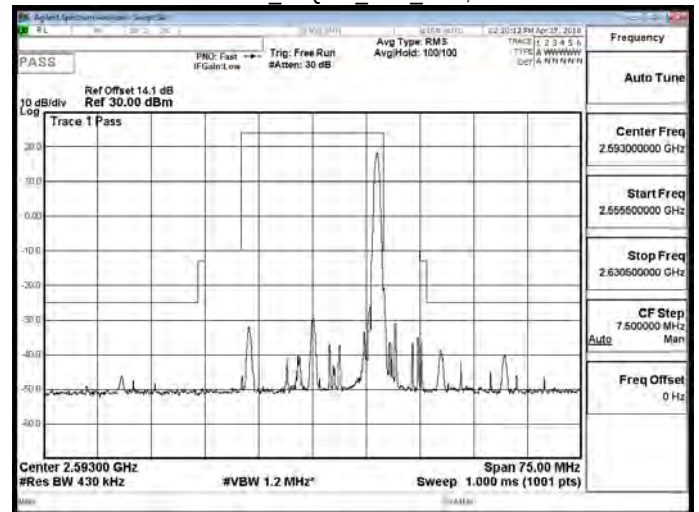
Band 41 16QAM 20M RB1,99
