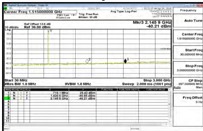
30MHz~3GHz_Band12_1_4MHz_QPSK_1_0_MidCH2309 5
