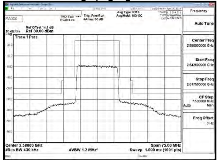
Band 38 16QAM 20M RB1,0
