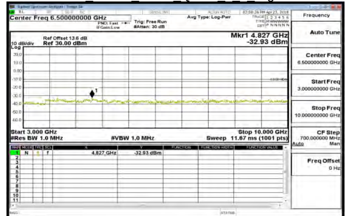
3GHz~10GHz Band5 5MHz QPSK 1 0 HighCH20625
