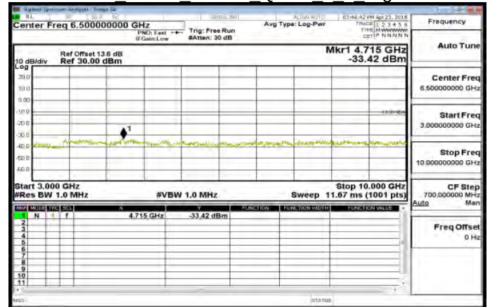
3GHz~10GHz Band5 10MHz QPSK 1 0 HighCH20600
