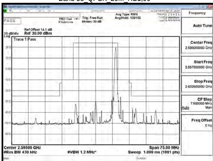
Band 38 QPSK 20M RB1,99
