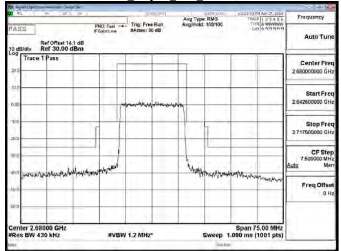
Band 41 16QAM 20M RB100,0
