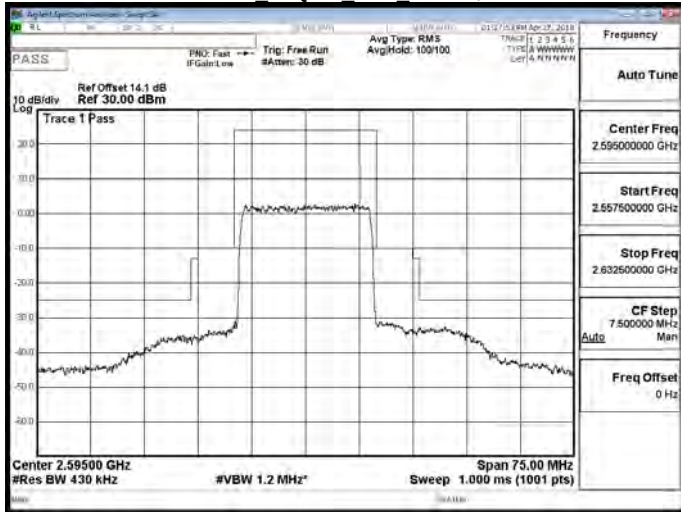
Band 38 16QAM 20M RB1,0
