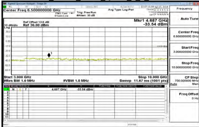
3GHz~10GHz Band5 5MHz QPSK 1 0 LowCH20425
