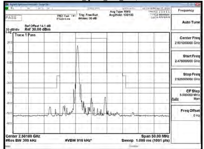
Band 41 QPSK 10M RB1,49
