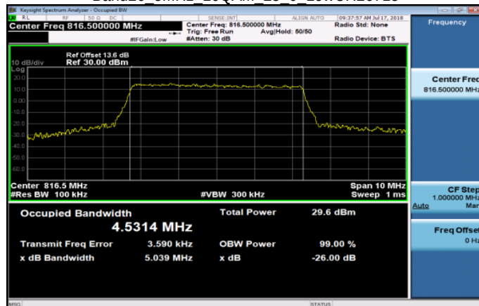
Band26 5MHz 16QAM 25 0 LowCH26715
