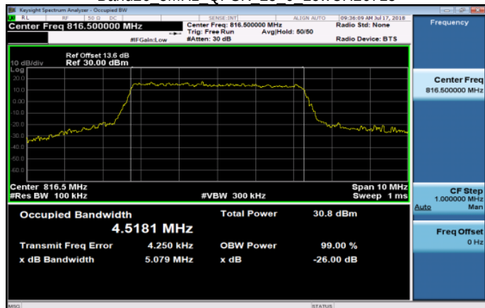
Band26 5MHz QPSK 25 0 LowCH26715
