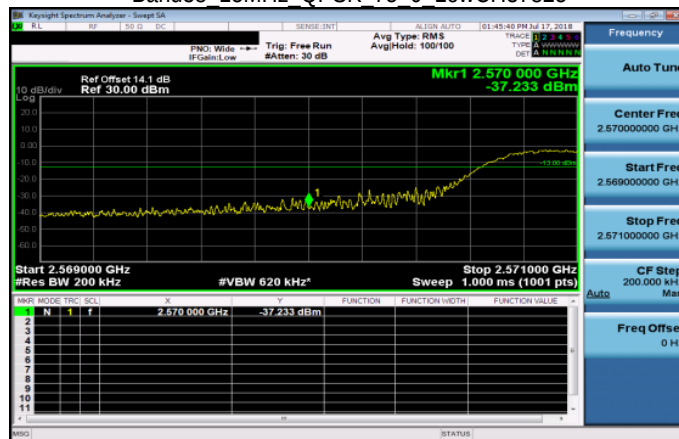
Band38 15MHz QPSK 75 0 LowCH37825
