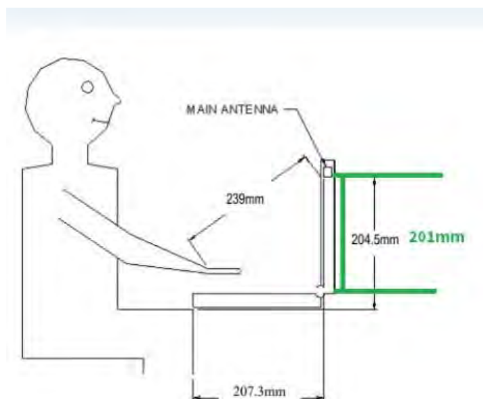
Fig.10 Antenna location of EUT (tablet mode)
