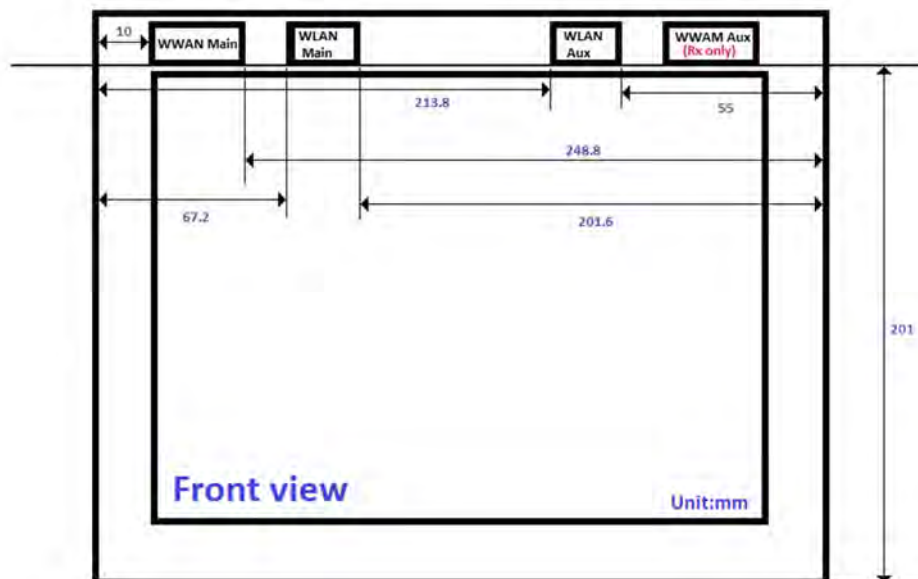
Fig.10 Antenna location of EUT (tablet mode)
