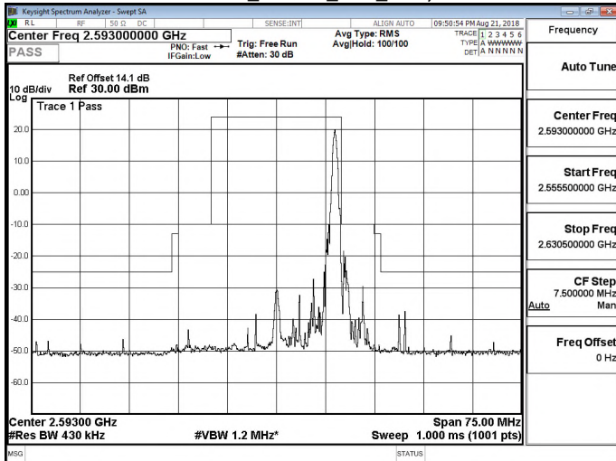
Band 41_16QAM_20M_RB100,0
