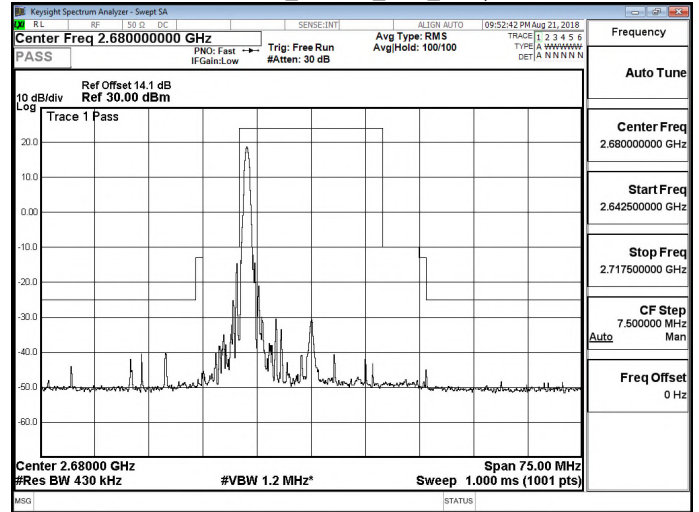
Band 41_16QAM_20M_RB1,99
