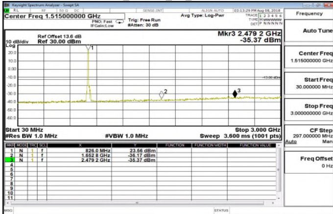
30MHz~3GHz_HSDPA_B5_LowCH4132-826.4
