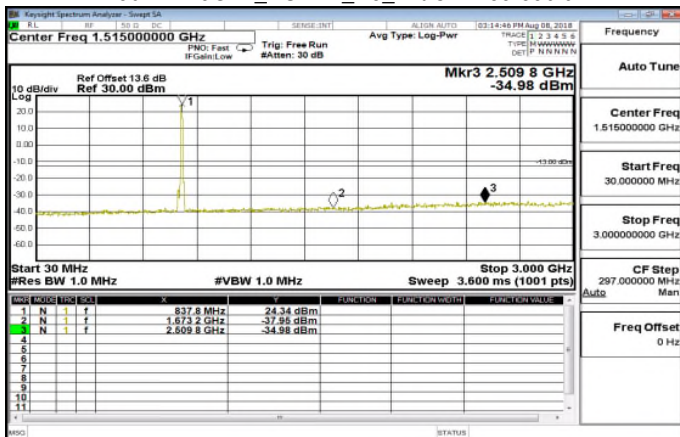
30MHz~3GHz_HSDPA_B5_MidCH4183-836.6
