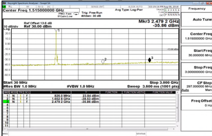
30MHz~3GHz_HSUPA_B5_LowCH4132-826.4
