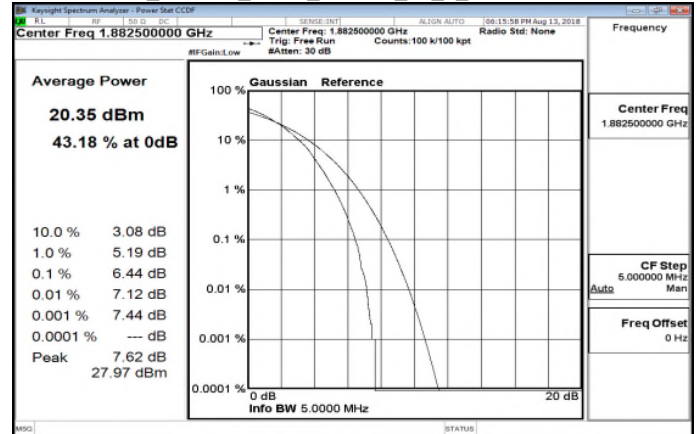
LTE_Band25_5MHz_16QAM_25_0_MidCH26365
