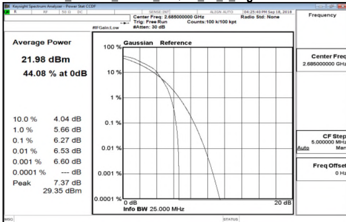
LTE_Band41_10MHz_16QAM_50_0_HighCH41540
