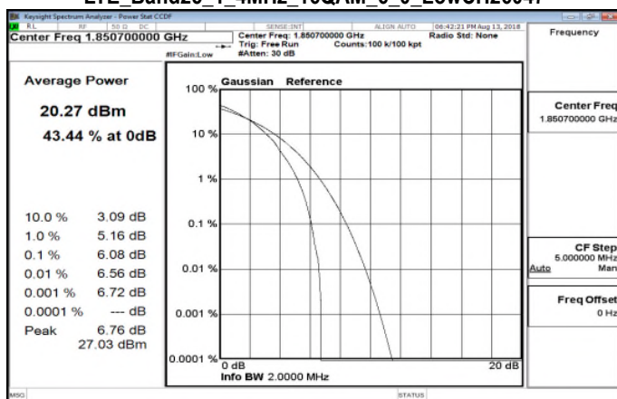
LTE_Band25_1_4MHz_16QAM_6_0_LowCH26047
