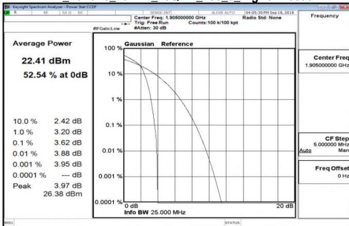
LTE_Band25_20MHz_16QAM_100_0_HighCH26590
