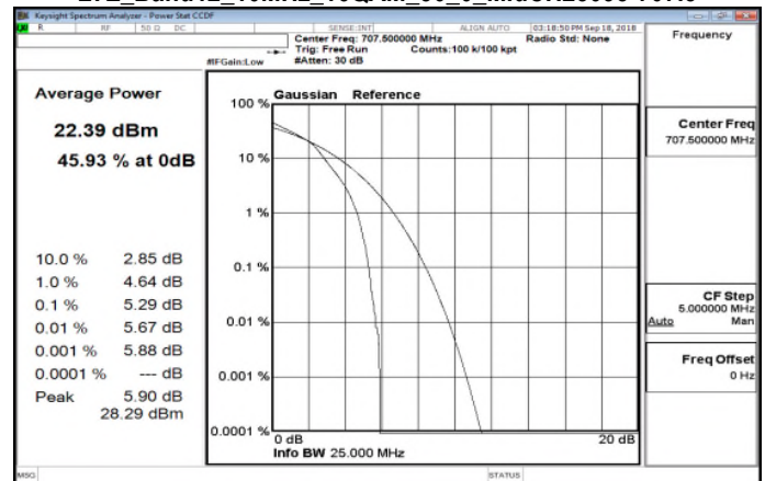
LTE_Band12_10MHz_16QAM_50_0_MidCH23095-707.5
