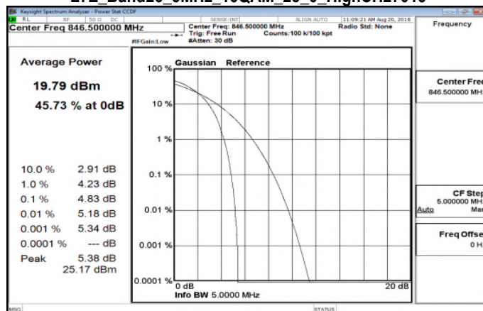
LTE_Band26_5MHz_16QAM_25_0_HighCH27015
