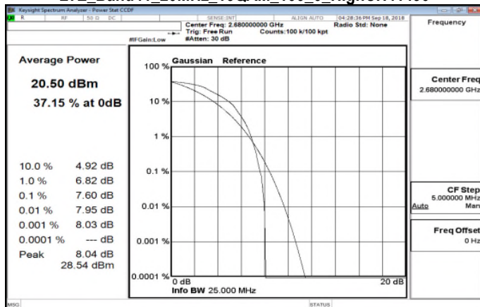
LTE_Band41_20MHz_16QAM_100_0_HighCH41490
