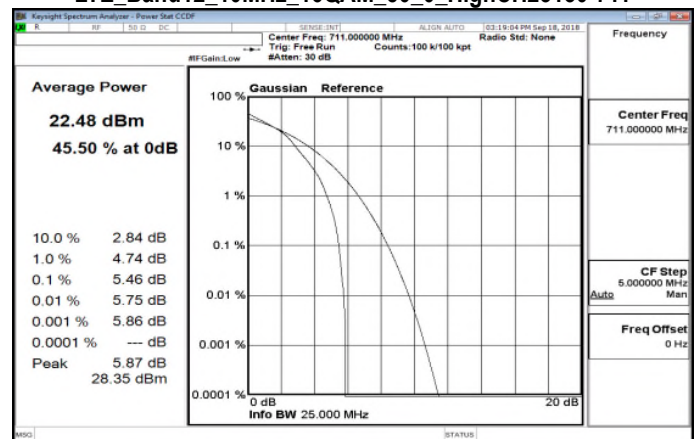
LTE_Band12_10MHz_16QAM_50_0_HighCH23130-711
