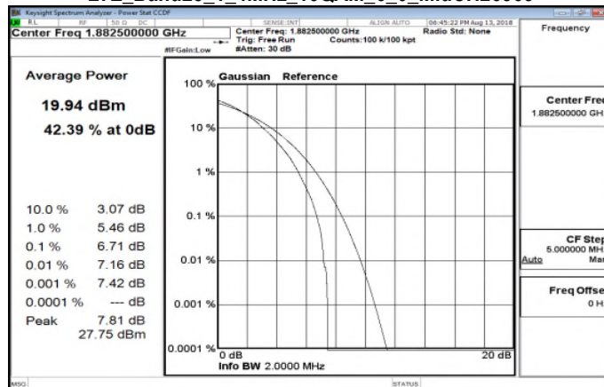
LTE_Band25_1_4MHz_16QAM_6_0_MidCH26365
