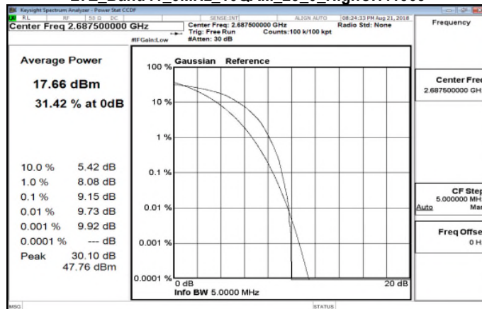
LTE_Band41_5MHz_16QAM_25_0_HighCH41565
