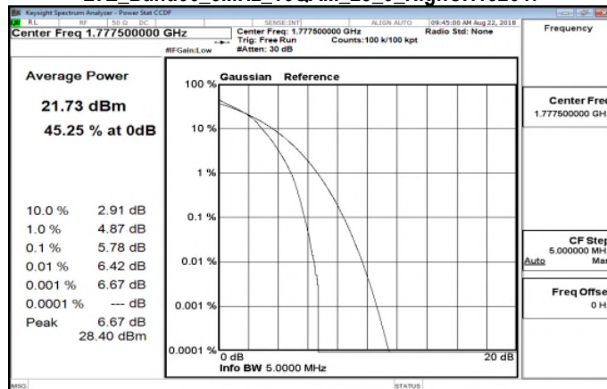
LTE_Band66_5MHz_16QAM_25_0_HighCH132647
