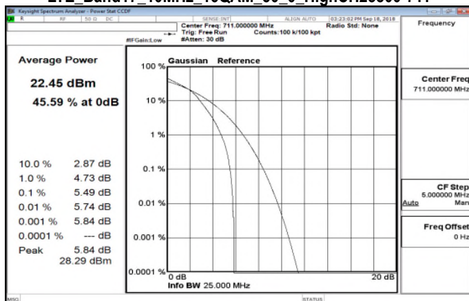
LTE_Band17_10MHz_16QAM_50_0_HighCH23800-711
