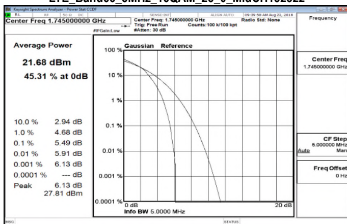
LTE_Band66_5MHz_16QAM_25_0_MidCH132322
