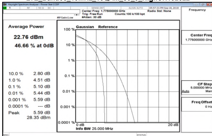
LTE_Band66_10MHz_16QAM_50_0_HighCH132622
