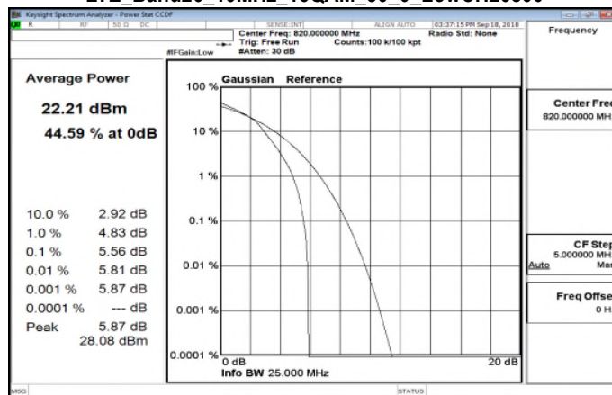
LTE_Band26_10MHz_16QAM_50_0_LowCH26800
