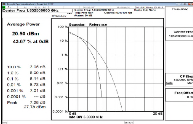
LTE_Band25_5MHz_16QAM_25_0_LowCH26065
