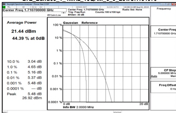
LTE_Band66_1_4MHz_16QAM_6_0_LowCH131979
