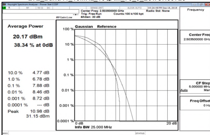
LTE_Band41_15MHz_16QAM_75_0_LowCH39725
