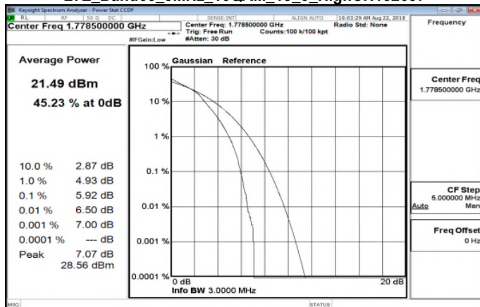
LTE_Band66_3MHz_16QAM_15_0_HighCH132657
