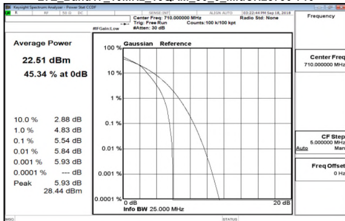
LTE_Band17_10MHz_16QAM_50_0_MidCH23790-710
