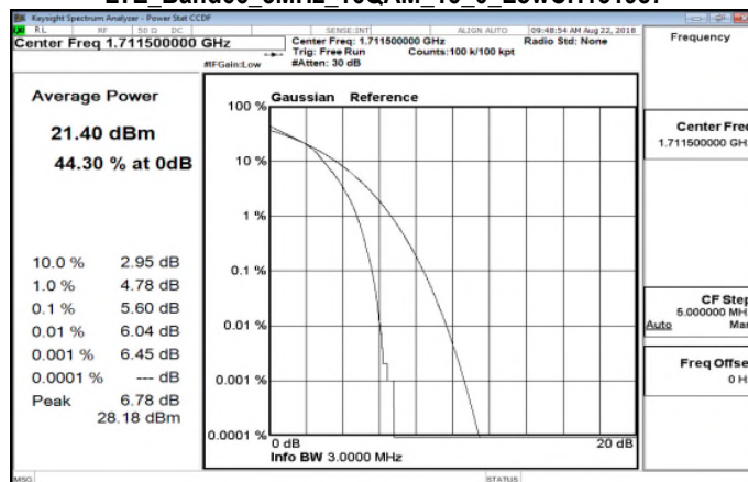
LTE_Band66_3MHz_16QAM_15_0_LowCH131987
