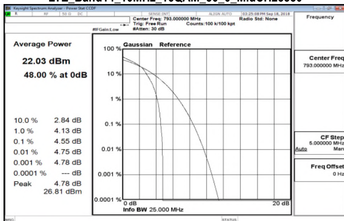
LTE_Band14 10MHz_16QAM_50_0_MidCH23330
