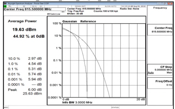
LTE_Band26_3MHz_16QAM_15_0_LowCH26705
