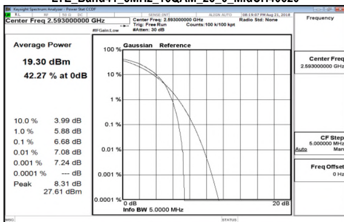
LTE_Band41_5MHz_16QAM_25_0_MidCH40620
