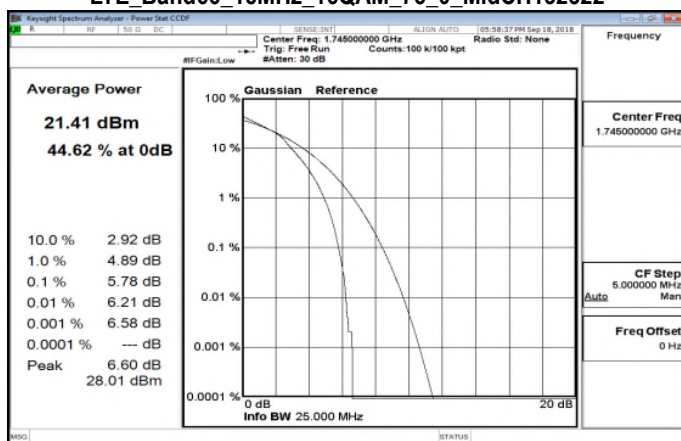
LTE_Band66_15MHz_16QAM_75_0_MidCH132322
