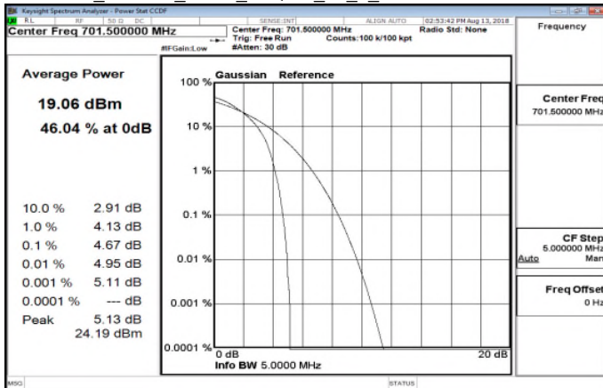
LTE_Band12_5MHz_16QAM_25_0_LowCH23035-701.5
