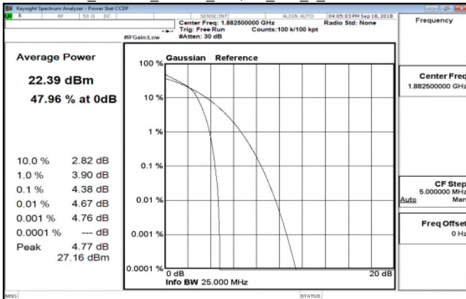
LTE_Band25_20MHz_16QAM_100_0_MidCH26365
