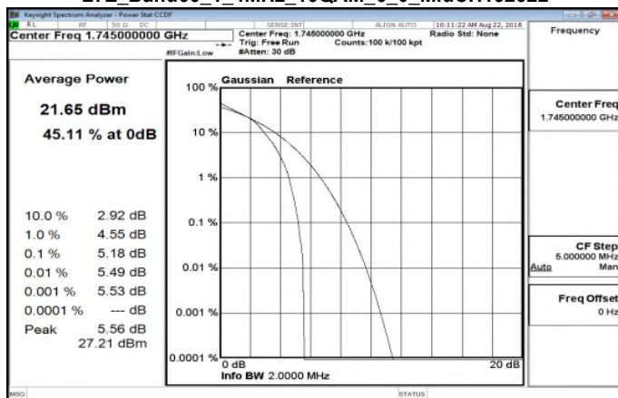
LTE_Band66_1_4MHz_16QAM_6_0_MidCH132322
