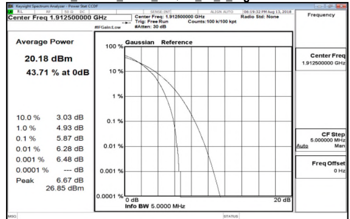
LTE_Band25_5MHz_16QAM_25_0_HighCH26665
