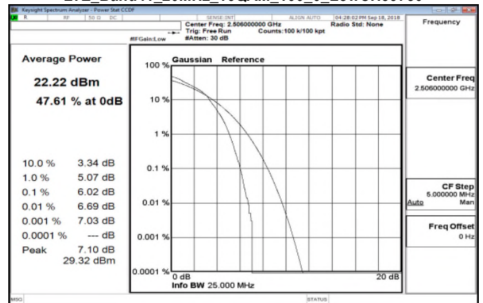
LTE_Band41_20MHz_16QAM_100_0_LowCH39750
