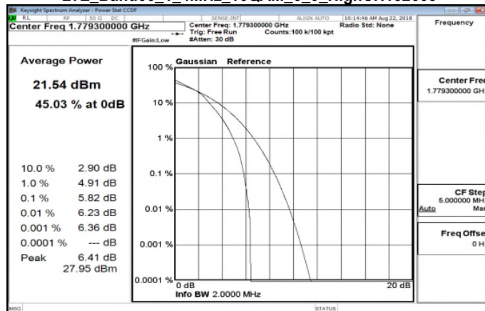
LTE_Band66_1_4MHz_16QAM_6_0_HighCH132665
