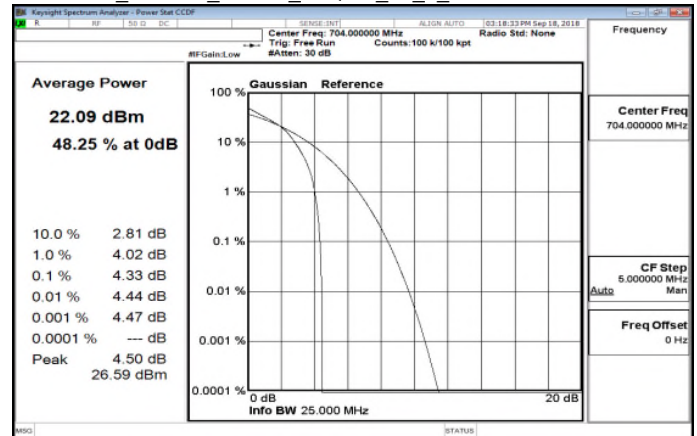
LTE_Band12_10MHz_16QAM_50_0_LowCH23060-704
