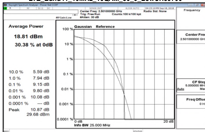
LTE_Band41_10MHz_16QAM_50_0_LowCH39700
