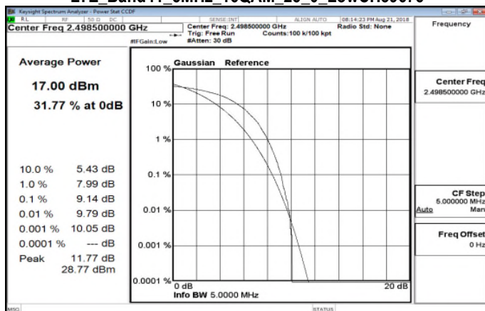
LTE_Band41_5MHz_16QAM_25_0_LowCH39675
