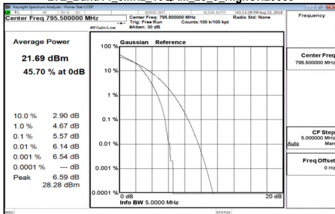
LTE_Band14 5MHz_16QAM_25_0_HighCH23355
