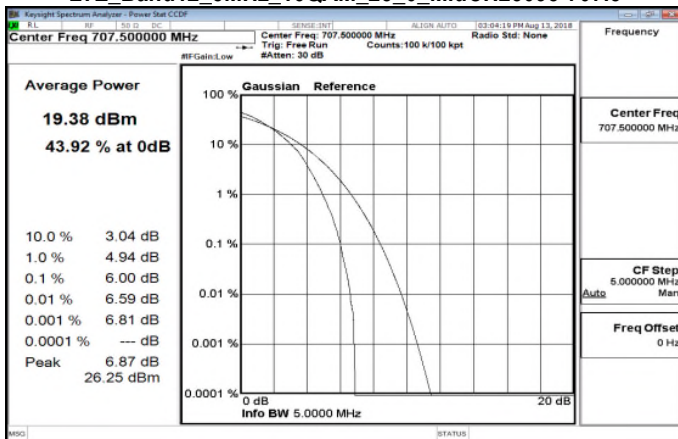
LTE_Band12_5MHz_16QAM_25_0_MidCH23095-707.5
