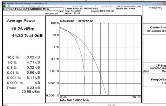
LTE_Band26_5MHz_16QAM_25_0_MidCH26865
