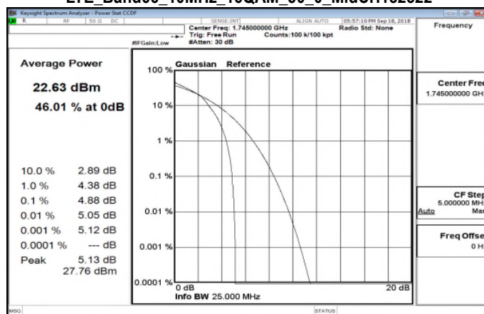
LTE_Band66_10MHz_16QAM_50_0_MidCH132322
