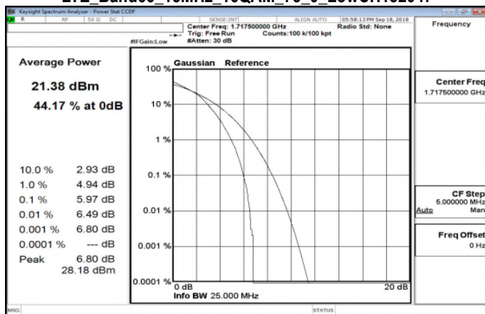
LTE_Band66_15MHz_16QAM_75_0_LowCH132047
