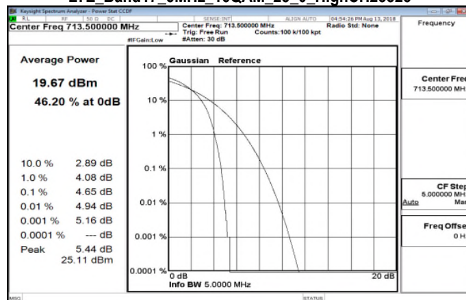
LTE_Band17 5MHz_16QAM_25_0_HighCH23825
