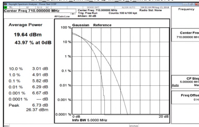
LTE_Band17 5MHz_16QAM_25_0_MidCH23790
