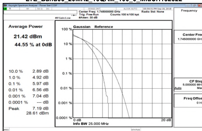
LTE_Band66_20MHz_16QAM_100_0_MidCH132322
