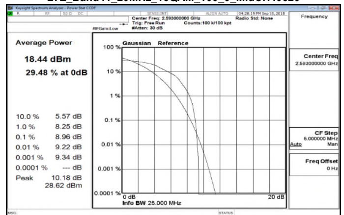
LTE_Band41_20MHz_16QAM_100_0_MidCH40620
