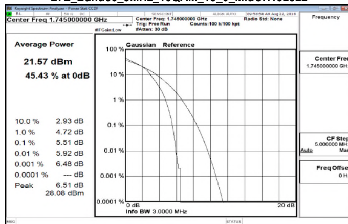
LTE_Band66_3MHz_16QAM_15_0_MidCH132322
