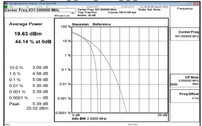
LTE_Band26_1_4MHz_16QAM_6_0_MidCH26865
