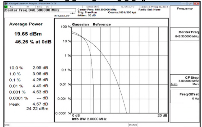
LTE_Band26_1_4MHz_16QAM_6_0_HighCH27033
