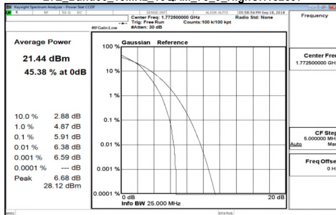
LTE_Band66_15MHz_16QAM_75_0_HighCH132597
