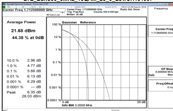
LTE_Band66_5MHz_16QAM_25_0_LowCH131997
