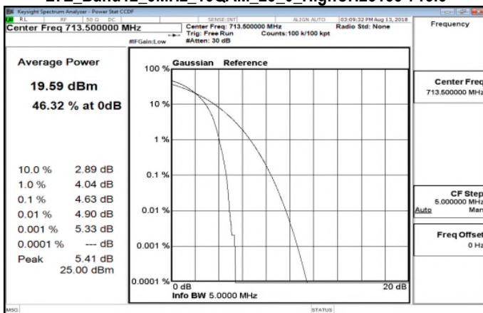
LTE_Band12_5MHz_16QAM_25_0_HighCH23155-713.5
