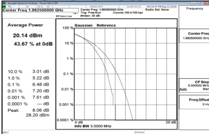
LTE_Band25_3MHz_16QAM_15_0_MidCH26365
