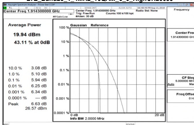
LTE_Band25_1_4MHz_16QAM_6_0_HighCH26683
