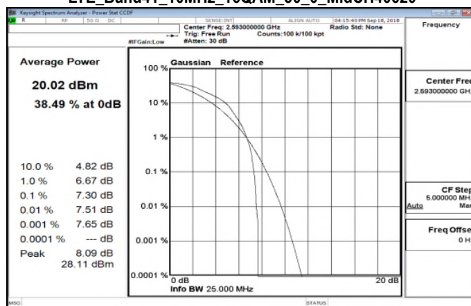
LTE_Band41_10MHz_16QAM_50_0_MidCH40620
