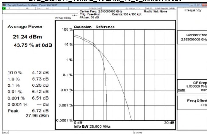
LTE_Band41_15MHz_16QAM_75_0_MidCH40620
