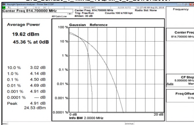
LTE_Band26_1_4MHz_16QAM_6_0_LowCH26697
