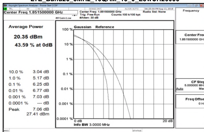
LTE_Band25_3MHz_16QAM_15_0_LowCH26055
