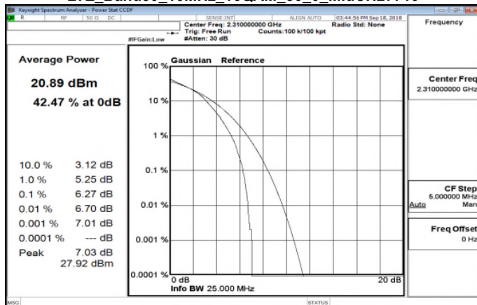
LTE_Band30_10MHz_16QAM_50_0_MidCH27710
