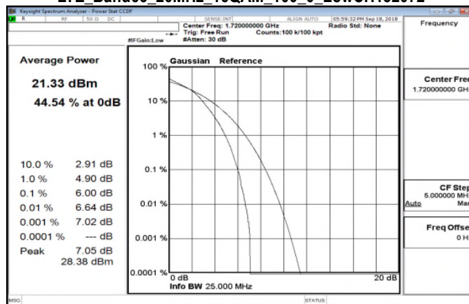
LTE_Band66_20MHz_16QAM_100_0_LowCH132072
