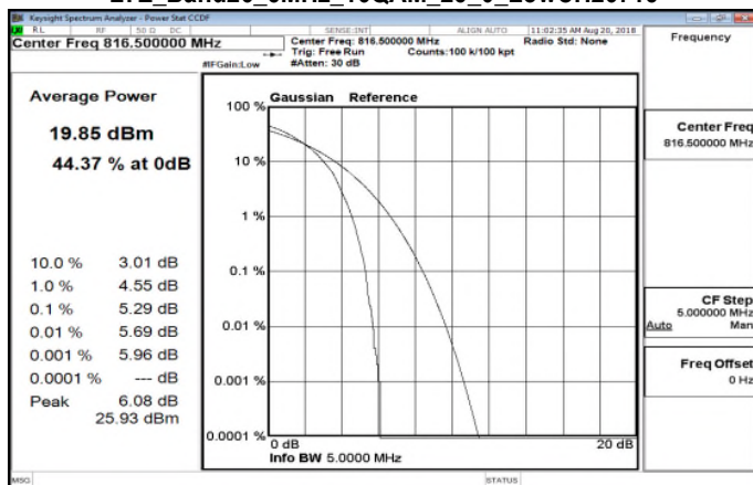
LTE_Band26_5MHz_16QAM_25_0_LowCH26715
