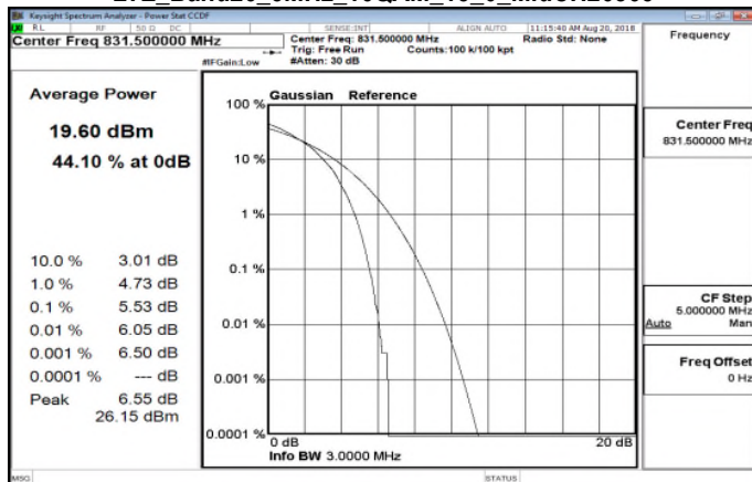
LTE_Band26_3MHz_16QAM_15_0_MidCH26865
