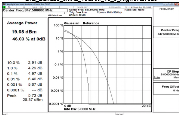
LTE_Band26_3MHz_16QAM_15_0_HighCH27025
