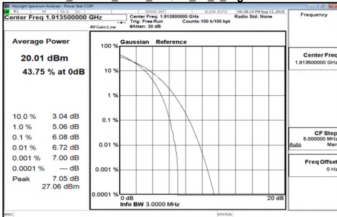
LTE_Band25_3MHz_16QAM_15_0_HighCH26675
