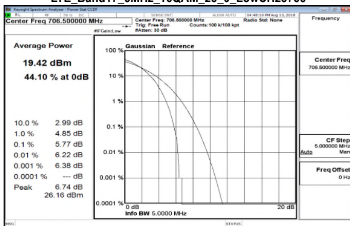
LTE_Band17 5MHz_16QAM_25_0_LowCH23755
