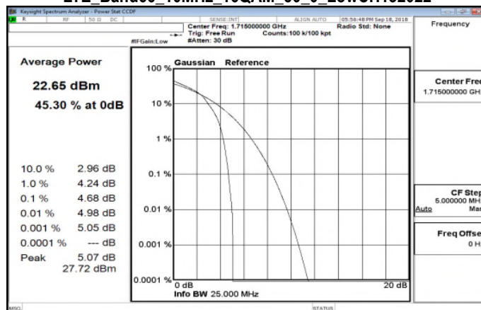
LTE_Band66_10MHz_16QAM_50_0_LowCH132022
