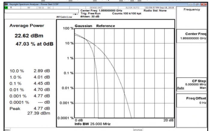
LTE_Band25_10MHz_16QAM_50_0_LowCH26090
