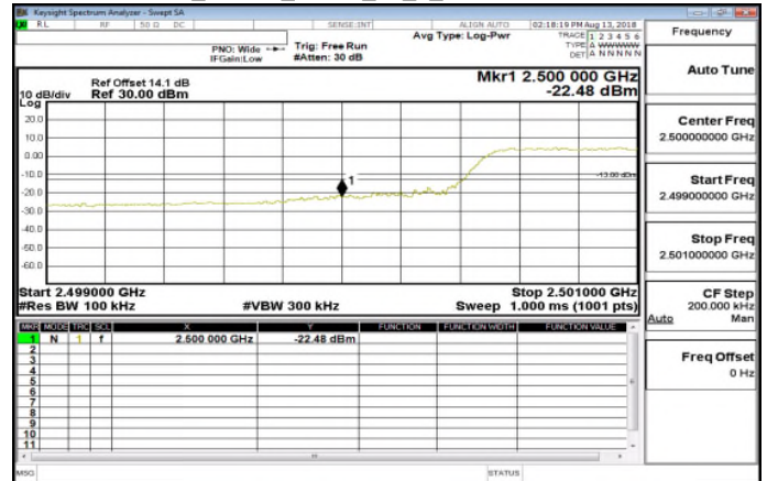
Band7_10MHz_QPSK_50_0_LowCH20800-2505
