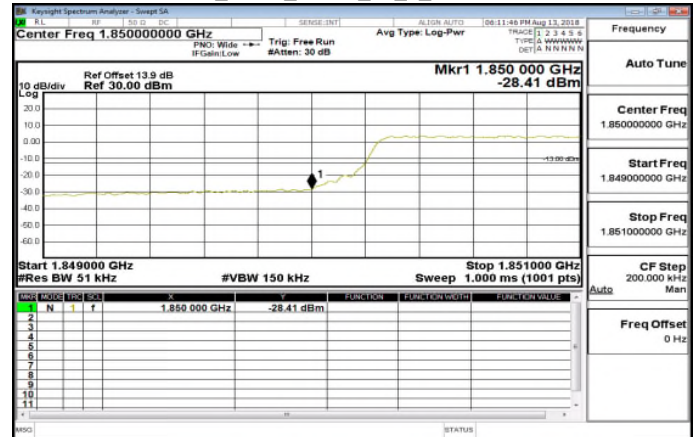
Band25_5MHz_QPSK_25_0_LowCH26065
