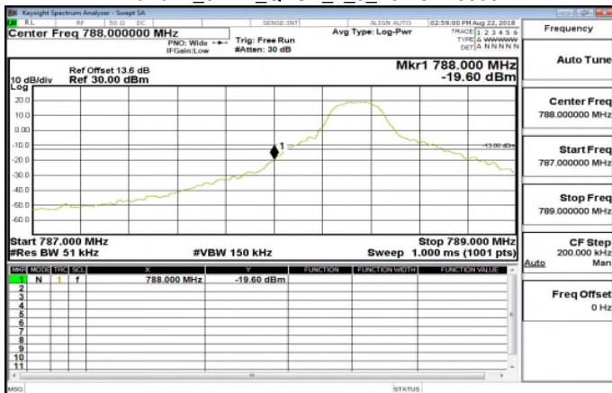
Band14_5MHz_QPSK_1_0_LowCH23305
