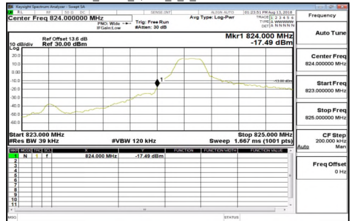
Band5_3MHz_QPSK_1_0_LowCH20415-825.5
