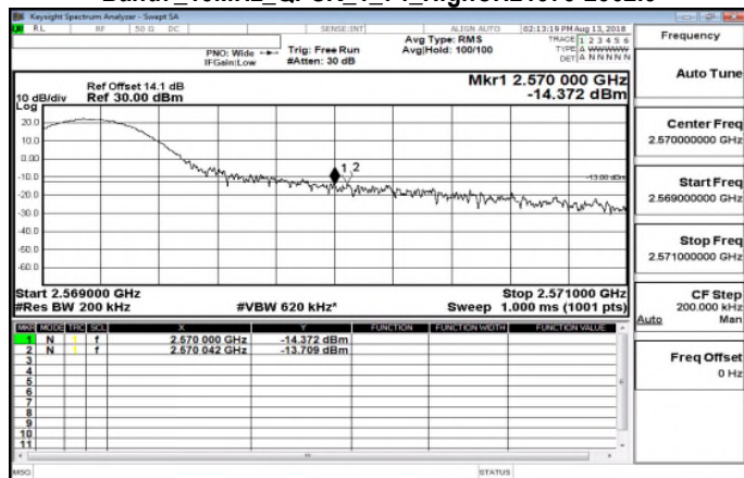
Band7_15MHz_QPSK_1_74_HighCH21375-2562.5
