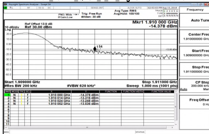
Band2 15MHz QPSK 1 74 HighCH19125-1902.5
