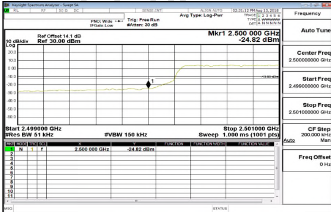
Band7_5MHz_QPSK_25_0_LowCH20775-2502.5
