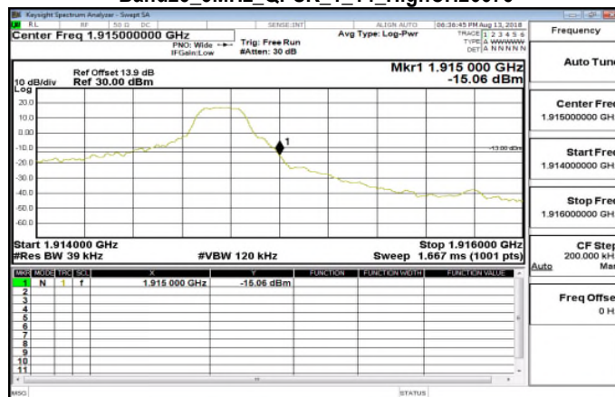
Band25_3MHz_QPSK_1_14_HighCH26675
