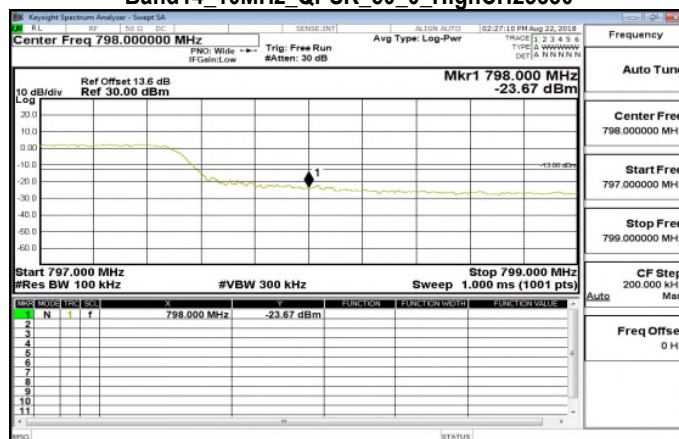
Band14_10MHz_QPSK_50_0_HighCH23330
