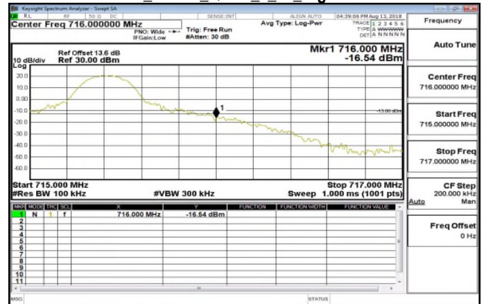
Band17_10MHz_QPSK_1_49_HighCH23800
