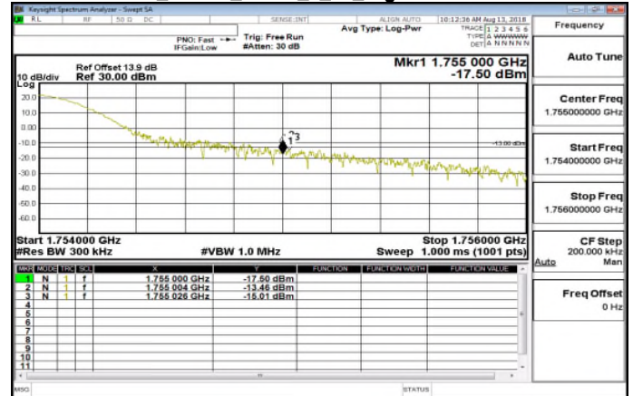
Band4 20MHz_QPSK 1_99_HighCH20300-1745
