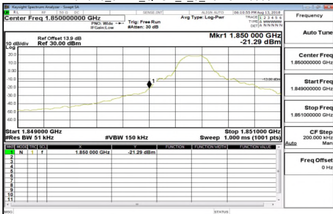
Band25_5MHz_QPSK_1_0_LowCH26065
