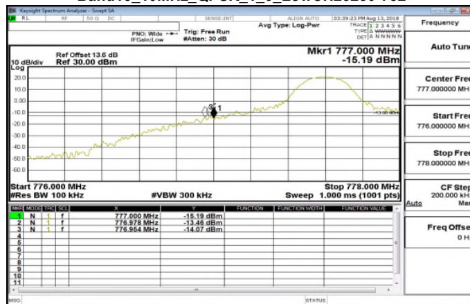
Band13_10MHz_QPSK_1_0_LowCH23230-782
