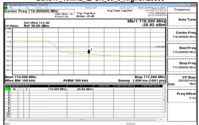
Band17_10MHz_QPSK_50_0_HighCH23800
