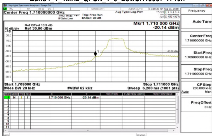
Band4_1_4MHz_QPSK_1_0_LowCH19957-1710.7
