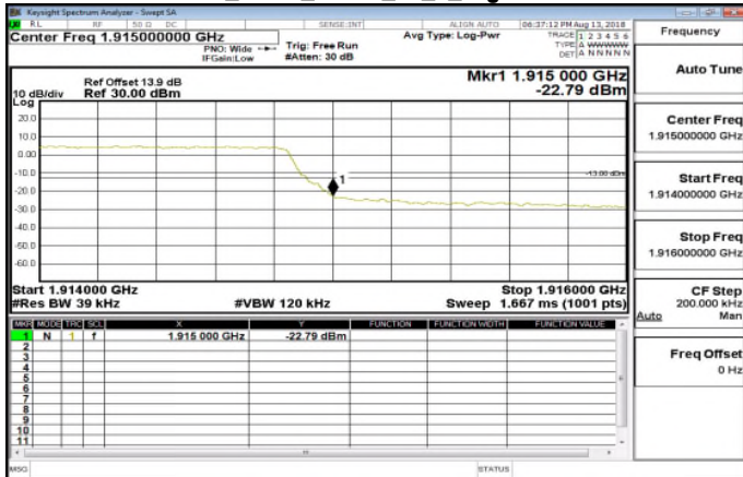
Band25_3MHz_QPSK_15_0_HighCH26675
