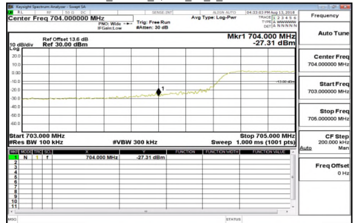
Band17_10MHz_QPSK_50_0_LowCH23780
