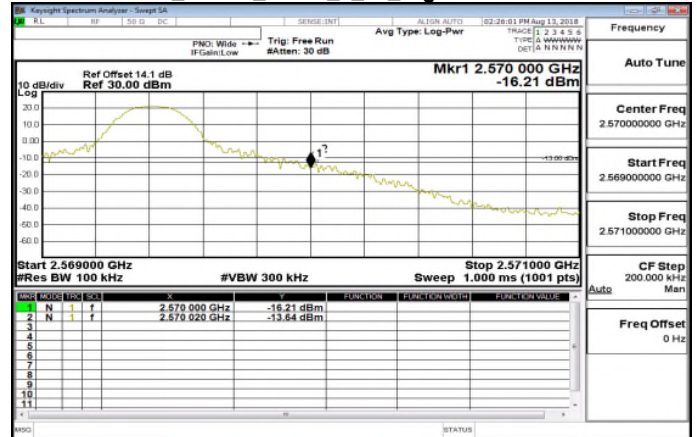
Band7_10MHz_QPSK_1_49_HighCH21400-2565
