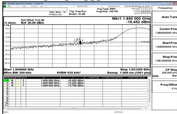
Band2 15MHz QPSK 1 0 LowCH18675-1857.5
