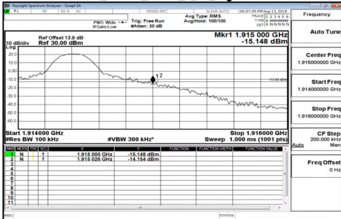
Band25_10MHz_QPSK_1_49_HighCH26640
