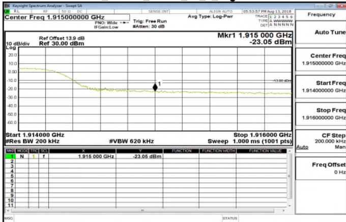
Band25 15MHz QPSK 75 0 HighCH26615
