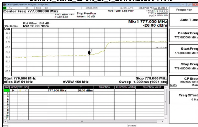
Band13_5MHz_QPSK_25_0_LowCH23205-779.5
