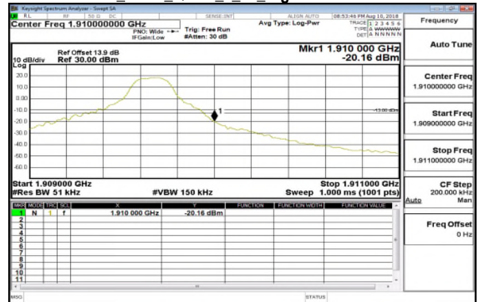
Band2 5MHz QPSK 1 24 HighCH19175-1907.5
