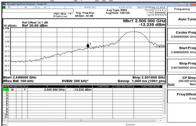
Band7_10MHz_QPSK_1_0_LowCH20800-2505
