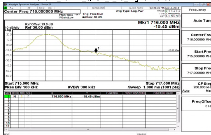
Band12_10MHz_QPSK_1_49_HighCH23130-711
