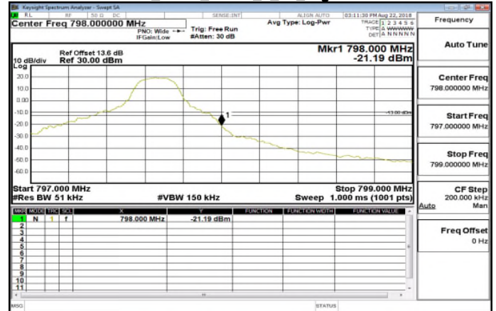
Band14_5MHz_QPSK_1_24_HighCH23355
