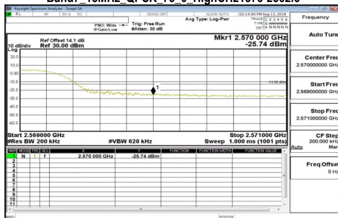
Band7_15MHz_QPSK_75_0_HighCH21375-2562.5
