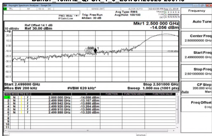
Band7_15MHz_QPSK_1_0_LowCH20825-2507.5
