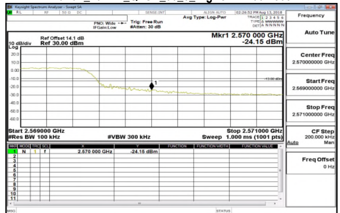
Band7_10MHz_QPSK_50_0_HighCH21400-2565
