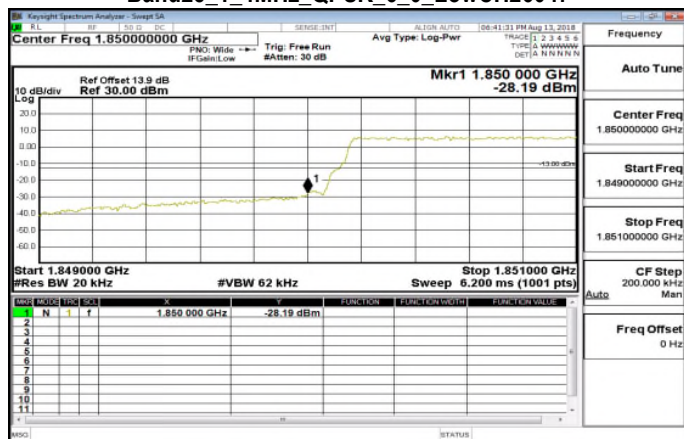
Band25_1_4MHz_QPSK_6_0_LowCH26047
