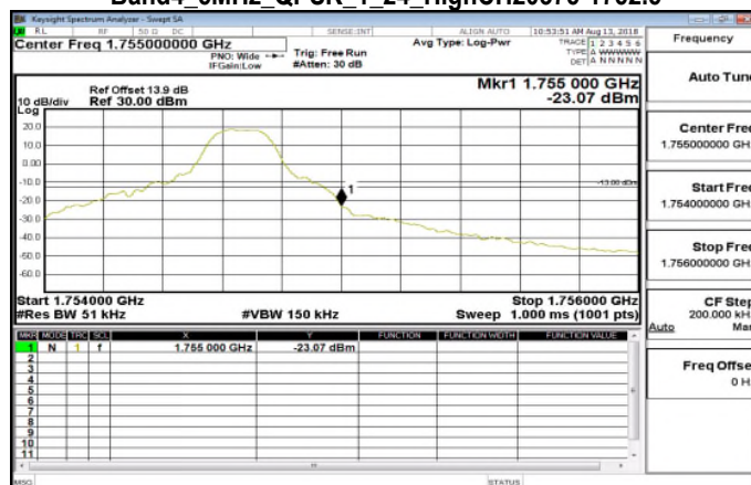
Band4 5MHz QPSK 1 24 HighCH20375-1752.5
