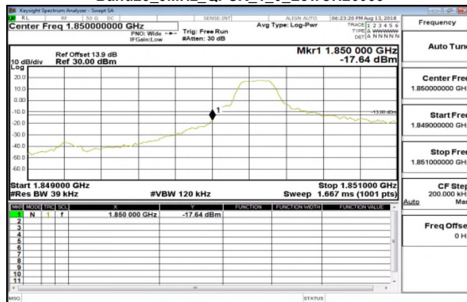
Band25_3MHz_QPSK_1_0_LowCH26055
