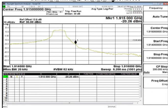
Band25_1_4MHz_QPSK_1_5_HighCH26683
