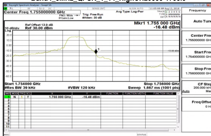
Band4_3MHz_QPSK_1_14_HighCH20385-1753.5
