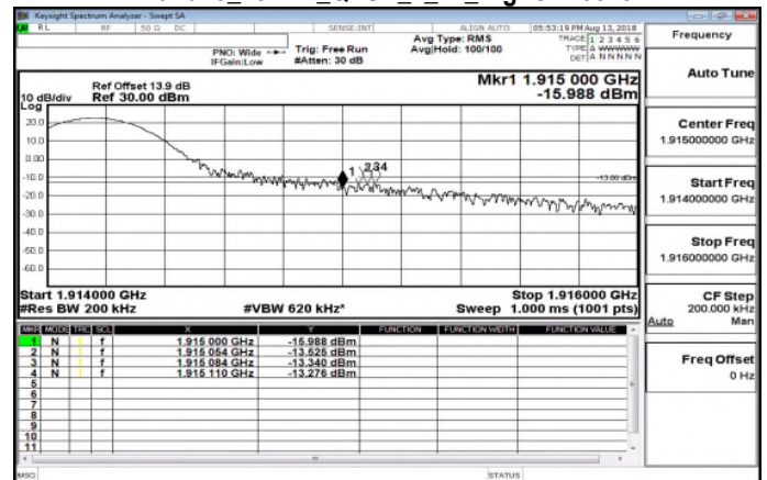
Band25_15MHz_QPSK_1_74_HighCH26615
