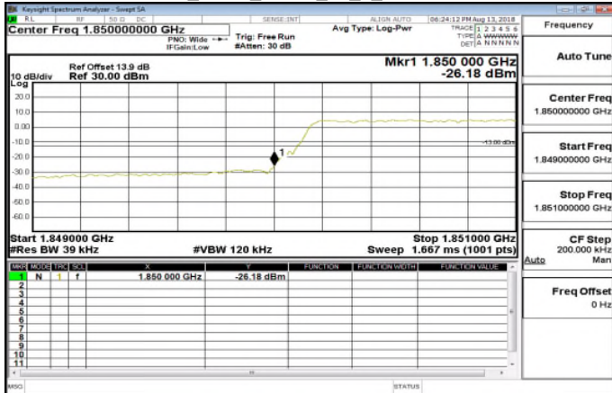
Band25_3MHz_QPSK_15_0_LowCH26055
