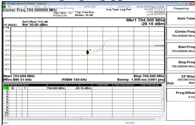
Band17_5MHz_QPSK_25_0_LowCH23755
