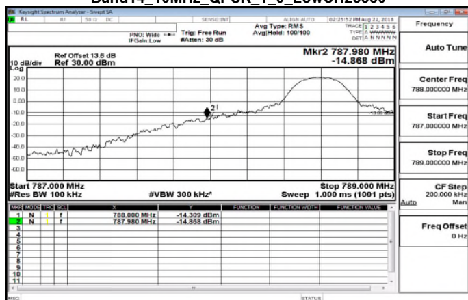
Band14_10MHz_QPSK_1_0_LowCH23330
