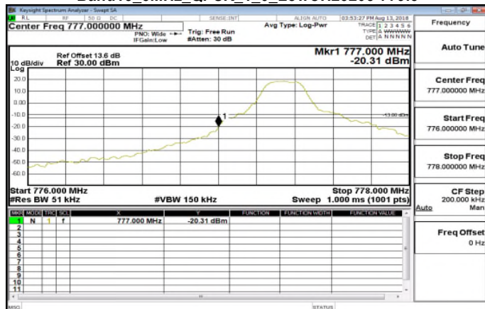
Band13_5MHz_QPSK_1_0_LowCH23205-779.5
