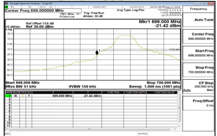
Band12_5MHz_QPSK_1_0_LowCH23035-701.5
