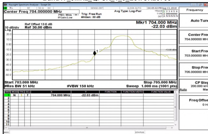
Band17_5MHz_QPSK_1_0_LowCH23755
