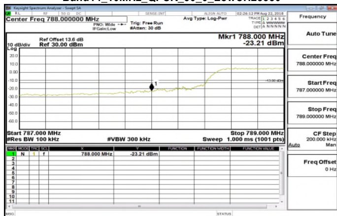
Band14_10MHz_QPSK_50_0_LowCH23330
