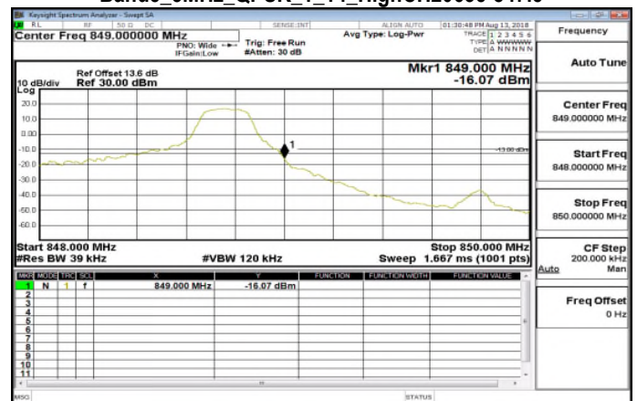
Band5_3MHz_QPSK_1_14_HighCH20635-847.5
