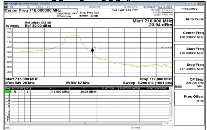
Band12 1 4MHz QPSK 1 5 HighCH23173-715.3
