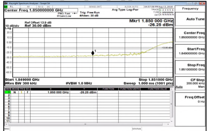
Band25 20MHz QPSK 100 0 LowCH26140
