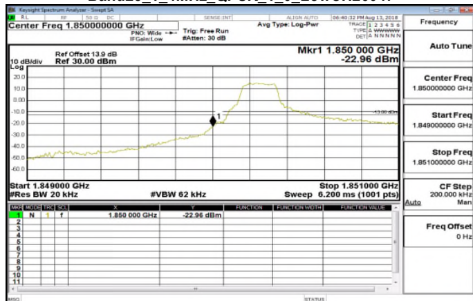
Band25_1_4MHz_QPSK_1_0_LowCH26047
