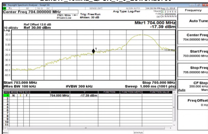
Band17_10MHz_QPSK_1_0_LowCH23780
