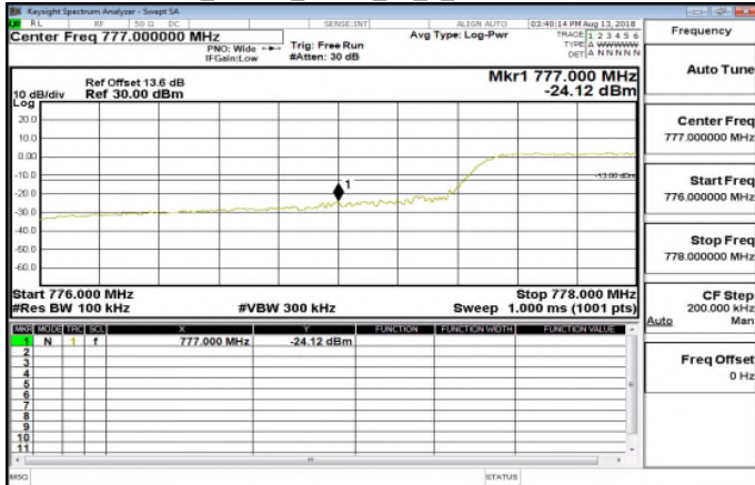
Band13_10MHz_QPSK_50_0_LowCH23230-782
