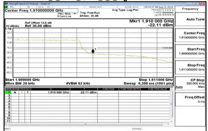
Band2 1 4MHz QPSK 6 0 HighCH19193-1909.3
