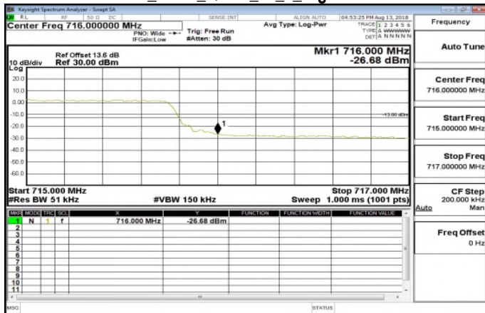
Band17_5MHz_QPSK_25_0_HighCH23825
