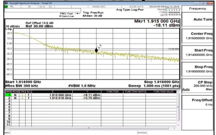
Band25 20MHz QPSK 1 99 HighCH26590
