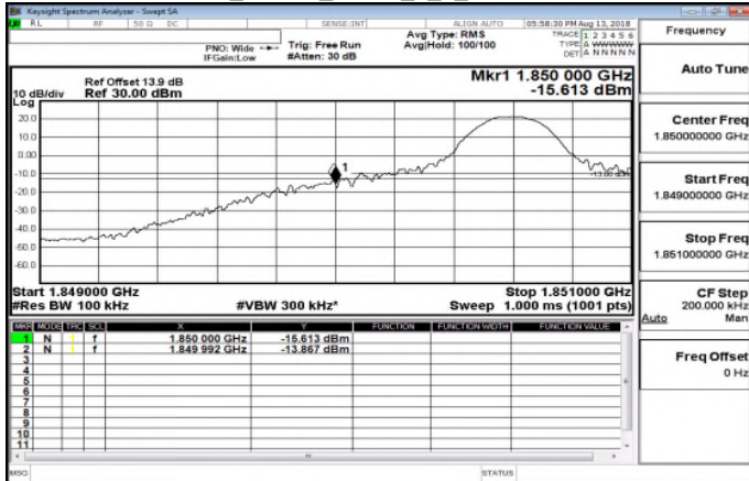
Band25_10MHz_QPSK_1_0_LowCH26090
