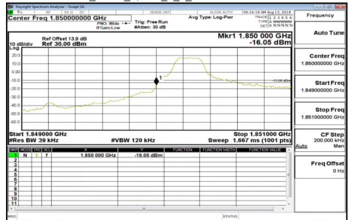
Band2 3MHz QPSK 1 0 LowCH18615-1851.5
