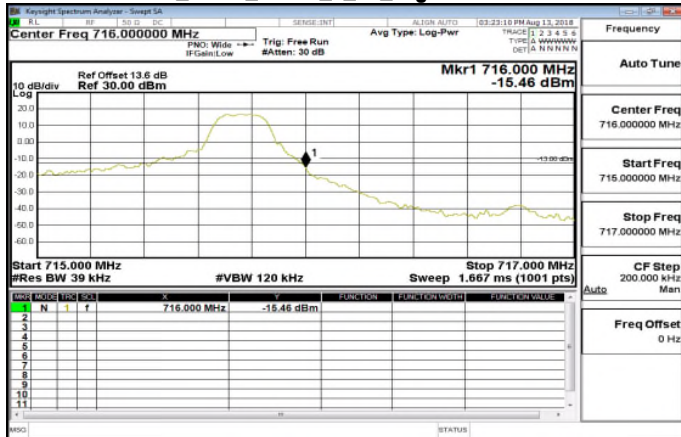
Band12_3MHz_QPSK_1_14_HighCH23165-714.5
