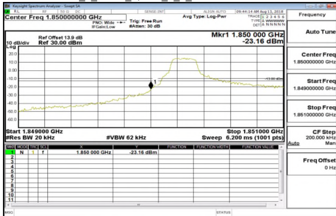
Band2 1 4MHz QPSK 1 0 LowCH18607-1850.7
