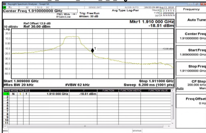
Band2 1 4MHz QPSK 1 5 HighCH19193-1909.3
