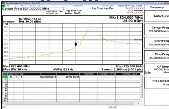
Band5_1_4MHz_QPSK_1_0_LowCH20407-824.7
