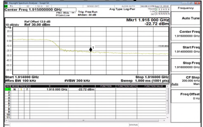
Band25_10MHz_QPSK_50_0_HighCH26640
