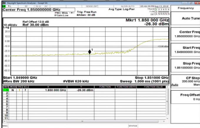
Band25 15MHz QPSK 75 0 LowCH26115
