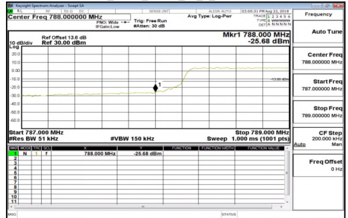
Band14_5MHz_QPSK_25_0_LowCH23305
