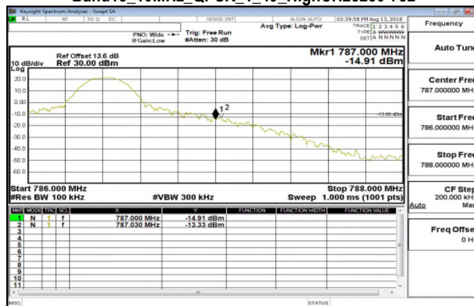
Band13_10MHz_QPSK_1_49_HighCH23230-782
