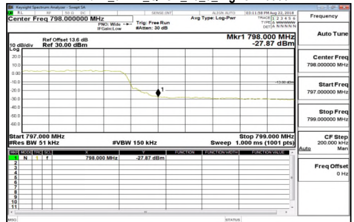
Band14_5MHz_QPSK_25_0_HighCH23355
