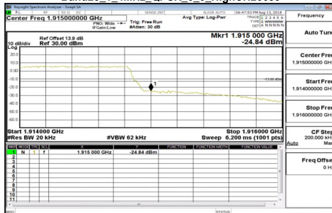
Band25_1_4MHz_QPSK_6_0_HighCH26683
