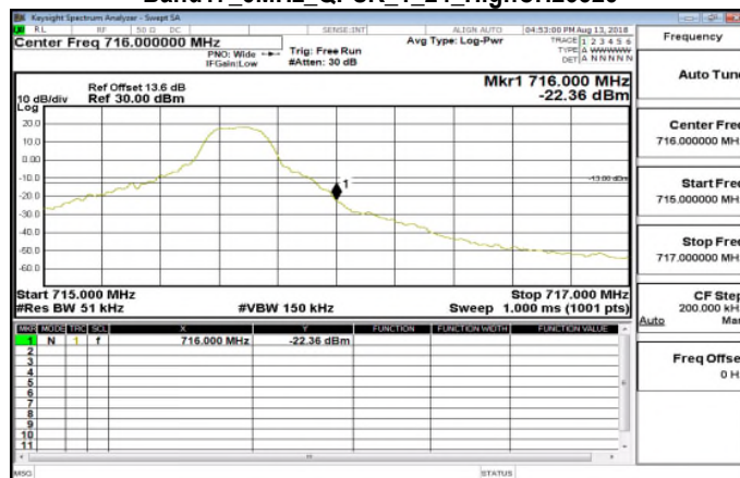
Band17_5MHz_QPSK_1_24_HighCH23825
