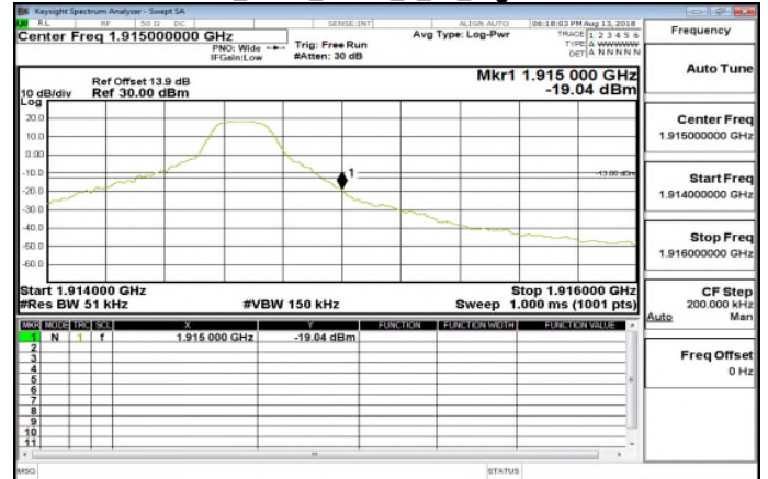
Band25_5MHz_QPSK_1_24_HighCH26665
