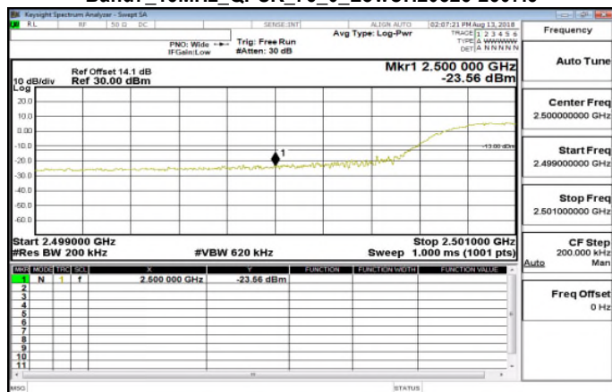
Band7_15MHz_QPSK_75_0_LowCH20825-2507.5
