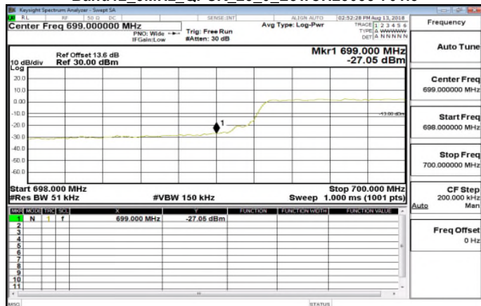
Band12_5MHz_QPSK_25_0_LowCH23035-701.5
