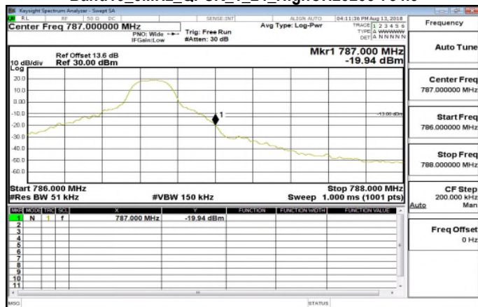
Band13_5MHz_QPSK_1_24_HighCH23255-784.5
