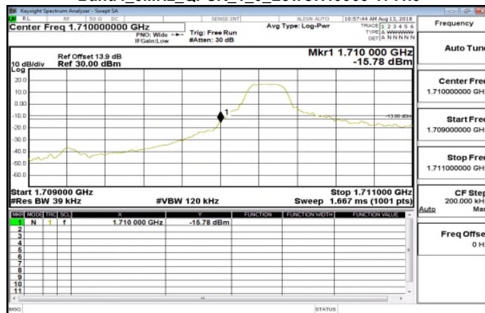
Band4_3MHz_QPSK_1_0_LowCH19965-1711.5
