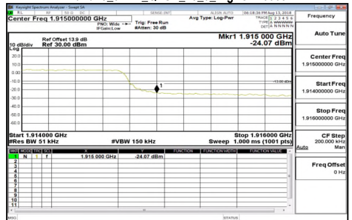
Band25_5MHz_QPSK_25_0_HighCH26665
