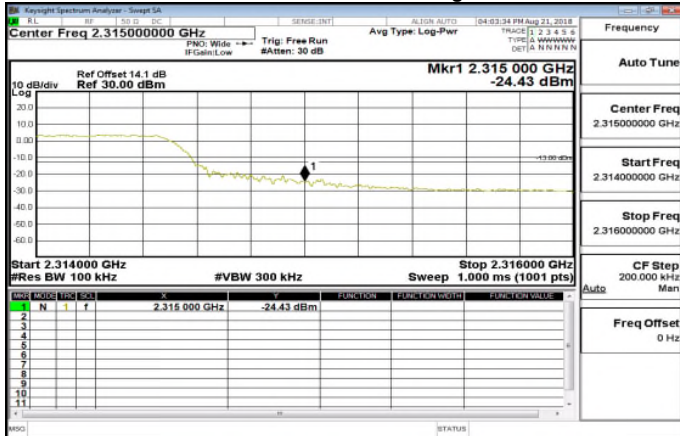
Band30_10MHz_QPSK_50_0_HighCH27710
