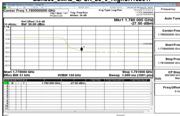
Band66_5MHz_QPSK_25_0_HighCH132647
