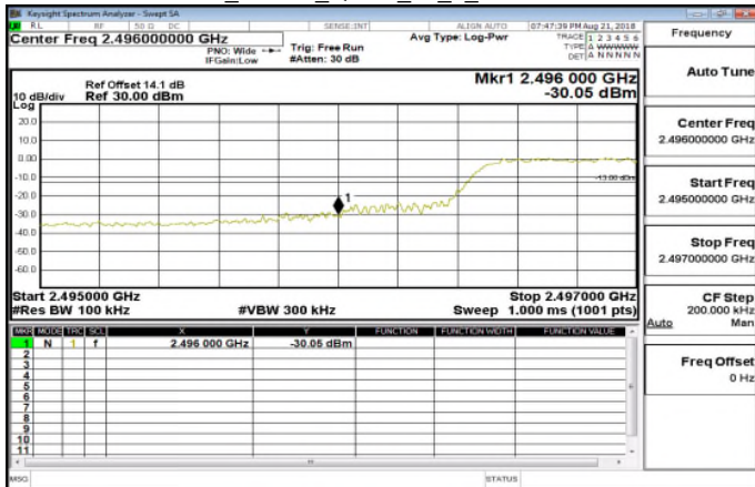
Band41_10MHz_QPSK_50_0_LowCH39700
