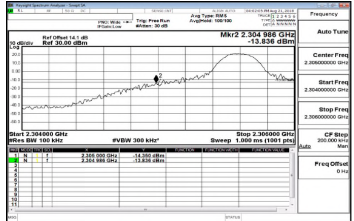
Band30_10MHz_QPSK_1_0_LowCH27710
