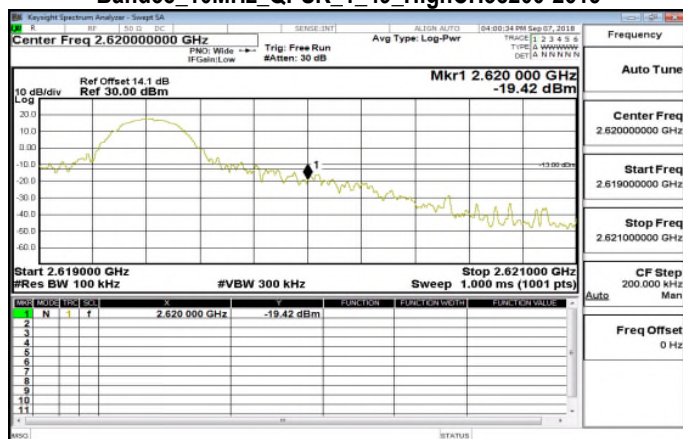
Band38_10MHz_QPSK_1_49_HighCH38200-2615
