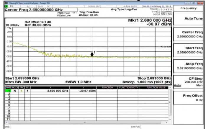
Band41_20MHz_QPSK_100_0_HighCH41490
