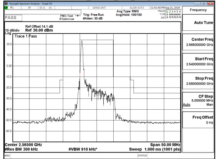
Band 7_16QAM_10M_RB1,49
