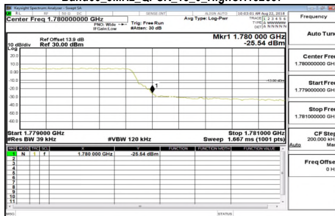
Band66_3MHz_QPSK_15_0_HighCH132657
