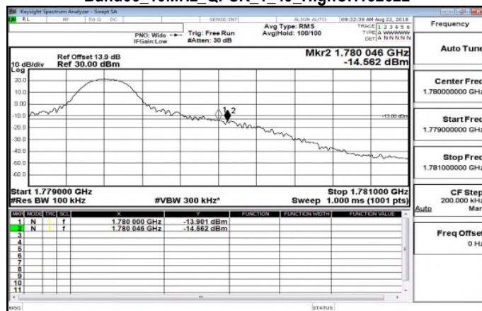
Band66_10MHz_QPSK_1_49_HighCH132622
