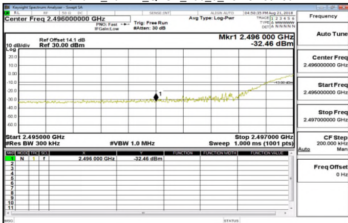
Band41_20MHz_QPSK_100_0_LowCH39750
