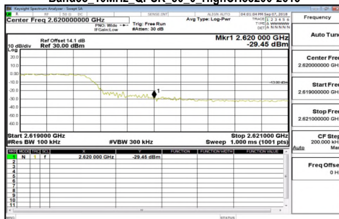
Band38_10MHz_QPSK_50_0_HighCH38200-2615
