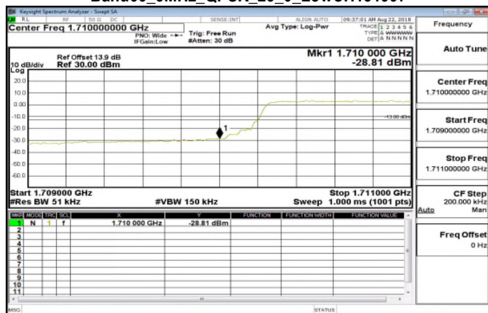
Band66_5MHz_QPSK_25_0_LowCH131997
