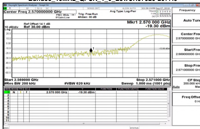
Band38_15MHz_QPSK_1_0_LowCH37825-2577.5
