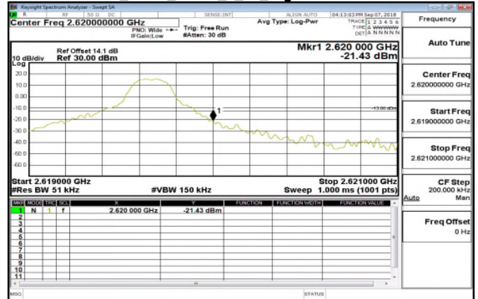
Band38_5MHz_QPSK_1_24_HighCH38225-2617.5
