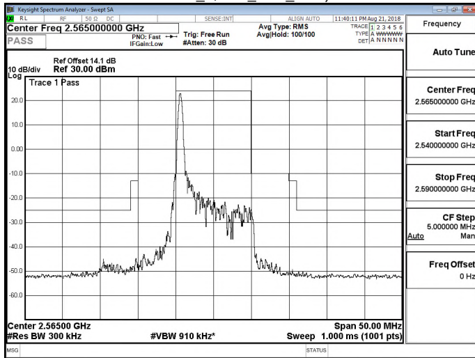
Band 7_QPSK_10M_RB1,49
