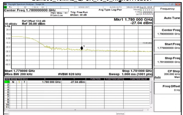
Band66_15MHz_QPSK_75_0_HighCH132597
