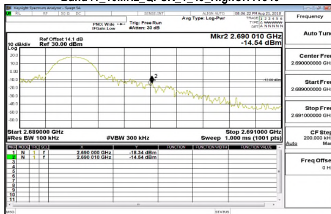
Band41_10MHz_QPSK_1_49_HighCH41540
