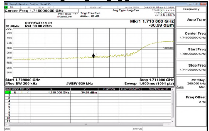
Band66_15MHz_QPSK_75_0_LowCH132047
