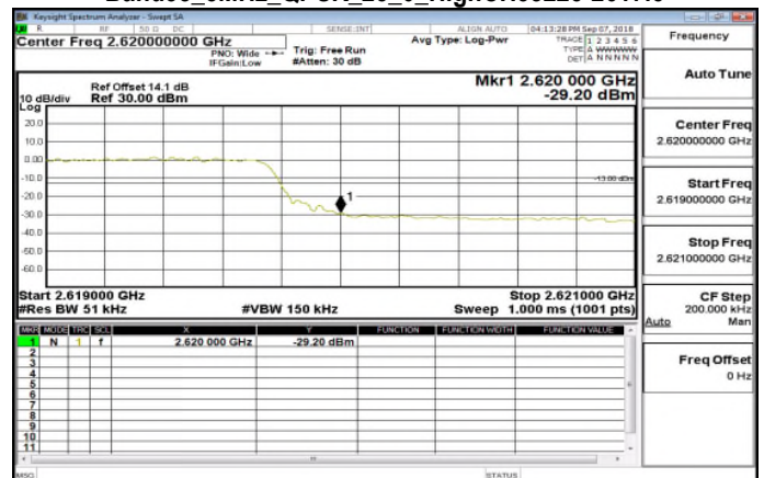
Band38_5MHz_QPSK_25_0_HighCH38225-2617.5
