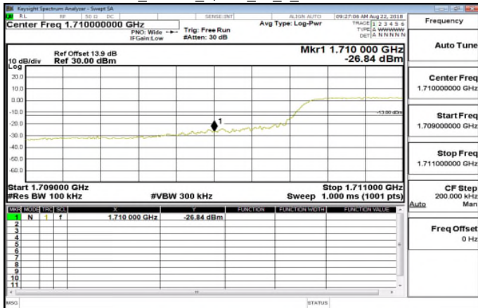
Band66_10MHz_QPSK_50_0_LowCH132022
