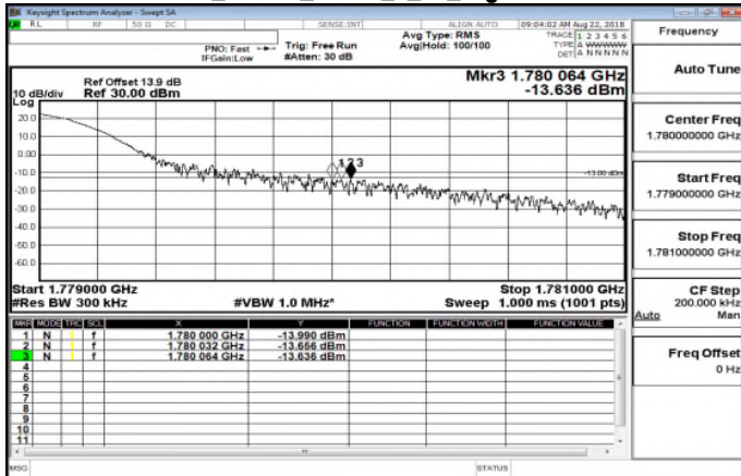
Band66_20MHz_QPSK_1_99_HighCH132572
