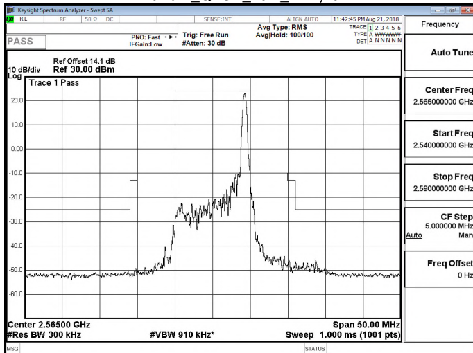
Band 7_QPSK_10M_RB50,0
