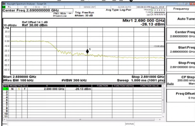
Band41_10MHz_QPSK_50_0_HighCH41540
