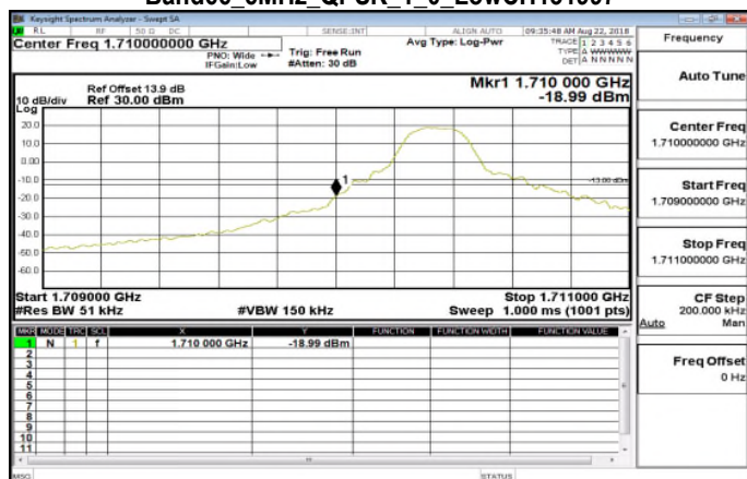
Band66_5MHz_QPSK_1_0_LowCH131997
