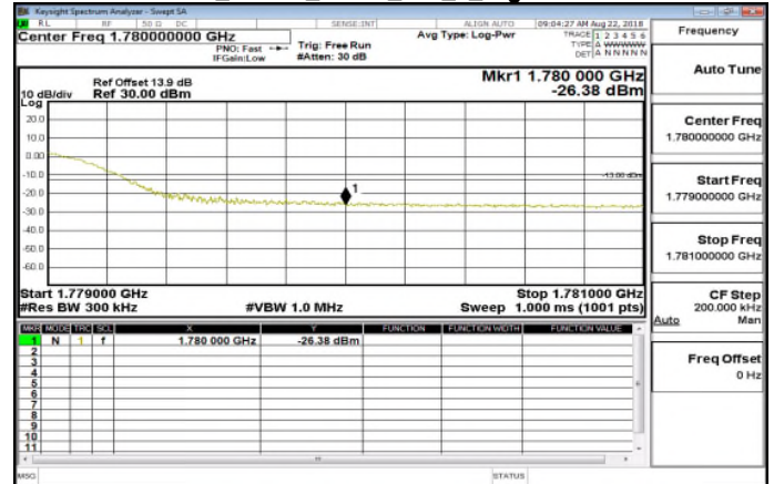
Band66_20MHz_QPSK_100_0_HighCH132572
