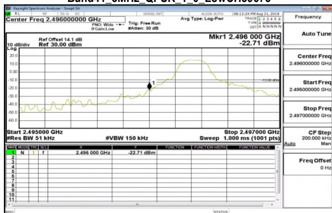
Band41_5MHz_QPSK_1_0_LowCH39675
