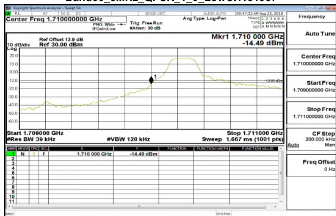
Band66_3MHz_QPSK_1_0_LowCH131987
