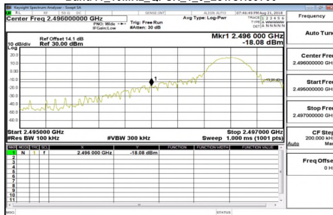
Band41_10MHz_QPSK_1_0_LowCH39700
