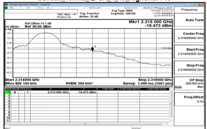
Band30_10MHz_QPSK_1_49_HighCH27710
