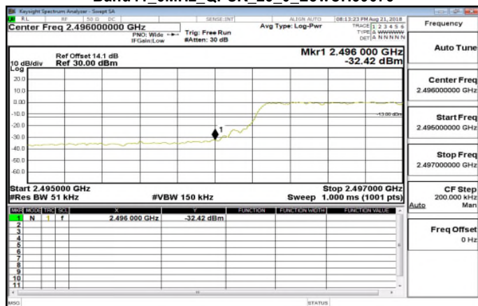
Band41_5MHz_QPSK_25_0_LowCH39675
