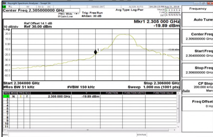
Band30_5MHz_QPSK_1_0_LowCH27685
