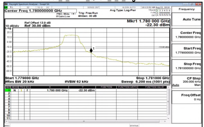
Band66_1_4MHz_QPSK_1_5_HighCH132665
