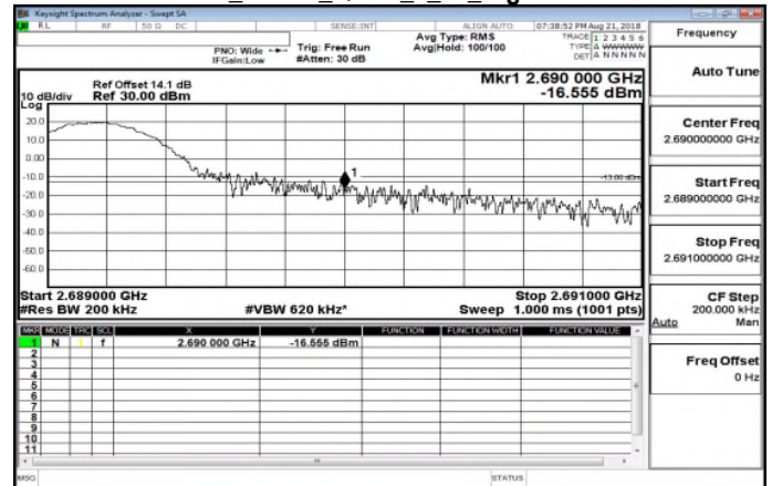
Band41_15MHz_QPSK_1_74_HighCH41515
