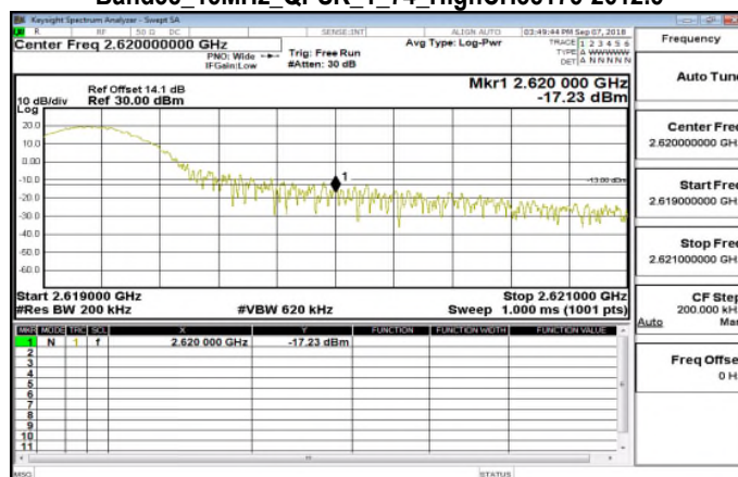
Band38_15MHz_QPSK_1_74_HighCH38175-2612.5
