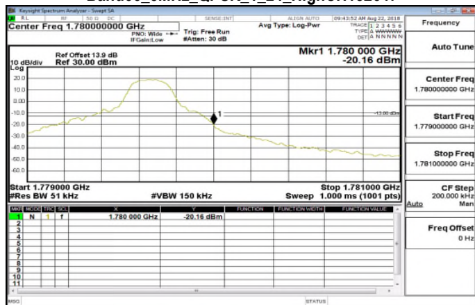
Band66_5MHz_QPSK_1_24_HighCH132647
