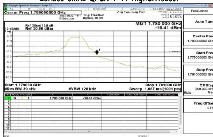
Band66_3MHz_QPSK_1_14_HighCH132657
