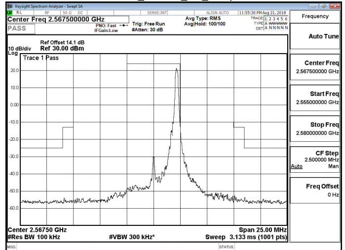
Band 7_16QAM_5M_RB25,0
