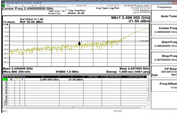
Band41_20MHz_QPSK_1_0_LowCH39750
