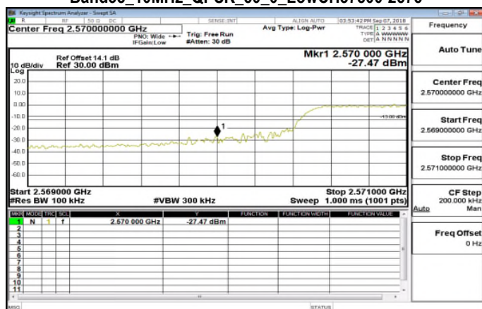
Band38_10MHz_QPSK_50_0_LowCH37800-2575
