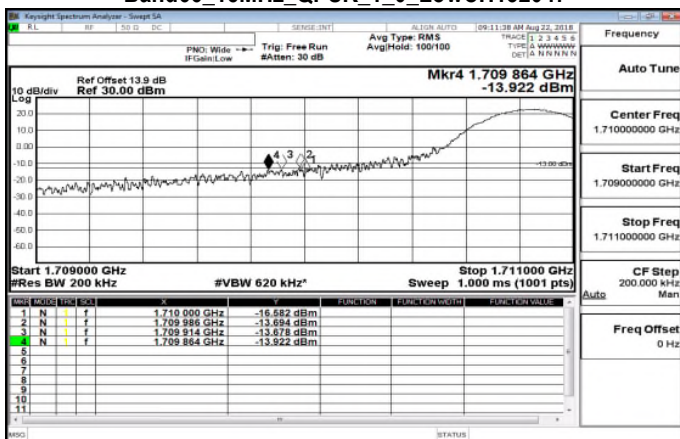
Band66_15MHz_QPSK_1_0_LowCH132047
