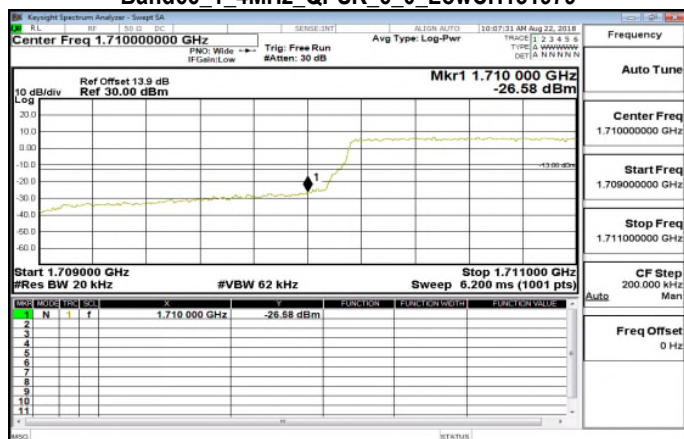
Band66_1_4MHz_QPSK_6_0_LowCH131979
