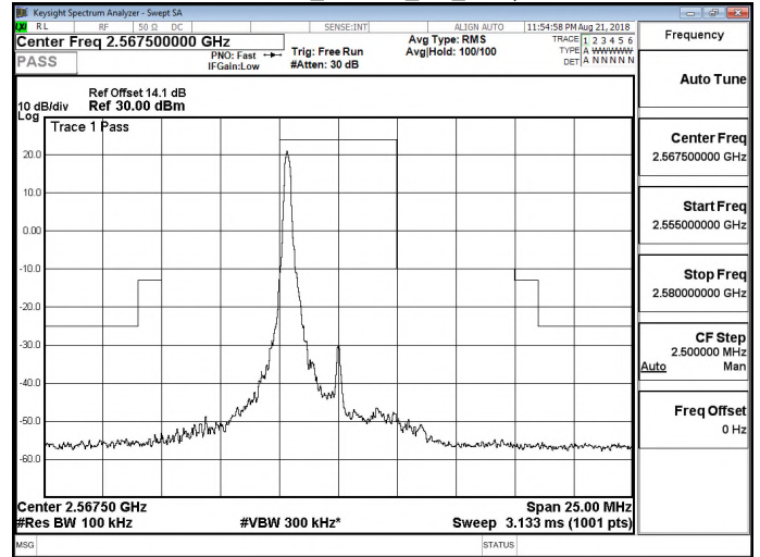
Band 7_16QAM_5M_RB1,24
