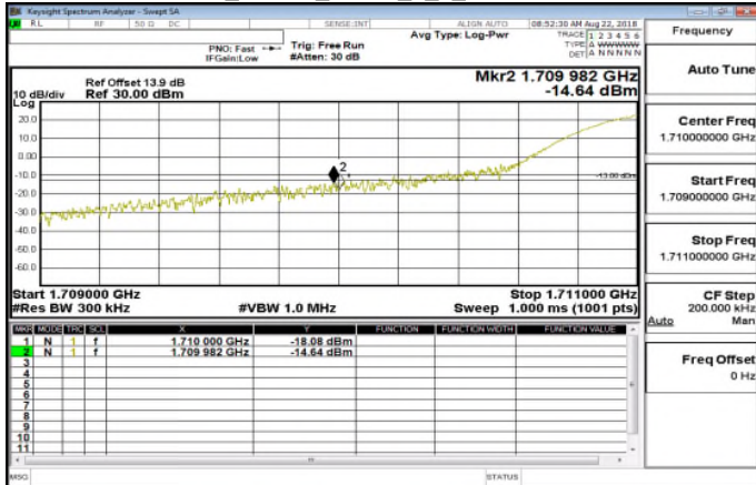
Band66_20MHz_QPSK_1_0_LowCH132072
