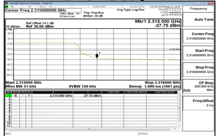
Band30_5MHz_QPSK_25_0_HighCH27735
