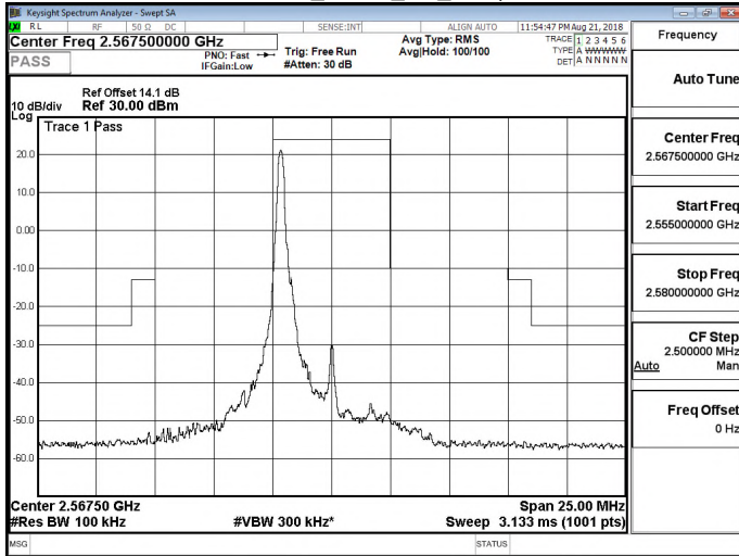
Band 7_QPSK_5M_RB1,24
