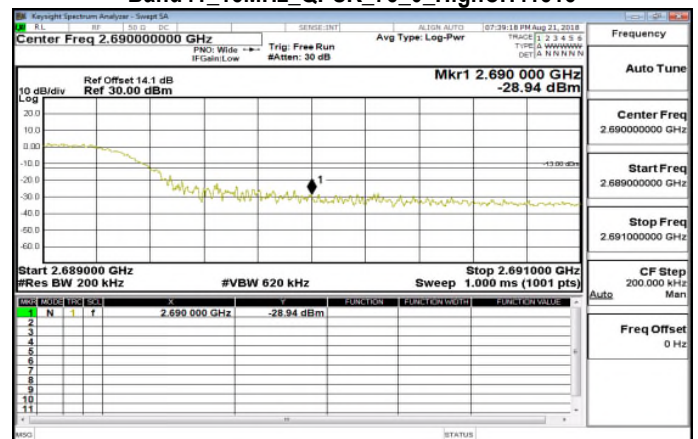
Band41_15MHz_QPSK_75_0_HighCH41515
