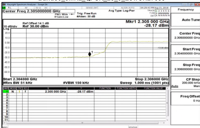
Band30_5MHz_QPSK_25_0_LowCH27685
