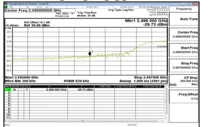
Band41_15MHz_QPSK_75_0_LowCH39725
