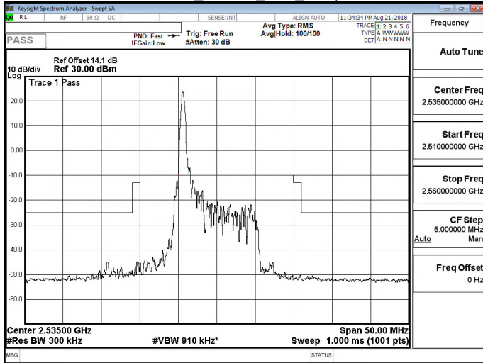
Band 7_16QAM_10M_RB1,49
