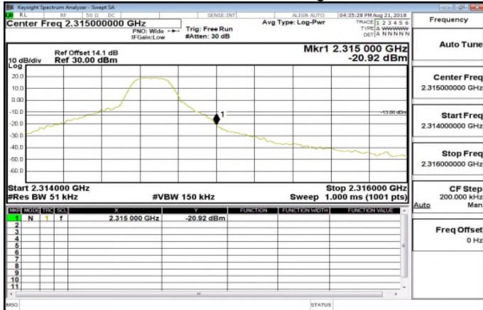
Band30_5MHz_QPSK_1_24_HighCH27735
