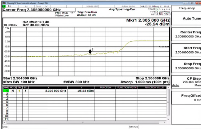
Band30_10MHz_QPSK_50_0_LowCH27710
