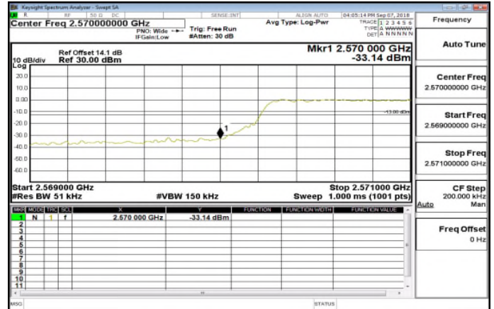
Band38_5MHz_QPSK_25_0_LowCH37775-2572.5
