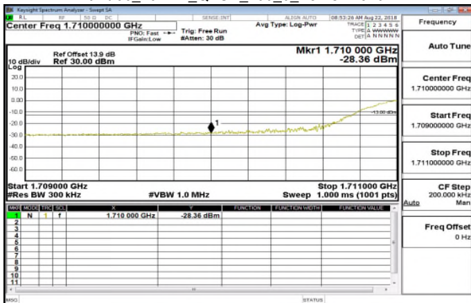
Band66_20MHz_QPSK_100_0_LowCH132072
