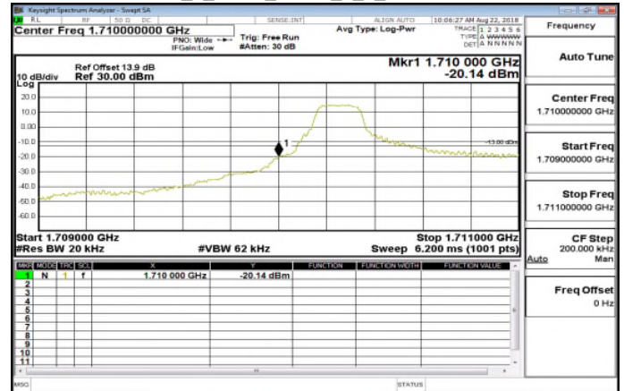
Band66_1_4MHz_QPSK_1_0_LowCH131979
