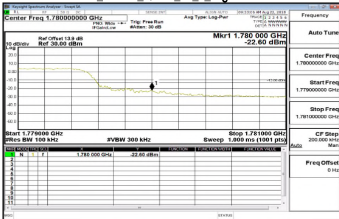
Band66_10MHz_QPSK_50_0_HighCH132622
