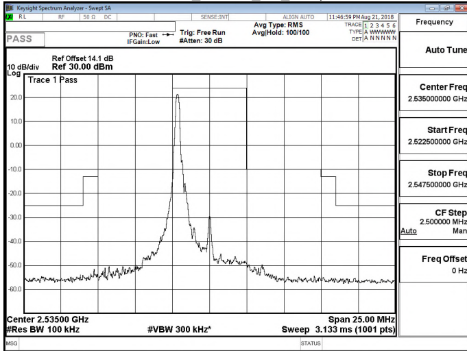
Band 7_16QAM_5M_RB1,24
