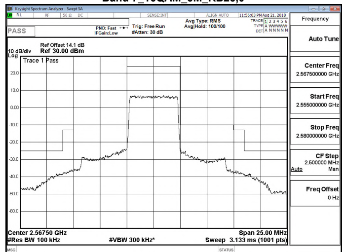
Band 7_16QAM_5M_RB25,0
