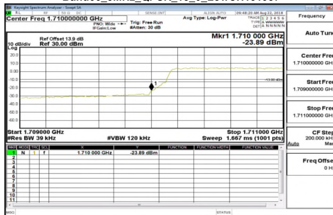
Band66_3MHz_QPSK_15_0_LowCH131987
