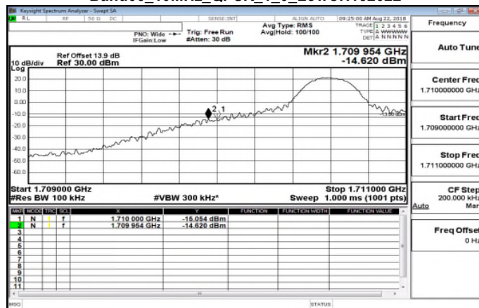
Band66_10MHz_QPSK_1_0_LowCH132022
