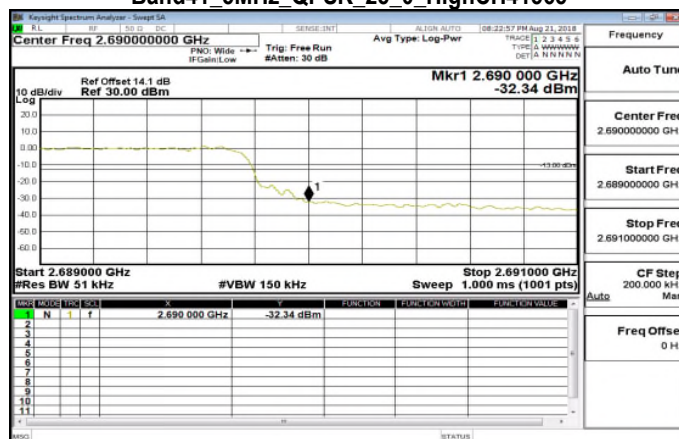
Band41_5MHz_QPSK_25_0_HighCH41565
