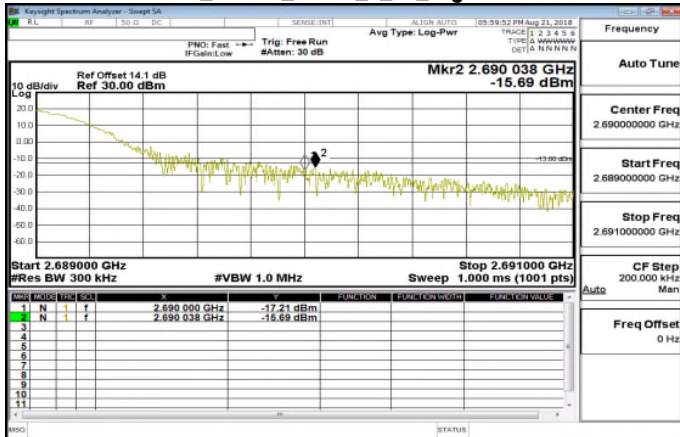
Band41_20MHz_QPSK_1_99_HighCH41490
