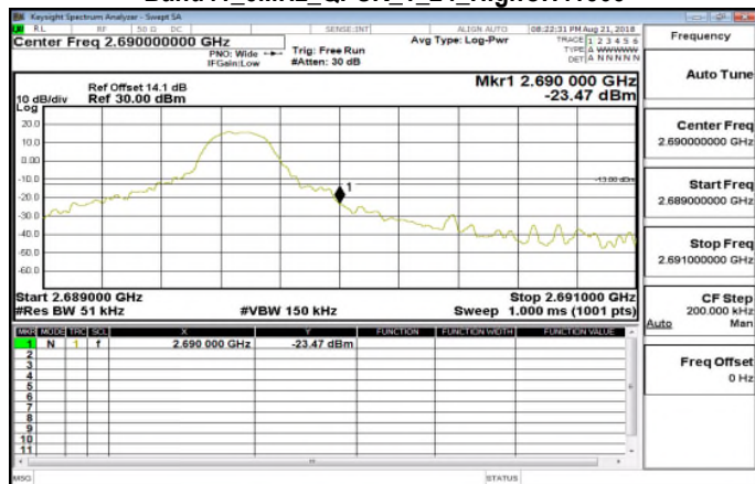
Band41_5MHz_QPSK_1_24_HighCH41565
