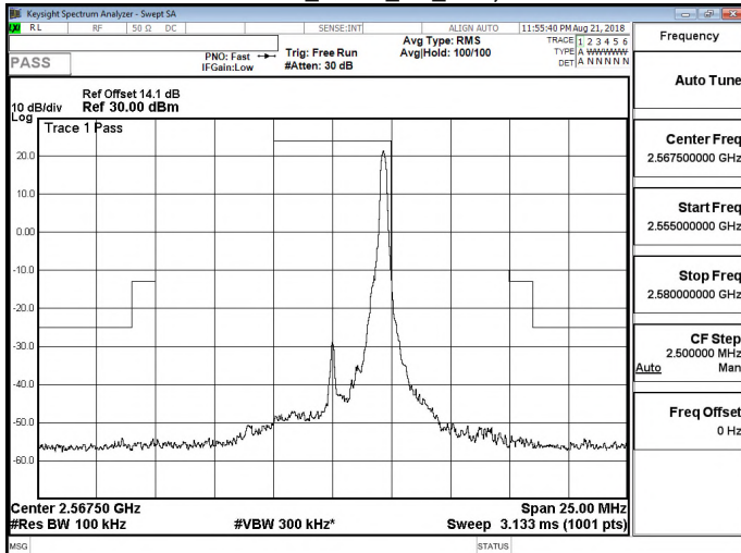
Band 7_QPSK_5M_RB25,0
