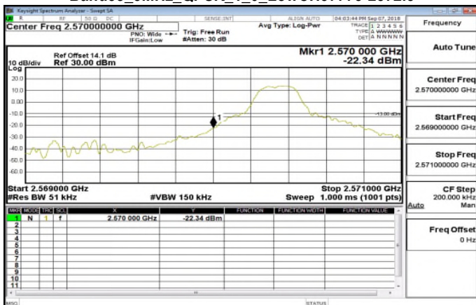
Band38_5MHz_QPSK_1_0_LowCH37775-2572.5
