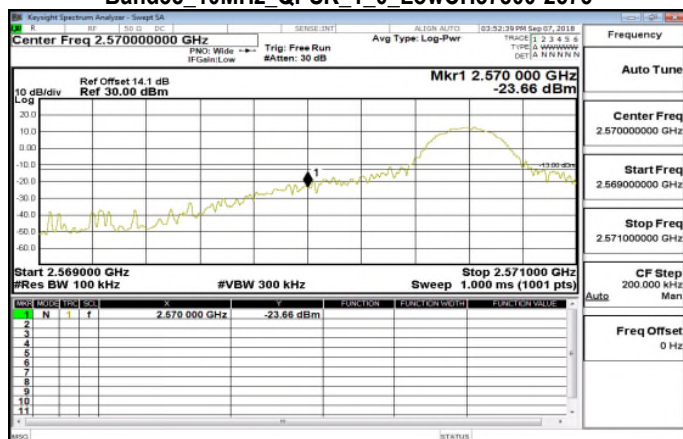
Band38_10MHz_QPSK_1_0_LowCH37800-2575
