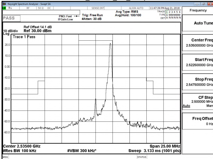
Band 7_16QAM_5M_RB25,0
