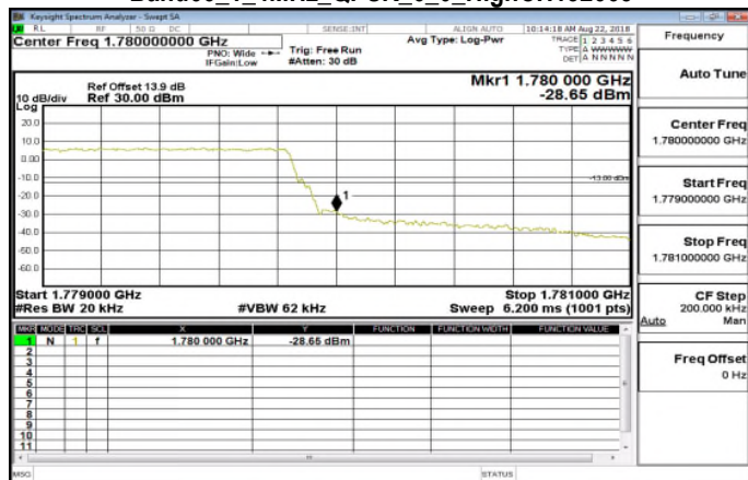
Band66_1_4MHz_QPSK_6_0_HighCH132665
