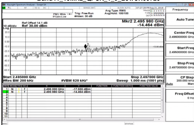
Band41_15MHz_QPSK_1_0_LowCH39725
