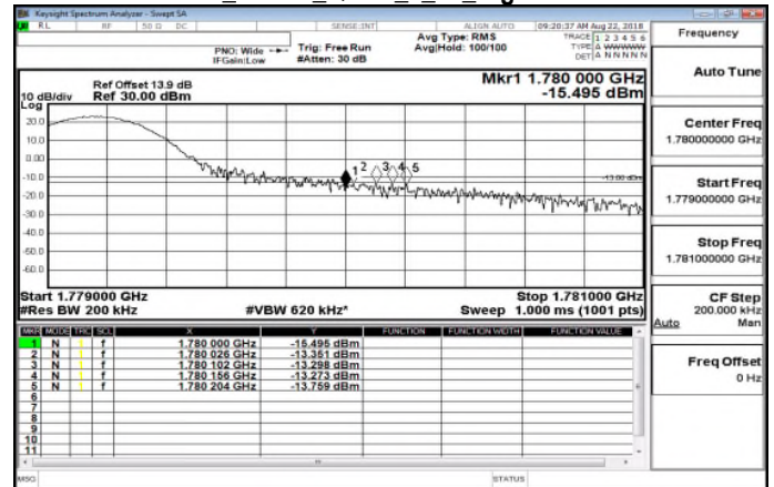
Band66_15MHz_QPSK_1_74_HighCH132597
