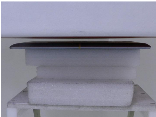
Bottom Face, Test Separation 1.2 cm
