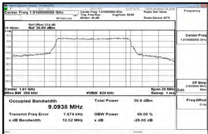
Band25_10MHz_16QAM_50_0_HighCH26640-1910
