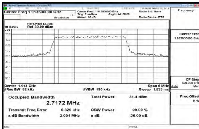
Band25_3MHz_64QAM_15_0_HighCH26675-1913.5
