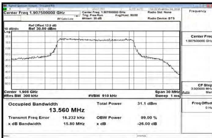
Band25_15MHz_16QAM_75_0_HighCH26615-1907.5
