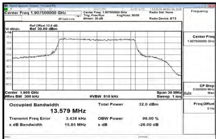
Band25_15MHz_QPSK_75_0_HighCH26615-1907.5
