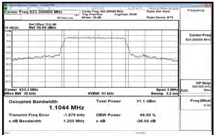
Band26_Part90s_1_4MHz_QPSK_6_0_Main_HighCH26783
