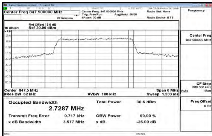
Band26_3MHz_16QAM_15_0_HighCH27025-847.5
