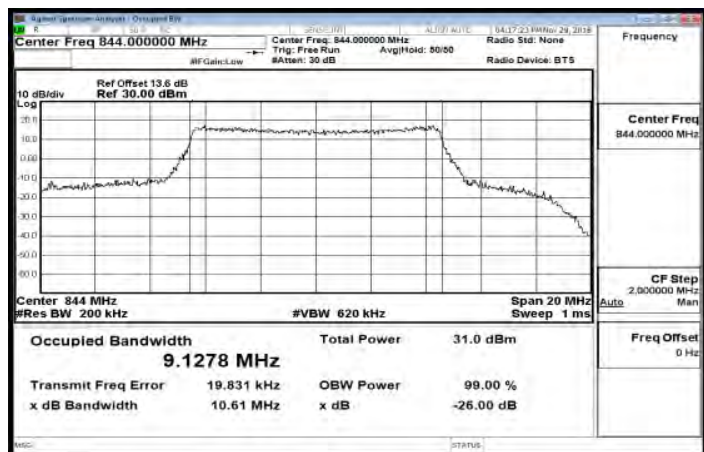
Band26_10MHz_16QAM_50_0_HighCH26990-844
