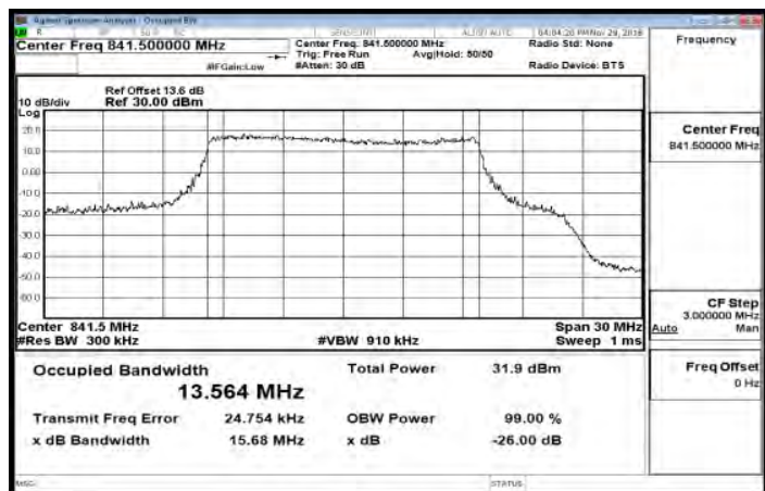
Band26_15MHz_QPSK_75_0_HighCH26965-841.5
