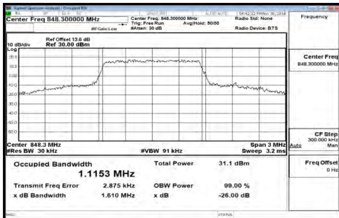
Band26_1_4MHz_QPSK_6_0_HighCH27033-848.3
