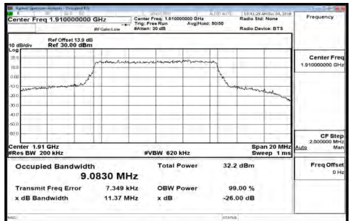
Band25_10MHz_QPSK_50_0_HighCH26640-1910
