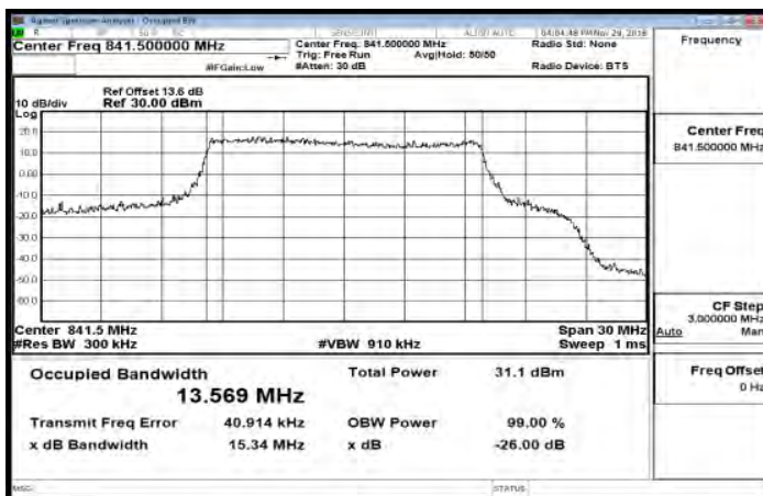
Band26_15MHz_16QAM_75_0_HighCH26965-841.5
