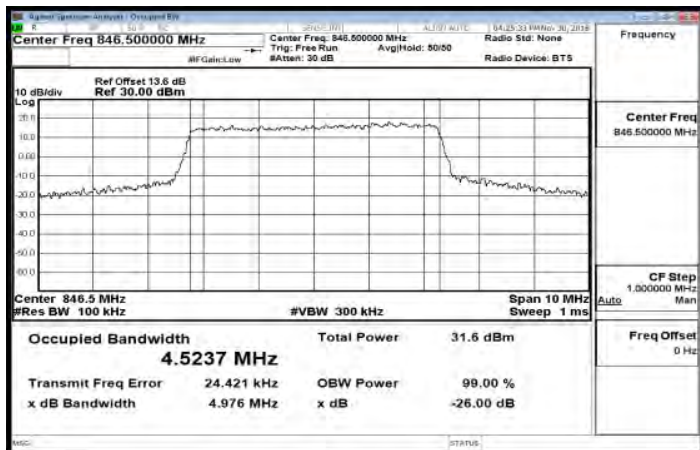
Band26_5MHz_QPSK_25_0_HighCH27015-846.5
