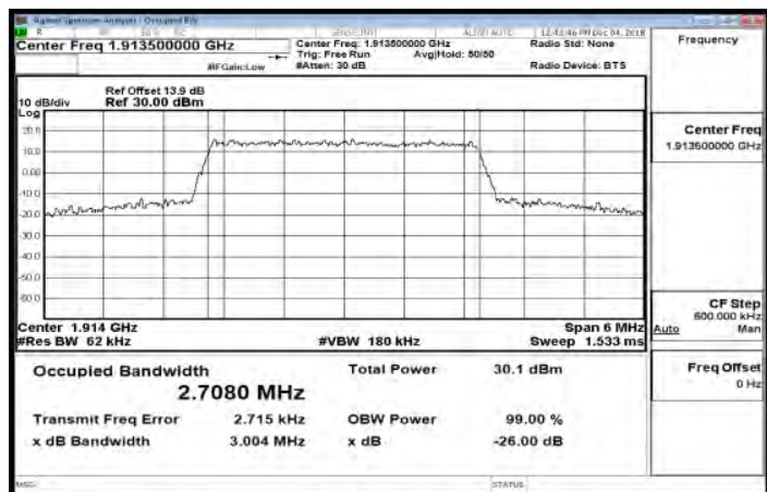
Band25_3MHz_16QAM_15_0_HighCH26675-1913.5
