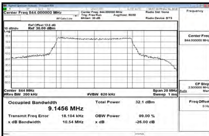
Band26_10MHz_64QAM_50_0_HighCH26990-844
