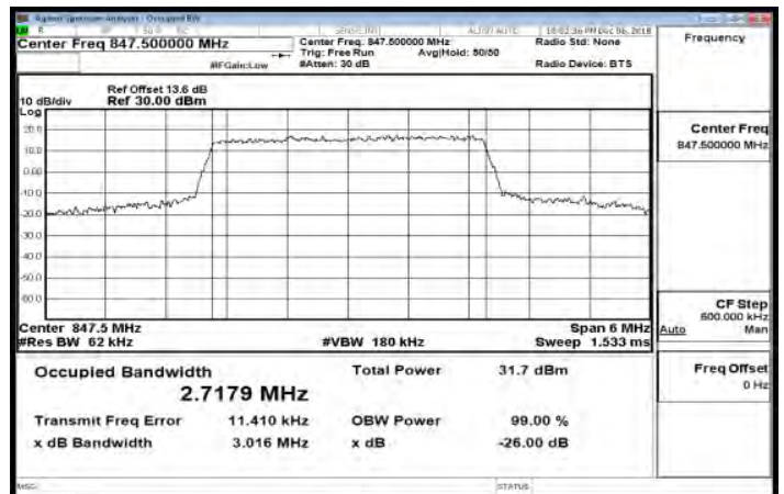
Band26_3MHz_64QAM_15_0_HighCH27025-847.5
