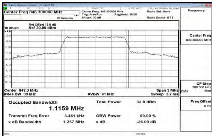
Band26_1_4MHz_64QAM_6_0_HighCH27033-848.3
