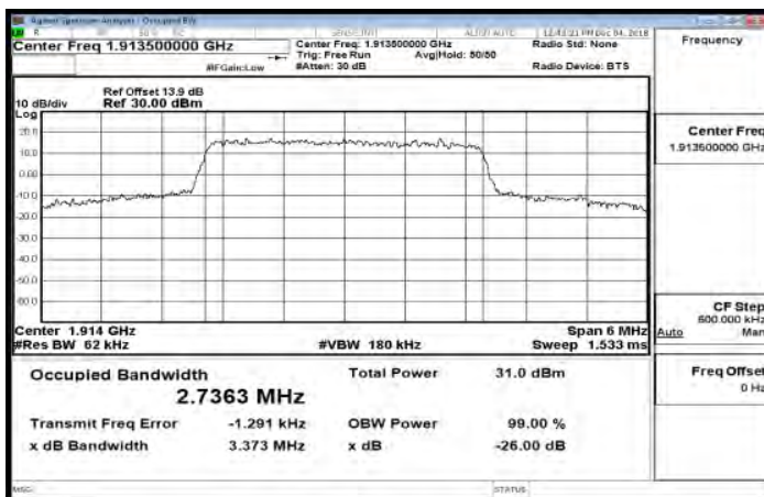
Band25_3MHz_QPSK_15_0_HighCH26675-1913.5
