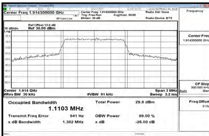
Band25_1_4MHz_16QAM_6_0_HighCH26683-1914.3
