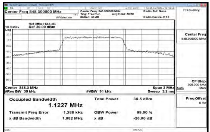
Band26_1_4MHz_16QAM_6_0_HighCH27033-848.3
