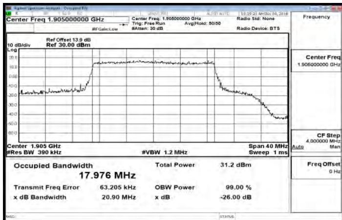
Band25_20MHz_16QAM_100_0_HighCH26590-1905
