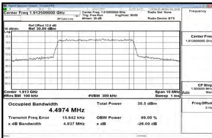
Band25_5MHz_16QAM_25_0_HighCH26665-1912.5
