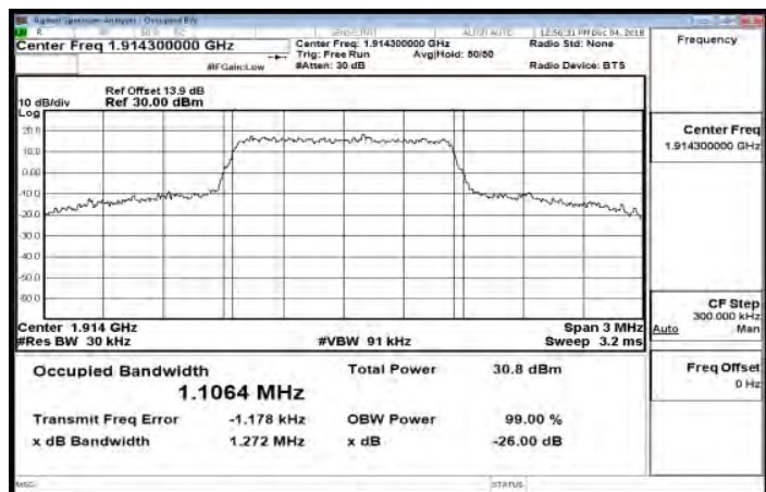
Band25_1_4MHz_QPSK_6_0_HighCH26683-1914.3
