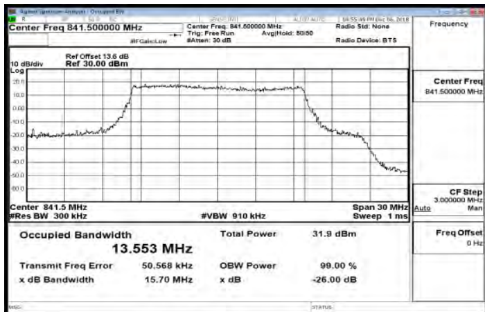
Band26_15MHz_64QAM_75_0_HighCH26965-841.5
