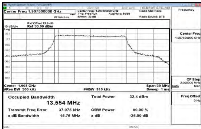
Band25_15MHz_64QAM_75_0_HighCH26615-1907.5
