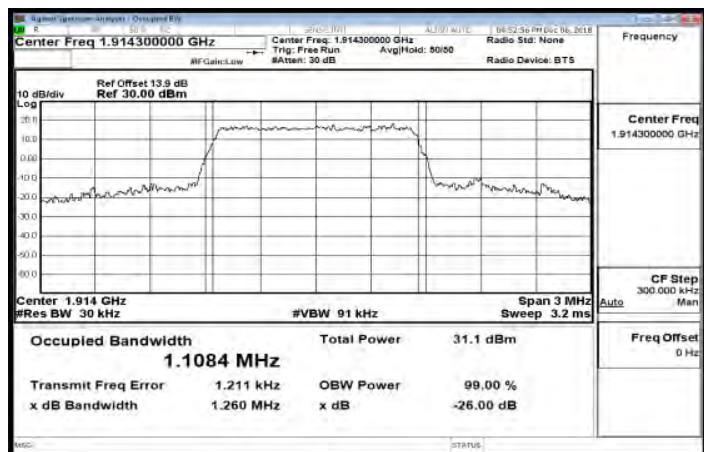
Band25_1_4MHz_64QAM_6_0_HighCH26683-1914.3
