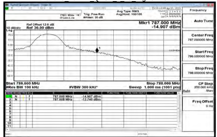
LTE\Band13 10MHz QPSK 1 49 HighCH23230-782
