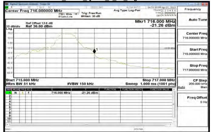
LTE\Band12 5MHz QPSK 1 24 HighCH23155-713.5
