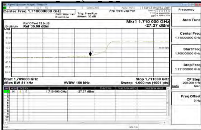
LTE/Band66 5MHz QPSK 25 0 LowCH131997-1712.5
