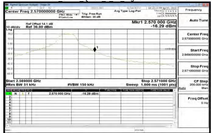
LTE\Band7 5MHz QPSK 1 24 HighCH21425-2567.5
