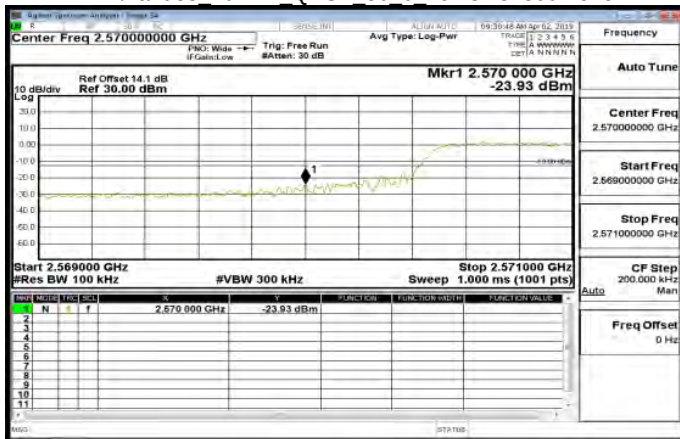
LTE\Band38 10MHz QPSK 50 0 LowCH37800-2575
