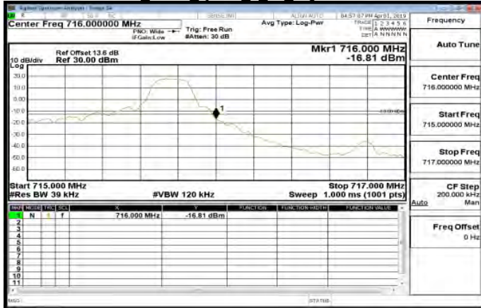
LTE\Band12 3MHz QPSK 1 14 HighCH23165-714.5
