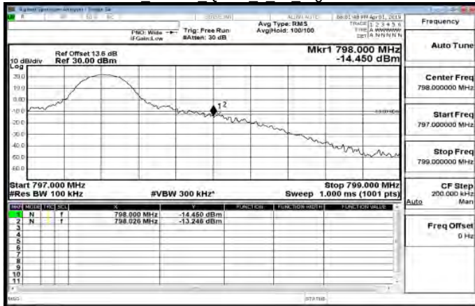
LTE\Band14 10MHz QPSK 50 0 LowCH23330-793
