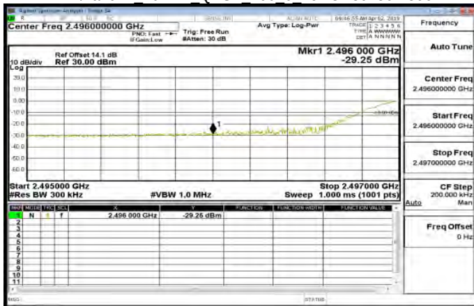
LTE\Band41 20MHz QPSK 100 0 LowCH39750-2506
