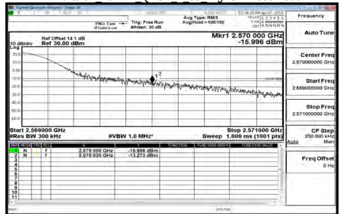
LTE\Band7 20MHz QPSK 1 99 HighCH21350-2560
