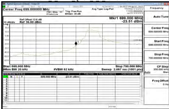
LTE\Band12 1 4MHz QPSK 1 0 LowCH23017-699.7
