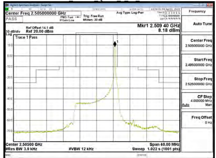
Band7 10MHz QPSK 50 0 CH20800
