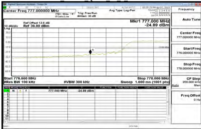
LTE\Band13 10MHz QPSK 50 0 HighCH23230-782
