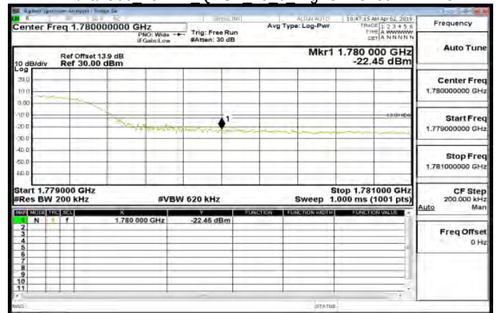
LTE\Band66 15MHz QPSK 75 0 HighCH132597-1772.5
