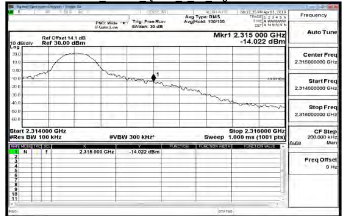
LTE\Band30 10MHz QPSK 1 49 HighCH27710-2310
