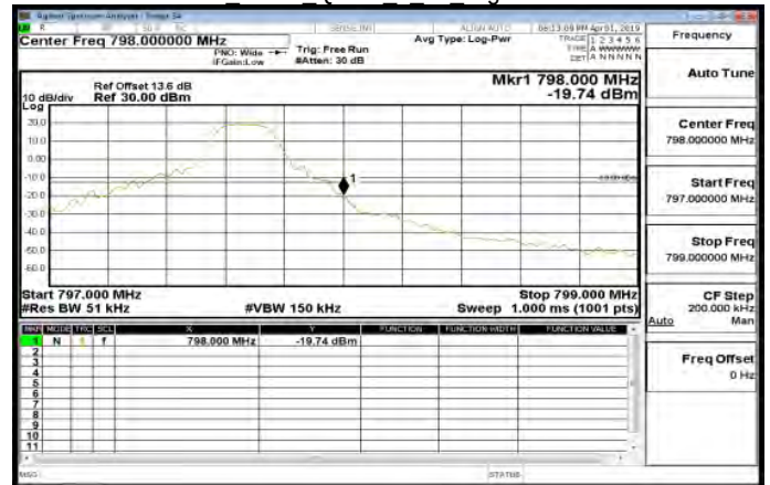
LTE\Band14 5MHz QPSK 25 0 LowCH23305-790.5
