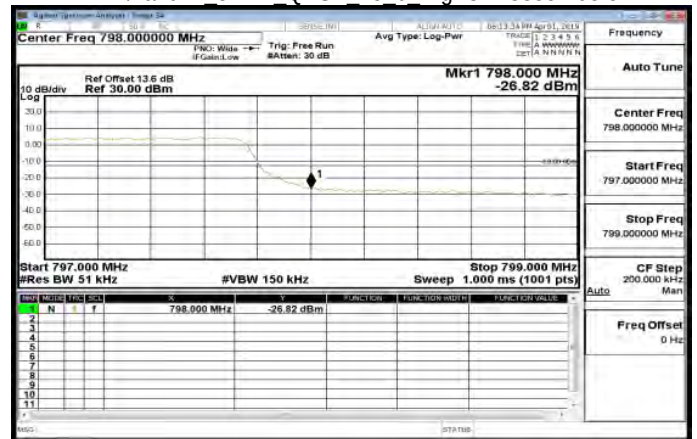
LTE\Band14 5MHz QPSK 25 0 HighCH23355-795.5
