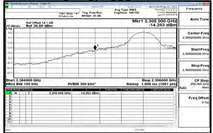
LTE\Band30 10MHz QPSK 1 0 LowCH27710-2310
