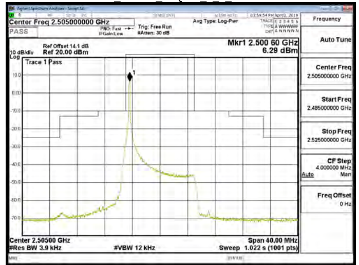
Band7 10MHz 64QAM 1 49 CH20800
