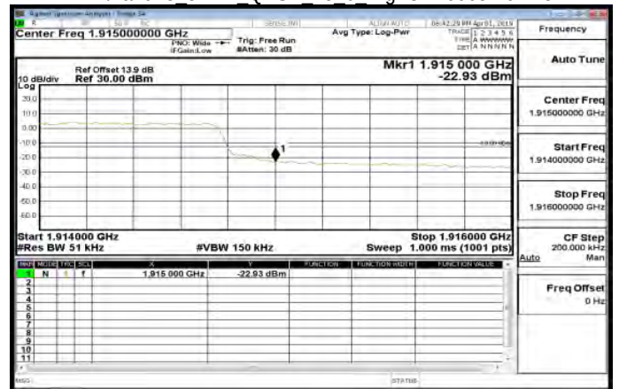
LTE\Band25 5MHz QPSK 25 0 HighCH26665-1912.5
