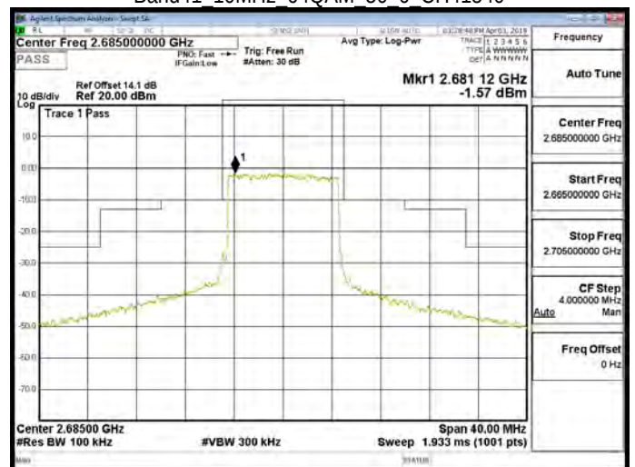
Band41 10MHz 64QAM 50 0 CH41540
