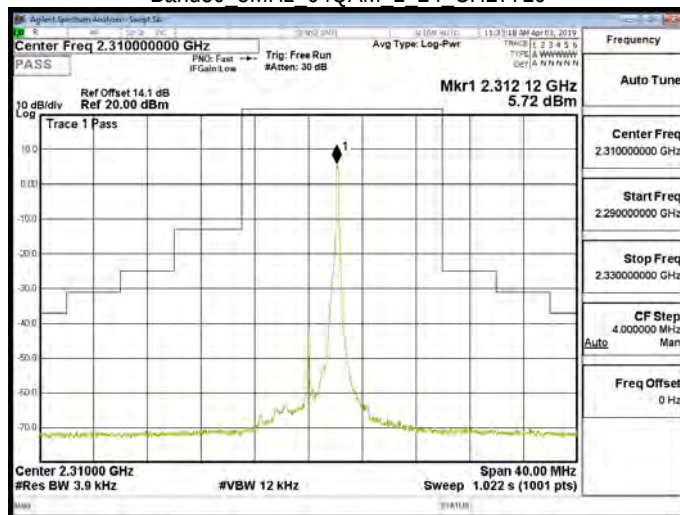
Band30 5MHz 64QAM 1 24 CH27735
