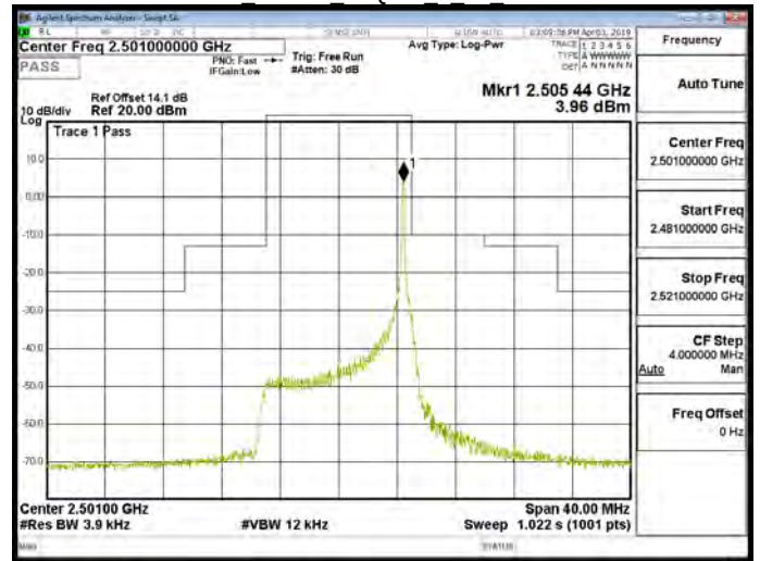
Band41 10MHz 16QAM 1 49 CH40620
