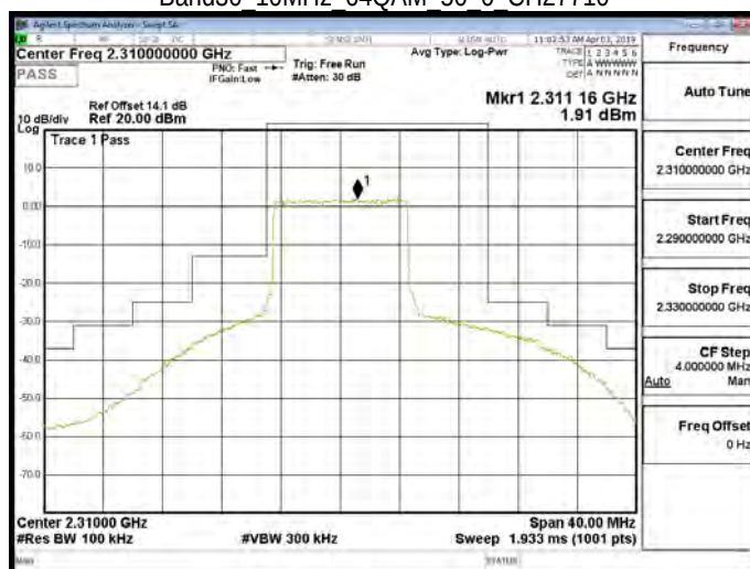
Band30 10MHz 64QAM 50 0 CH27710
