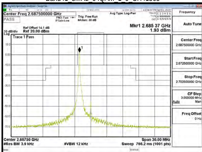
Band41 5MHz 64QAM 1 0 CH41565
