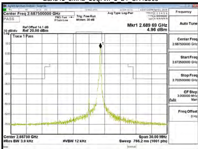
Band41 5MHz 16QAM 1 24 CH41565
