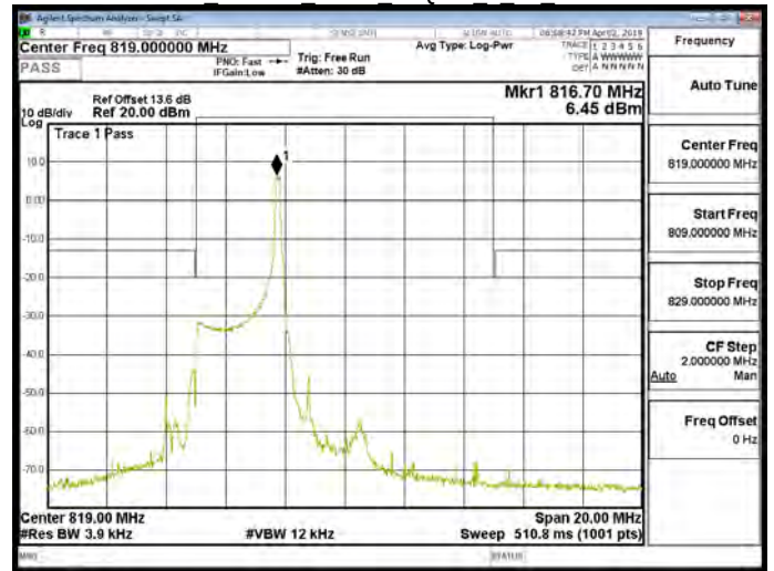
Band26 Part90s 3MHz 16QAM 1 14 CH26740
