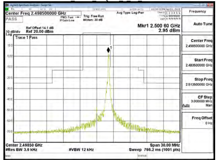
Band41 5MHz 64QAM 1 24 CH40620
