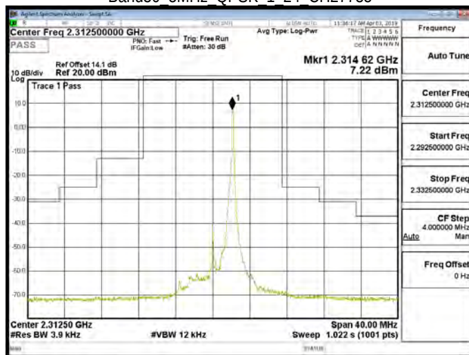
Band30 5MHz QPSK 1 24 CH27735
