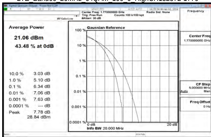
LTE Band66 20MHz 64QAM 100 0 HighCH132572-1770
