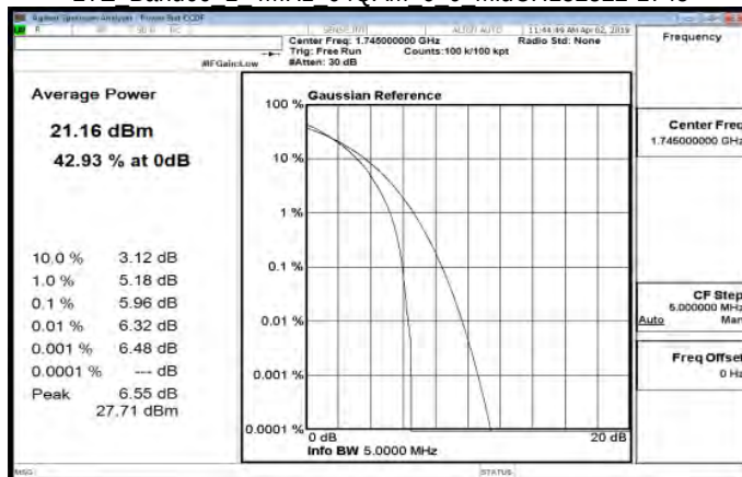
LTE Band66 1 4MHz 64QAM 6 0 MidCH132322-1745
