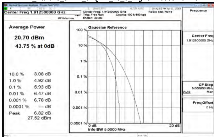
LTE Band25 5MHz 64QAM 25 0 HighCH26665-1912.5
