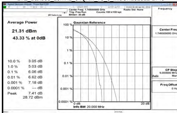
LTE Band66 15MHz 64QAM 75 0 MidCH132322-1745
