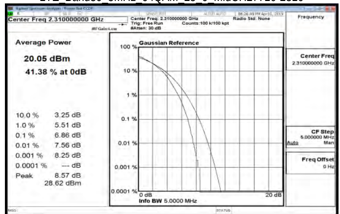
LTE Band30 5MHz 64QAM 25 0 MidCH27710-2310
