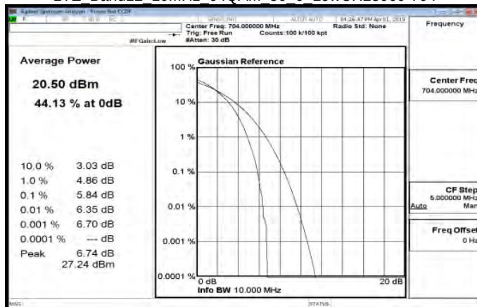
LTE Band12 10MHz 64QAM 50 0 LowCH23060-704
