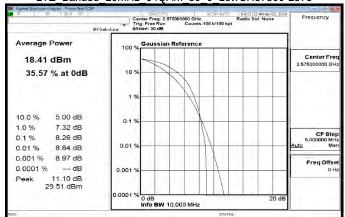
LTE Band38 10MHz 64QAM 50 0 LowCH37800-2575
