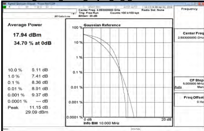
LTE Band41 10MHz 64QAM 50 0 MidCH40620-2593
