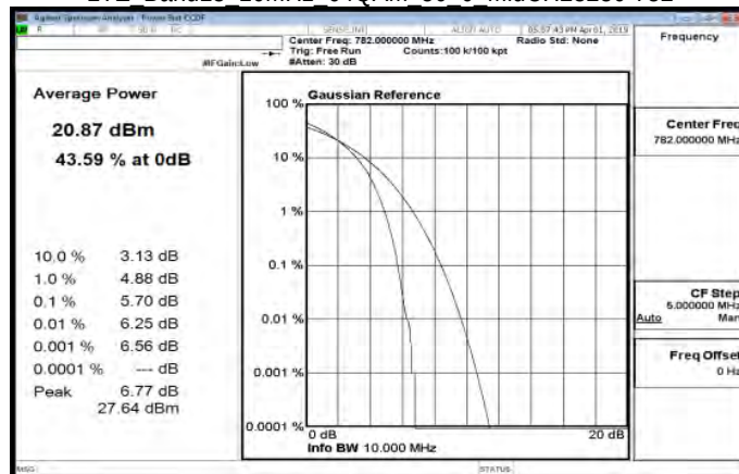
LTE Band13 10MHz 64QAM 50 0 MidCH23230-782
