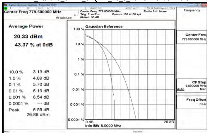
LTE Band13 5MHz 64QAM 25 0 LowCH23205-779.5
