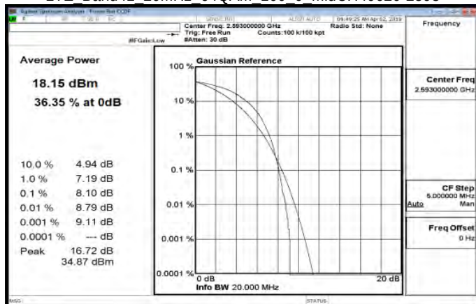
LTE Band41 20MHz 64QAM 100 0 MidCH40620-2593
