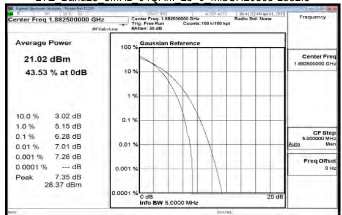
LTE Band25 5MHz 64QAM 25 0 MidCH26365-1882.5
