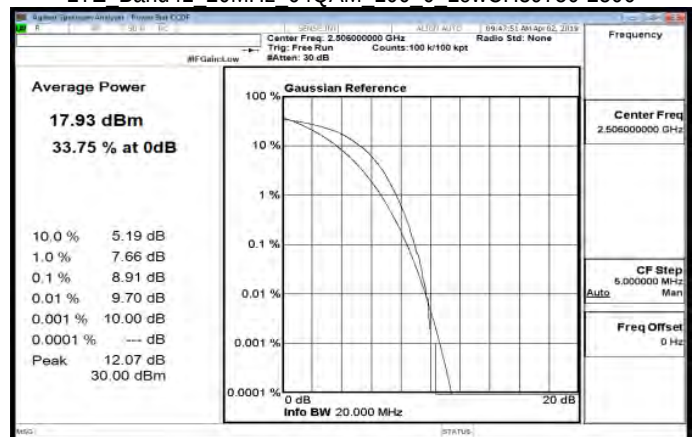
LTE Band41 20MHz 64QAM 100 0 LowCH39750-2506
