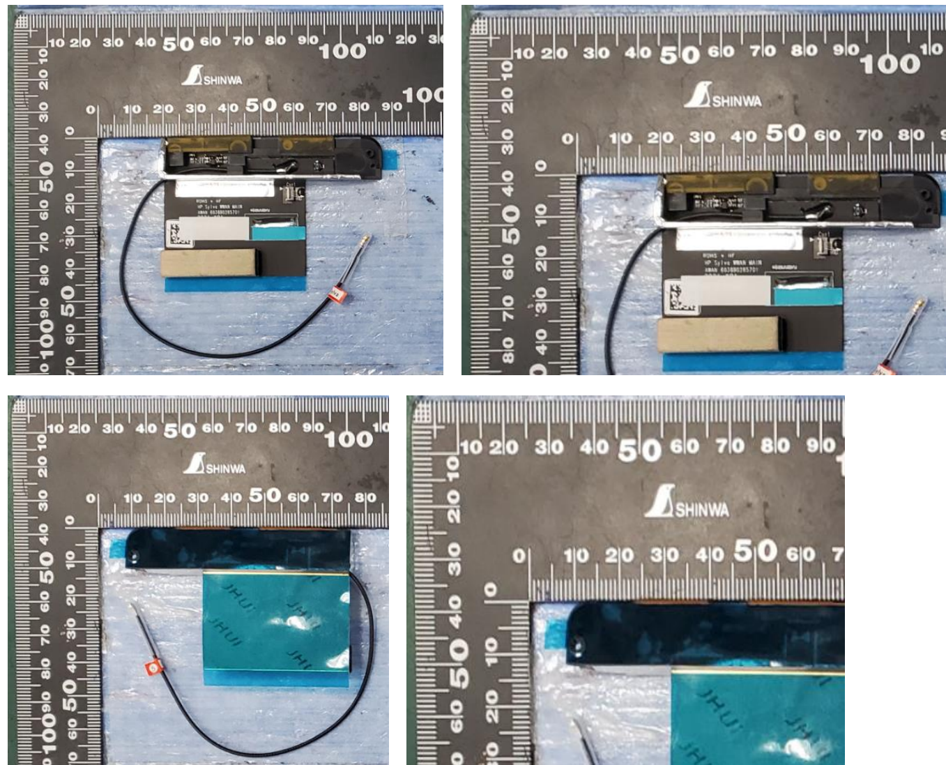
Tx1/Rx1 Antenna Photo:
