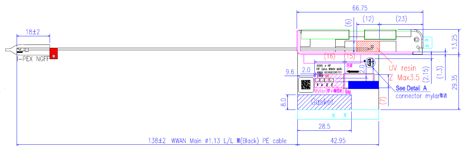
Tx1/Rx1 Antenna Photo:
